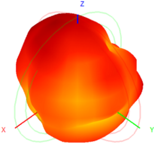
2400.0MHz Total, Eff: 36.1%
