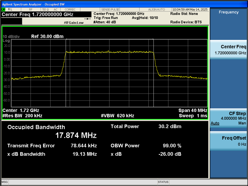
Test_Graph_band4_1720MHz_20M_16QAM_100RB#LOW_OBW&EBW
