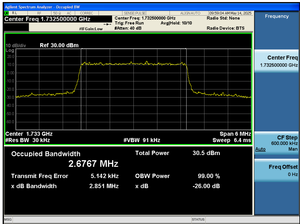
Test_Graph_band4_1732.5MHz_3M_QPSK_15RB#LOW_OBW&EBW
