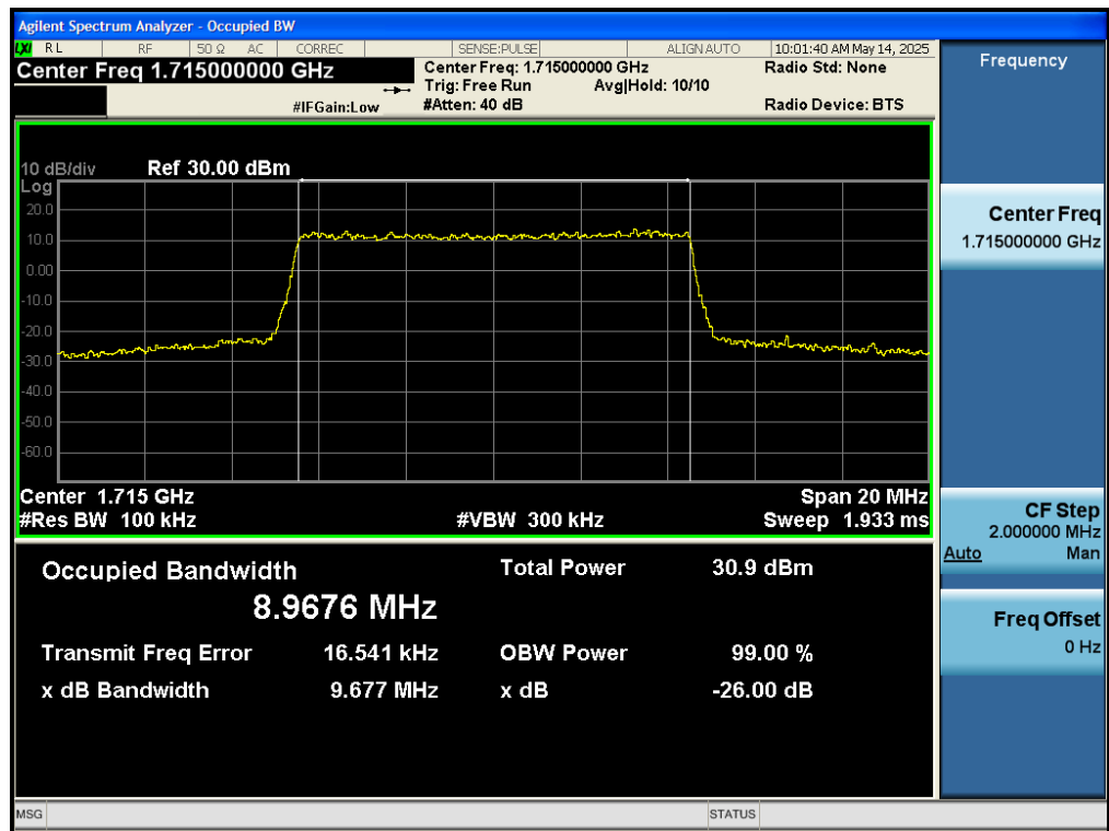
Test_Graph_band4_1715MHz_10M_QPSK_50RB#LOW_OBW&EBW
