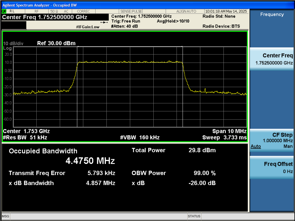
Test_Graph_band4_1752.5MHz_5M_16QAM_25RB#LOW_OBW&EBW
