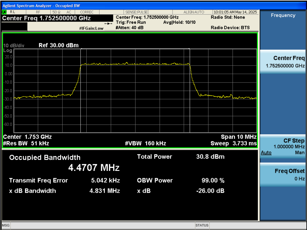
Test_Graph_band4_1752.5MHz_5M_QPSK_25RB#LOW_OBW&EBW
