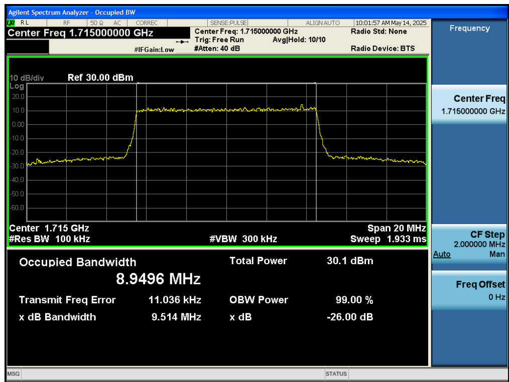
Test_Graph_band4_1715MHz_10M_16QAM_50RB#LOW_OBW&EBW
