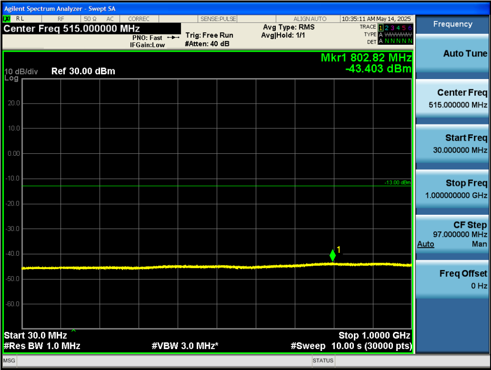
Test_Graph_band4_1747.5MHz_15M_QPSK_75RB#LOW_30M_1G_TX
