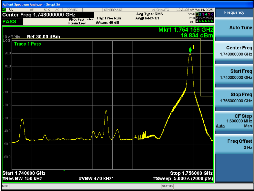
Test_Graph_band4_1747.5MHz_15M_16QAM_1RB#HIGH_Band edge
