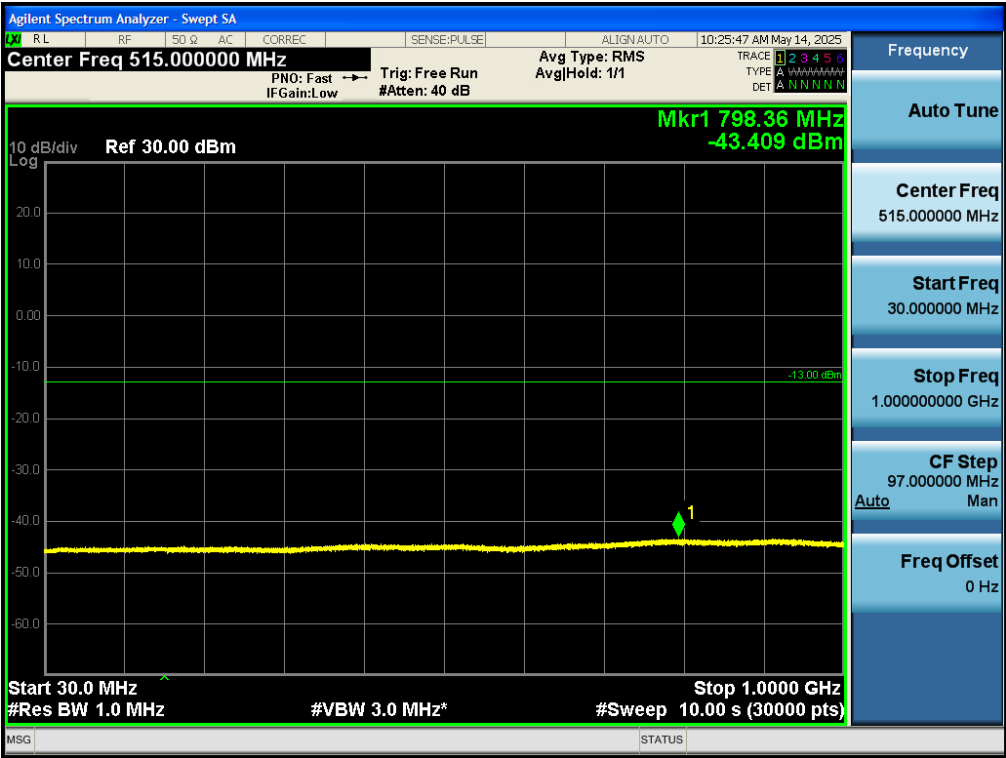
Test_Graph_band4_1732.5MHz_1.4M_QPSK_6RB#LOW_30M_1G_TX
