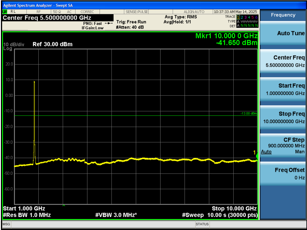
Test_Graph_band4_1745MHz_20M_QPSK_100RB#LOW_1G_10G_TX
