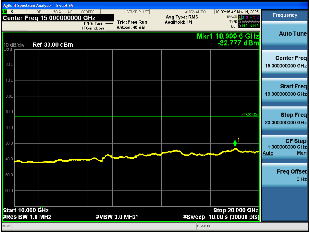
Test_Graph_band4_1732.5MHz_10M_QPSK_50RB#LOW_10G_20.0G_TX
