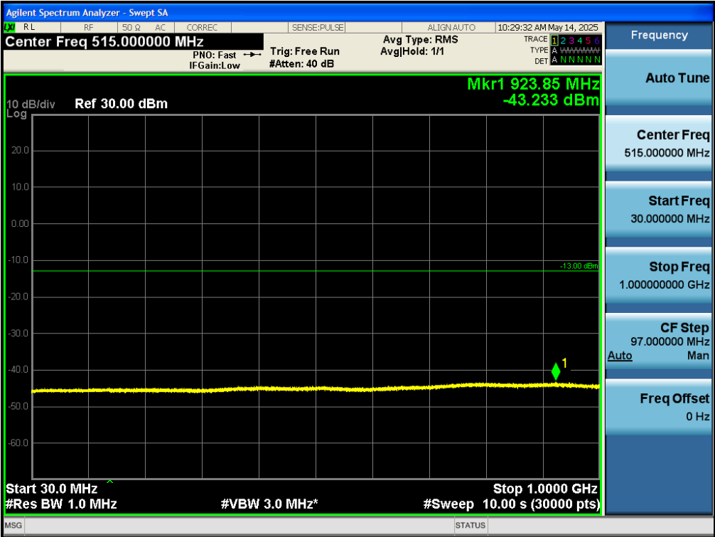
Test_Graph_band4_1712.5MHz_5M_QPSK_25RB#LOW_30M_1G_TX
