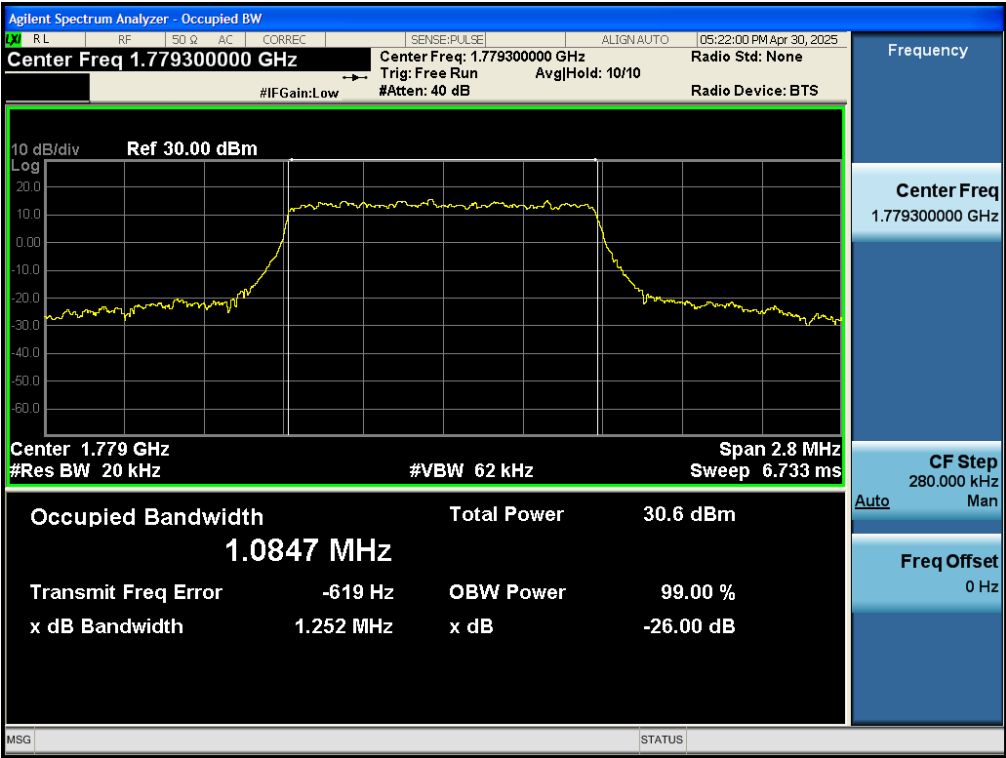
Test_Graph_band66_1779.3MHz_1.4M_QPSK_6RB#LOW_OBW&EBW
