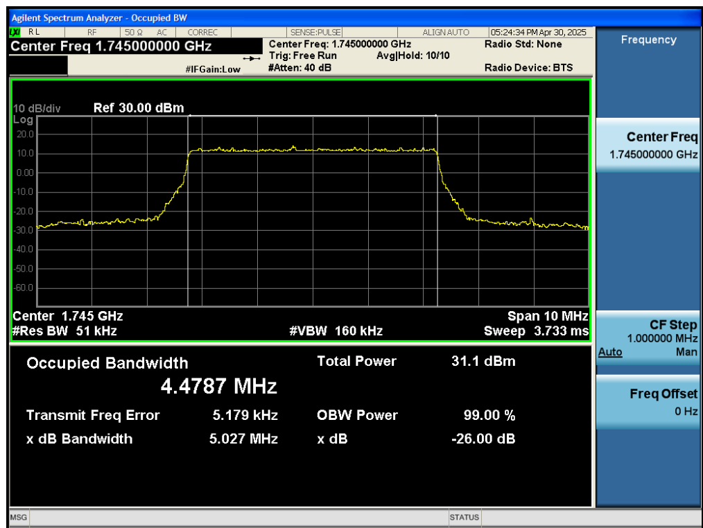
Test_Graph_band66_1745MHz_5M_QPSK_25RB#LOW_OBW&EBW
