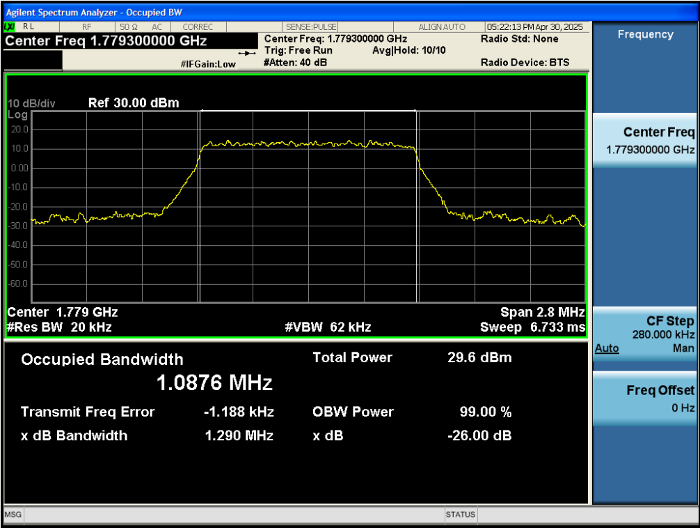
Test_Graph_band66_1779.3MHz_1.4M_16QAM_6RB#LOW_OBW&EBW
