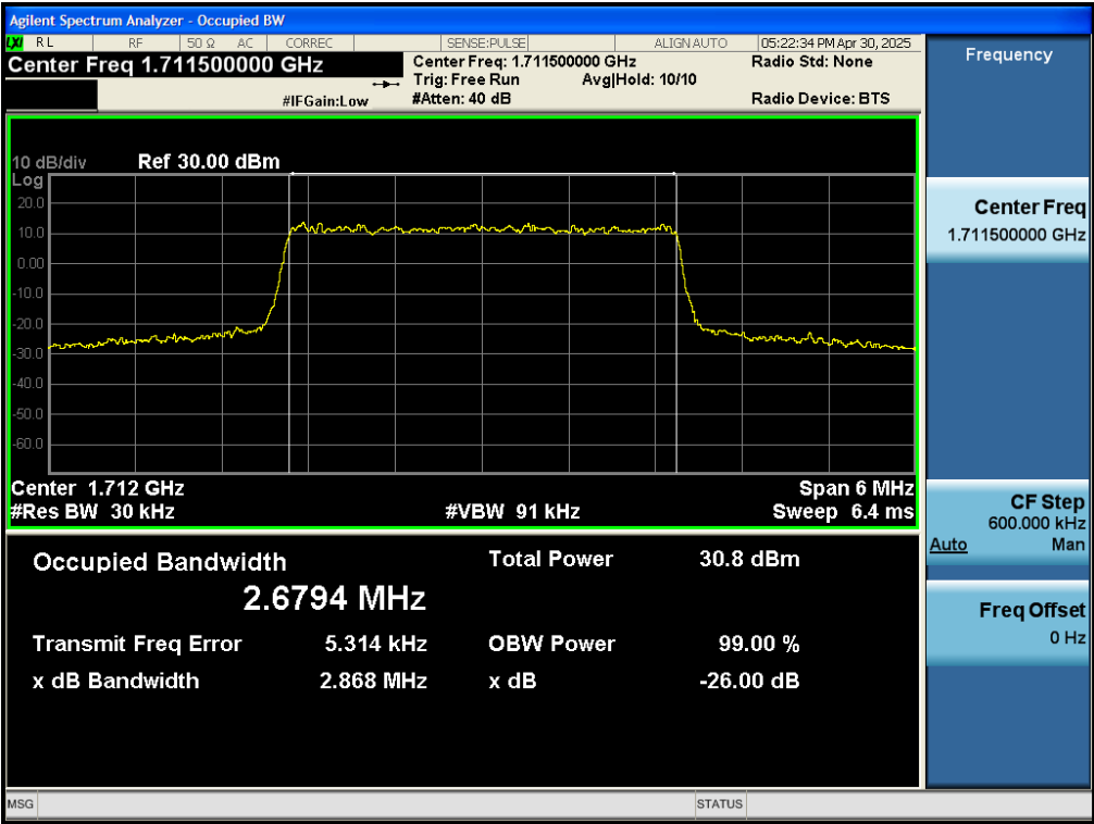
Test_Graph_band66_1711.5MHz_3M_QPSK_15RB#LOW_OBW&EBW
