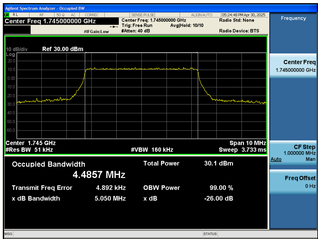
Test_Graph_band66_1745MHz_5M_16QAM_25RB#LOW_OBW&EBW
