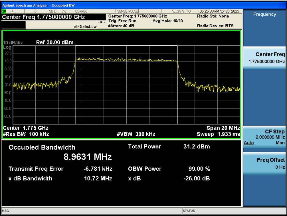
Test_Graph_band66_1775MHz_10M_QPSK_50RB#LOW_OBW&EBW
