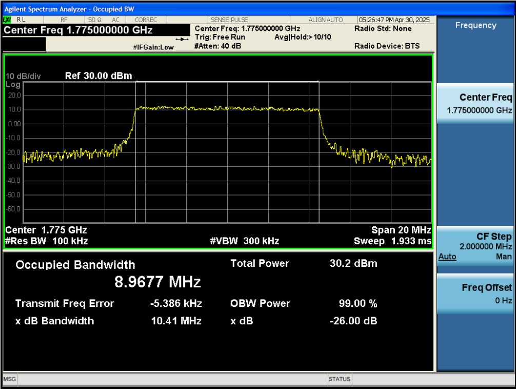
Test_Graph_band66_1775MHz_10M_16QAM_50RB#LOW_OBW&EBW
