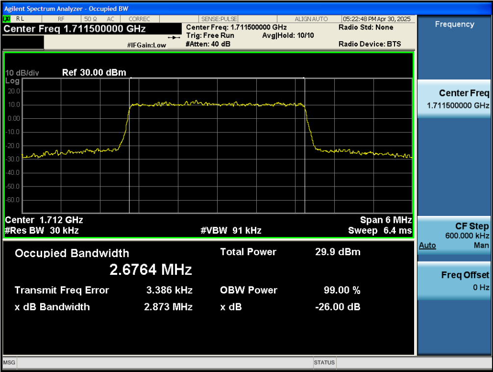
Test_Graph_band66_1711.5MHz_3M_16QAM_15RB#LOW_OBW&EBW
