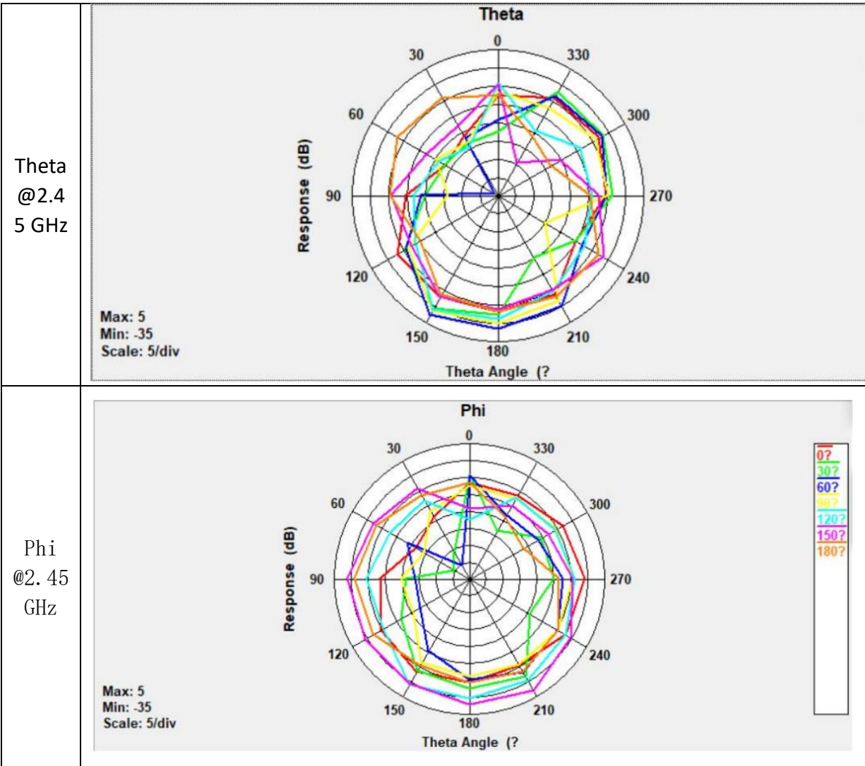
Antenna Pattern/Gain Measurement data/Table:
