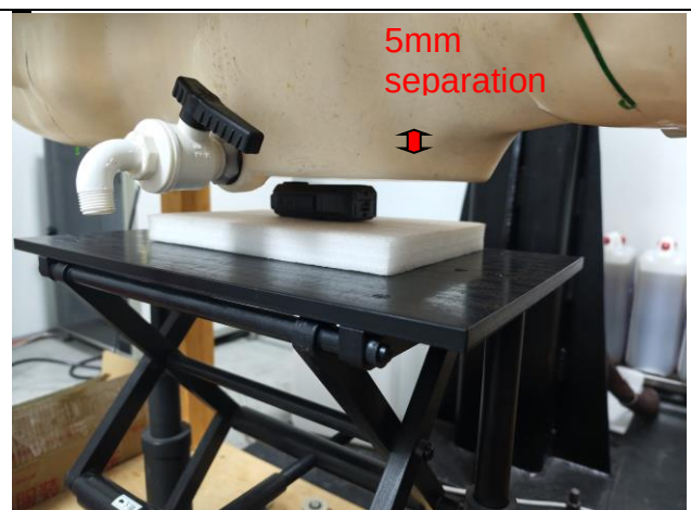
Body (Wrist-worn)
