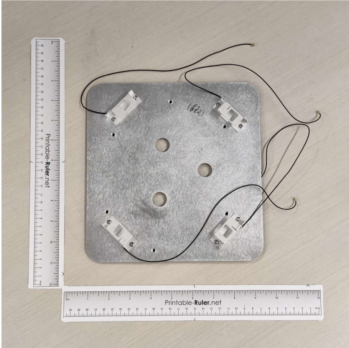
Antenna Pad Top View
