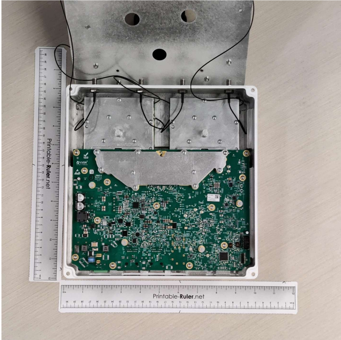
Antenna Pad Removed
