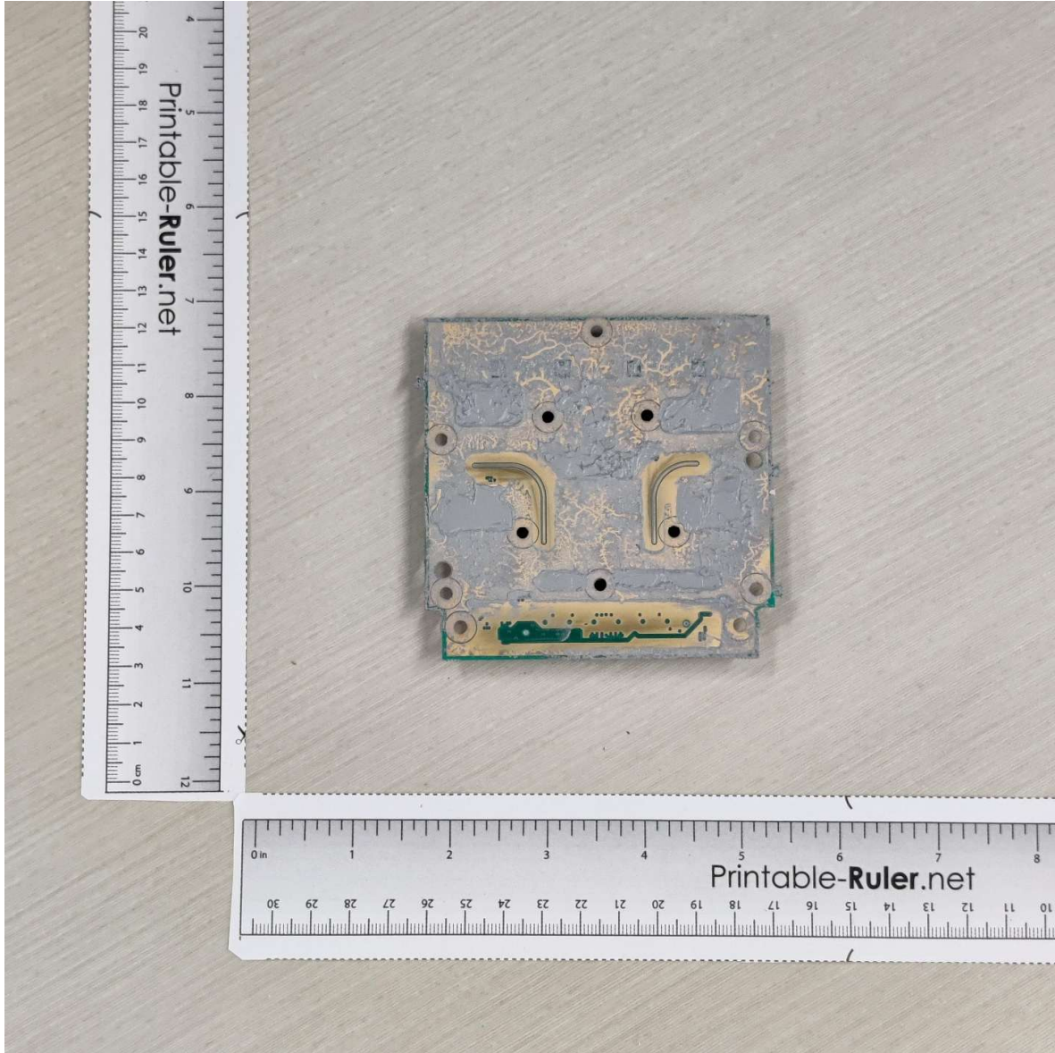
Left RF Card Bottom View
