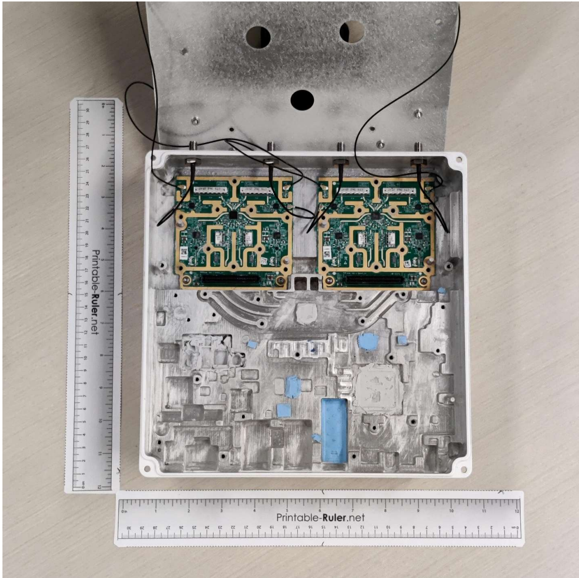
Main Board Removed
