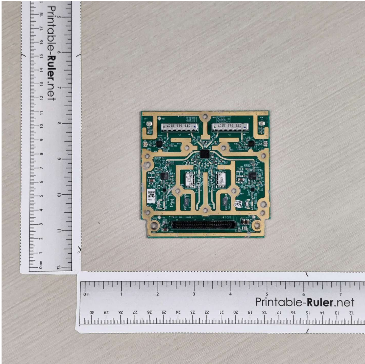
Right RF Card Top View
