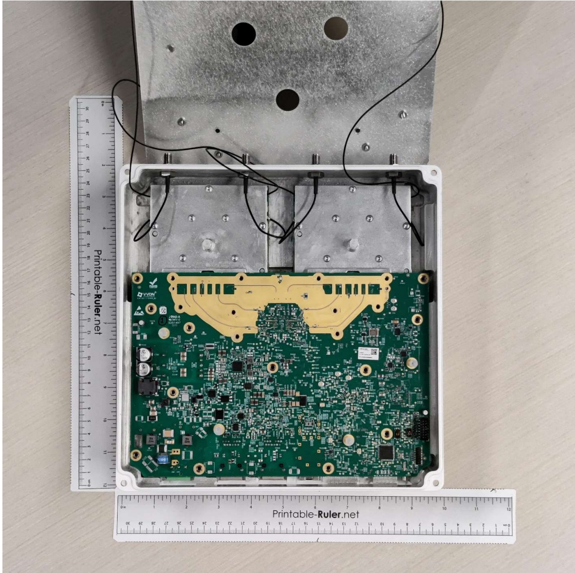
Main Board Heatsink Removed
