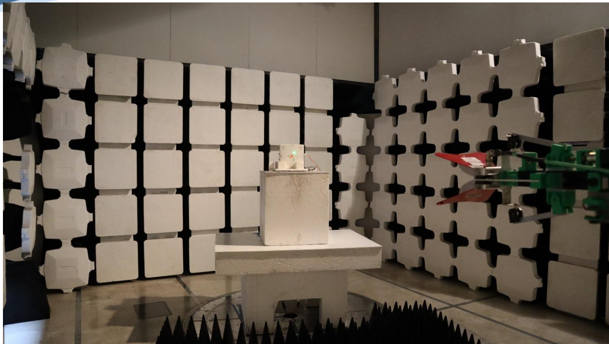
Integral Spurious Emissions 1GHz to 18GHz
