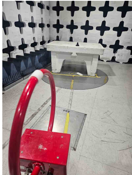
Radiated emissions test set up below 30MHz.
