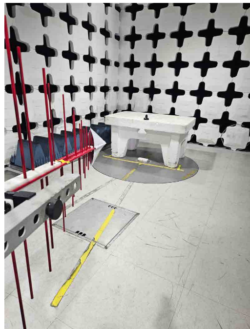
Radiated emissions test set up in 30MHz-1GHz frequency range
