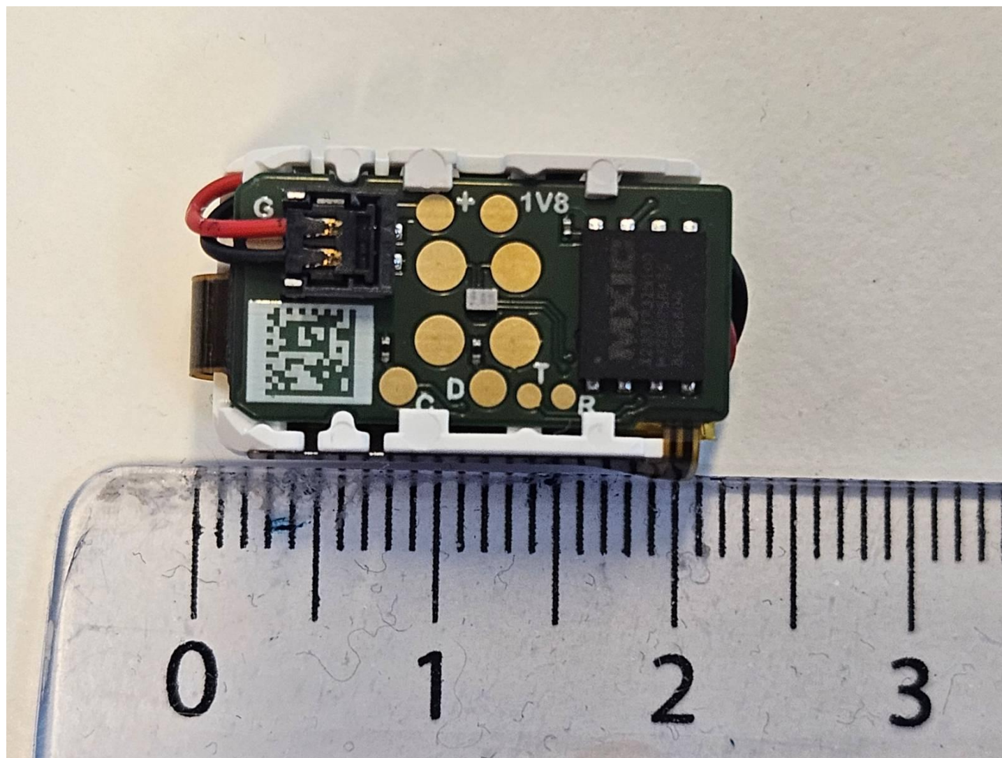
Frame assembly top
