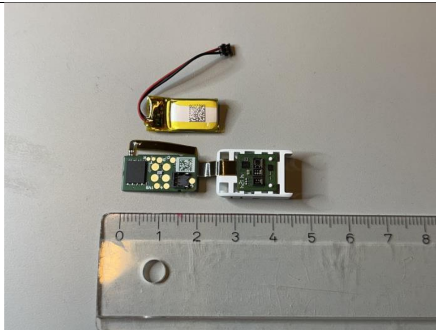
Picture 6, EUT PCB + battery
