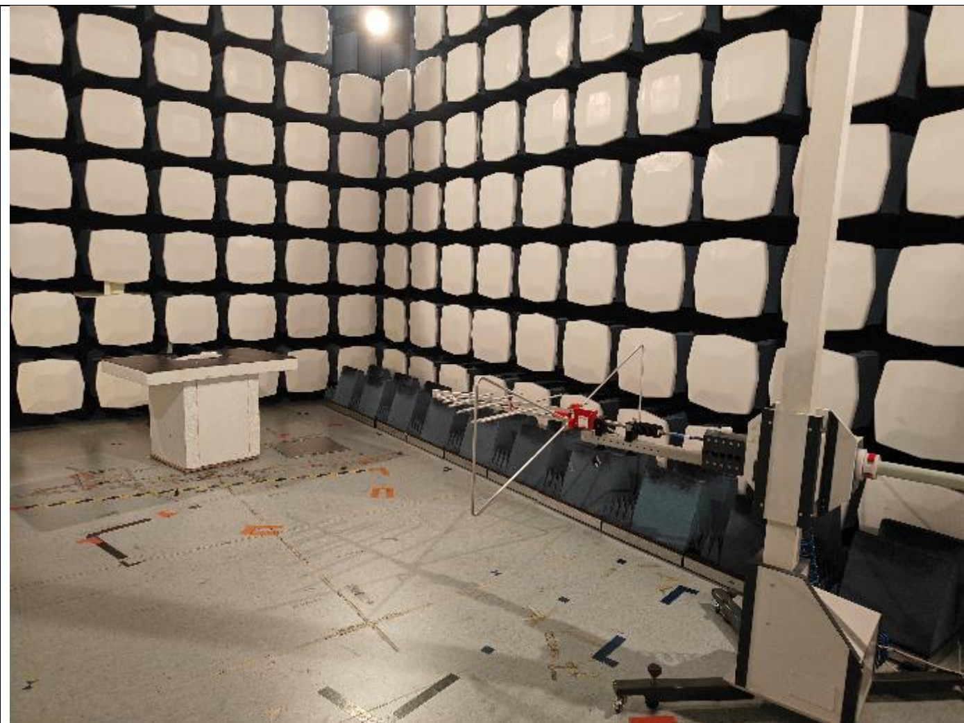
Picture 8, Radiated Spurious Emissions, common setup, TX and RX 30 - 1000 MHz
