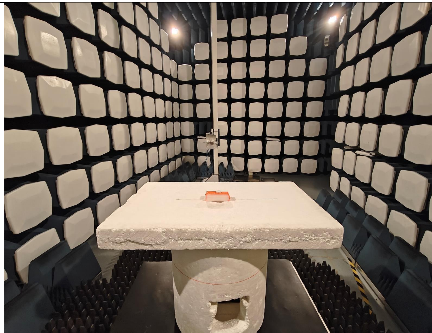
Picture 14, Radiated Spurious Emissions, EUT setup back view, TX 1 – 26 GHz
