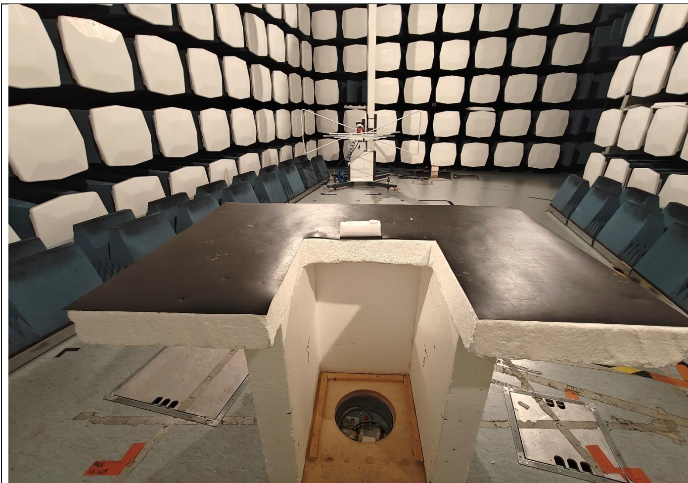
Picture 13, Radiated Spurious Emissions, EUT setup back view, TX and RX 30 – 1000 MHz
