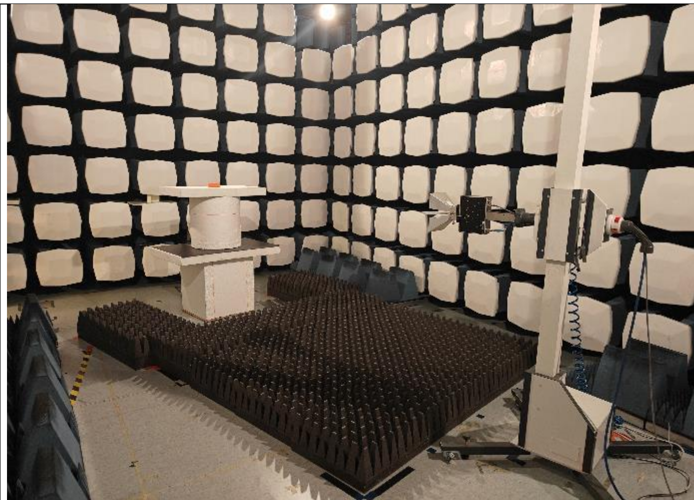
Picture 9, Radiated Spurious Emissions, common setup, TX, 1 – 26 GHz
