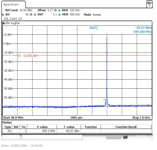
Band12_3MHz_16QAM_23095_1RB#0_30~1000_30~1000
