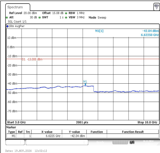
Band12_3MHz_QPSK_23095_1RB#0_3000~10000_3000~10000
