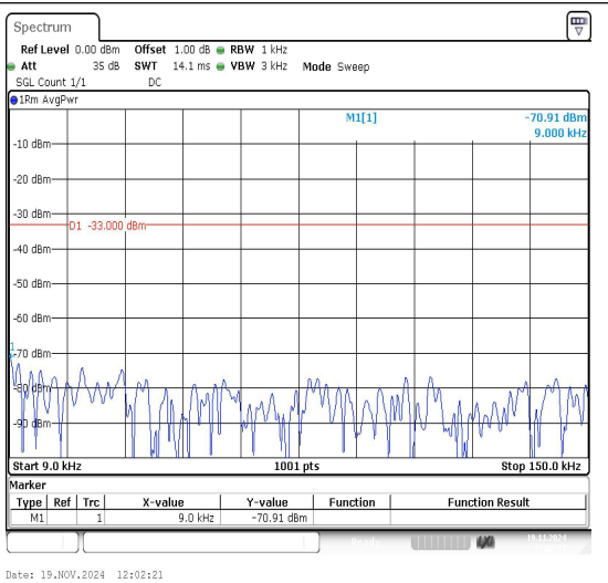
Band12_3MHz_16QAM_23095_1RB#0_0.009~0.15_0.009~0.15
