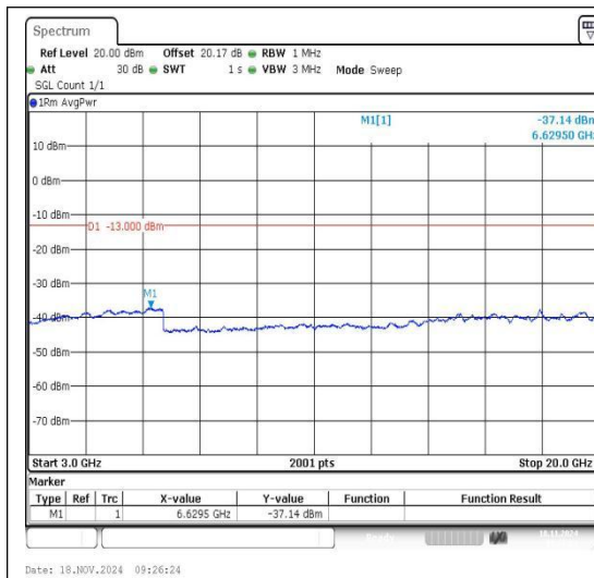
Band2_5MHz_QPSK_19175_1RB#0_3000~2000 0_3000~20000
