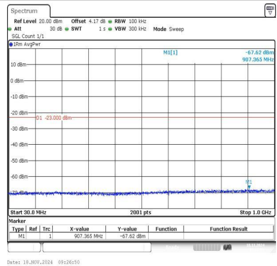
Band2_5MHz_16QAM_19175_1RB#0_30~1000_3 0~1000
