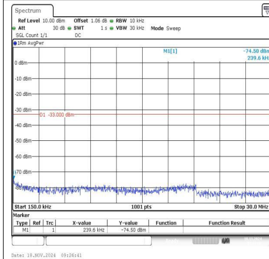
Band2_5MHz_16QAM_19175_1RB#0_0.15~30 0.15~30
