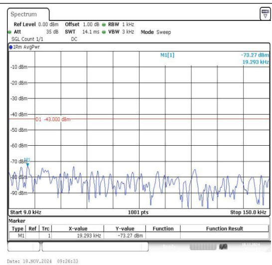
Band2_5MHz_16QAM_19175_1RB#0_0.009~0.15 _0.009~0.15
