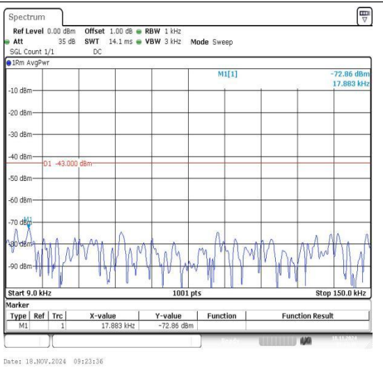
Band2_5MHz_16QAM_18625_1RB#0_0.009~0.15 _0.009~0.15
