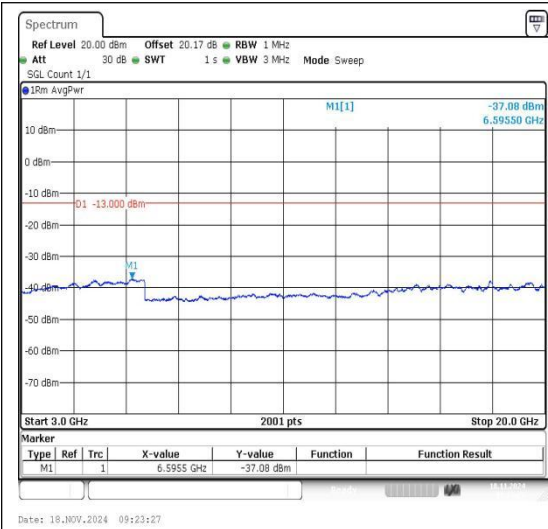
Band2_5MHz_QPSK_18625_1RB#0_3000~2000 0_3000~20000
