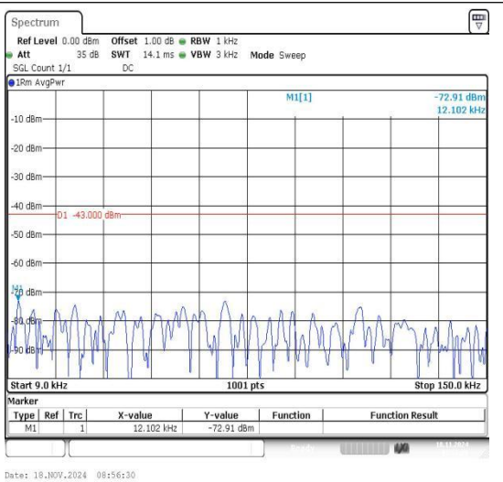
Band2_3MHz_16QAM_19185_1RB#0_0.009~0.15 _0.009~0.15
