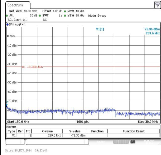
Band2_5MHz_16QAM_18625_1RB#0_0.15~30 0.15~30
