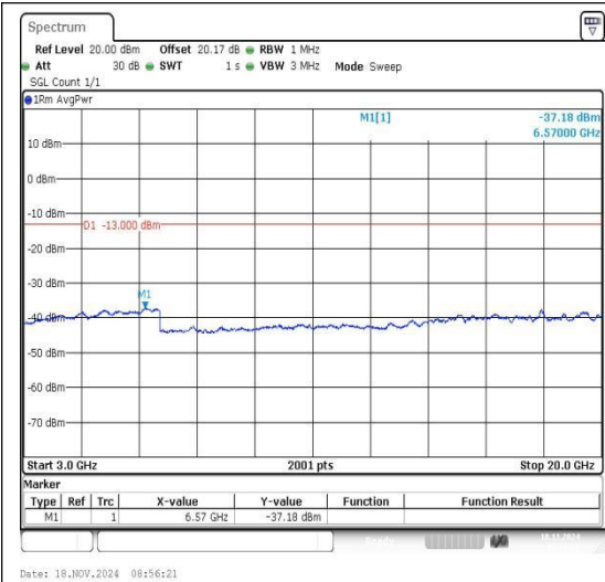
Band2_3MHz_QPSK_19185_1RB#0_3000~2000 0_3000~20000
