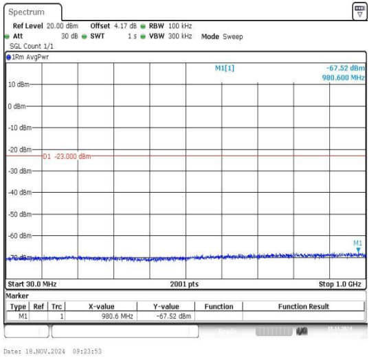
Band2_5MHz_16QAM_18625_1RB#0_30~1000_3 0~1000
