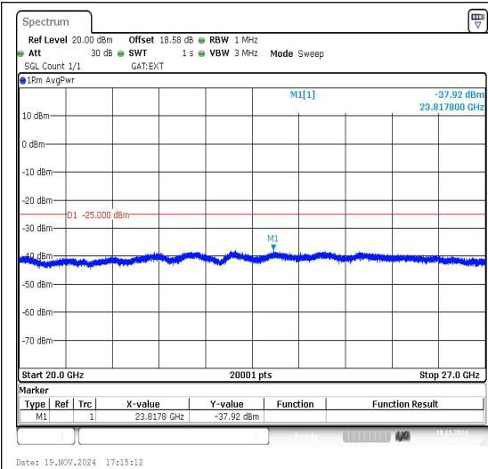
Band41_10MHz_QPSK_41540_1RB#0_20000~27000
