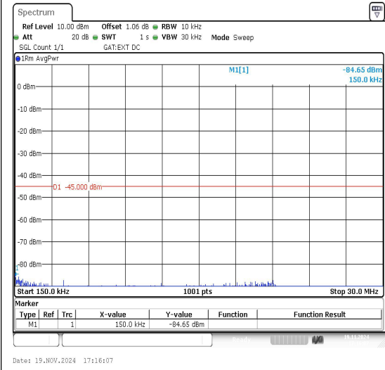
Band41_10MHz_16QAM_41540_1RB#0_0.15~30_0.15~30
