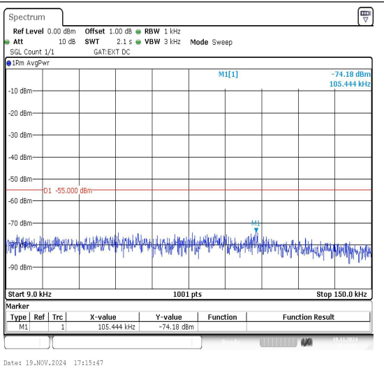
Band41_10MHz_16QAM_41540_1RB#0_0.009~0.15_0.009~0.15
