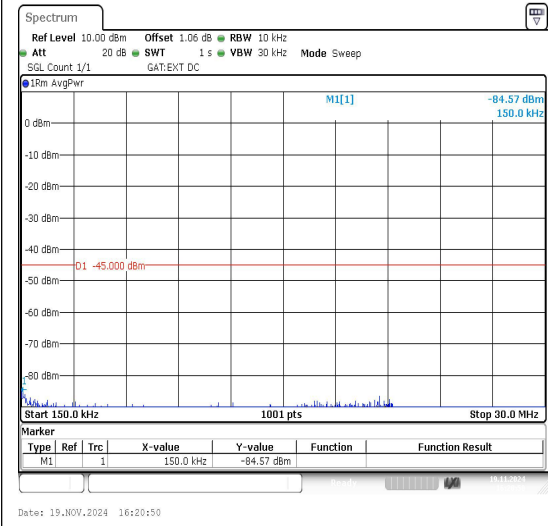
Band41_5MHz_16QAM_40620_1RB#0_0.15~30 _0.15~30
