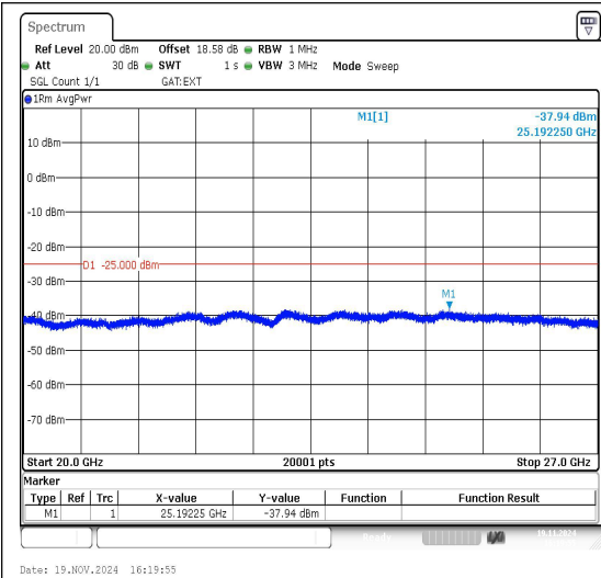
Band41_5MHz_QPSK_40620_1RB#0_20000~27000 000_20000~27000
