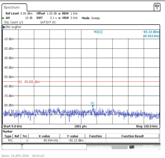
Band41_5MHz_16QAM_40620_1RB#0_0.009~0.1 5_0.009~0.15
