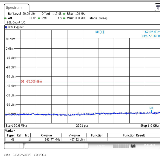
Band7_15MHz_QPSK_20825_1RB#0_30~1000_30~1000
