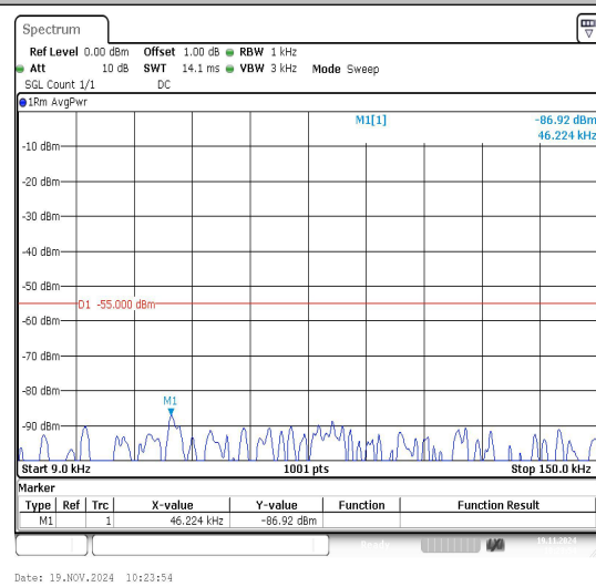
Band7_15MHz_QPSK_20825_1RB#0_0.009~0.15_0.009~0.15
