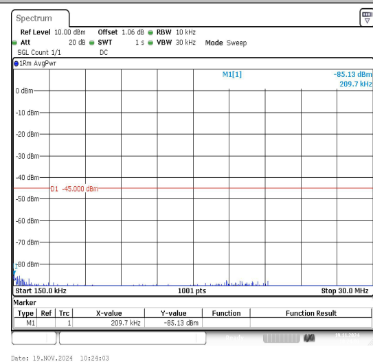
Band7_15MHz_QPSK_20825_1RB#0_0.15~30_0.15~30
