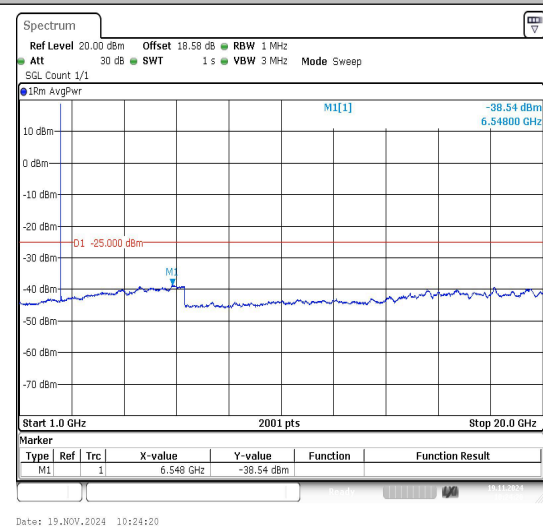
Band7_15MHz_QPSK_20825_1RB#0_1000~20000_1000~20000
