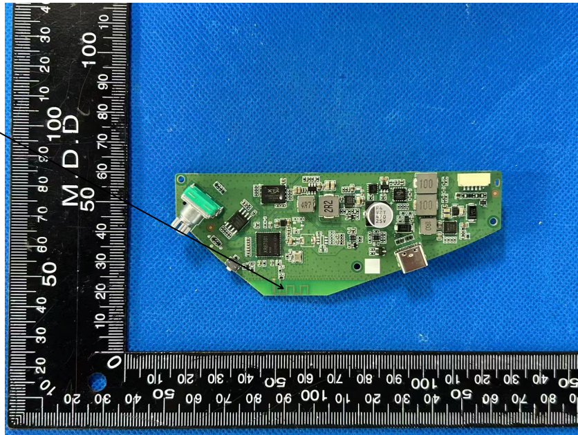
PCB Antenna
