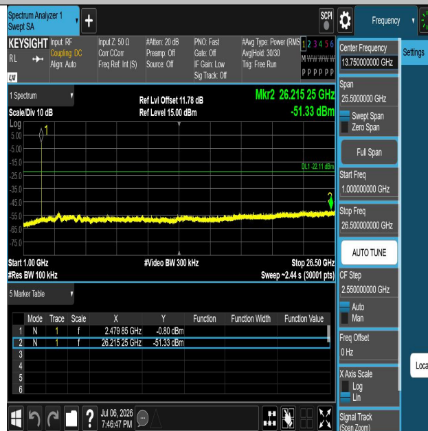
BLE_2M-Ant1-2480-1000~26500-PASS
