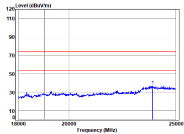
remote 2.4G_SRD_TX_CH_M_Vertical
