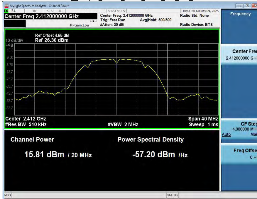
MAX_Output_Power_NVNT_ANT1_802_11b_2412
