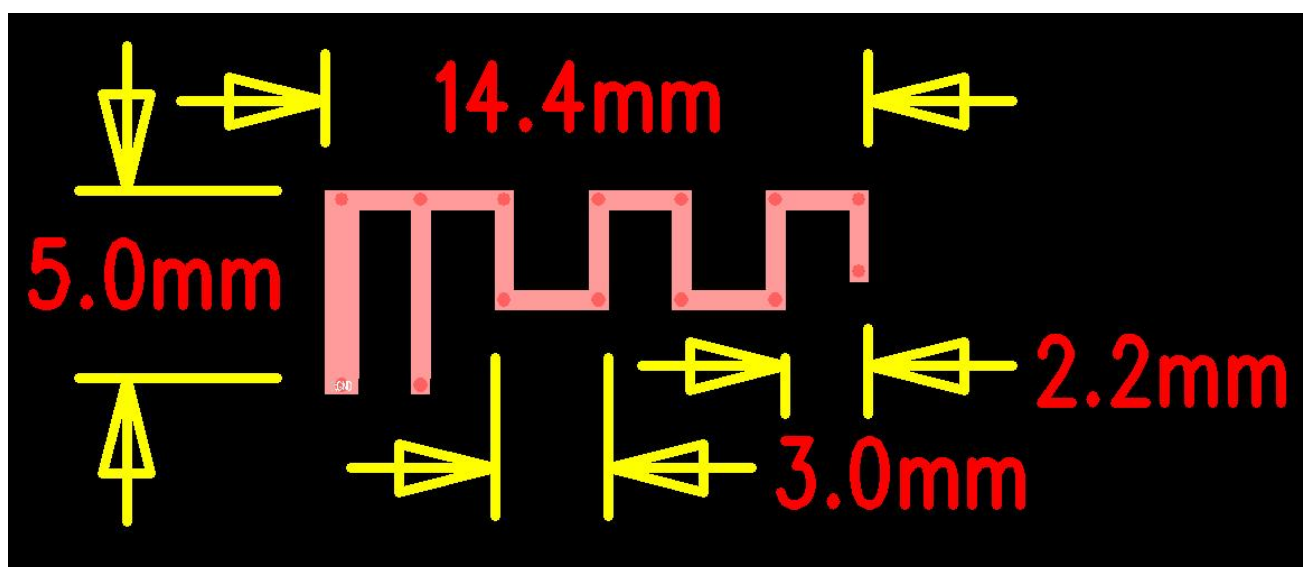
Picture of antenna
