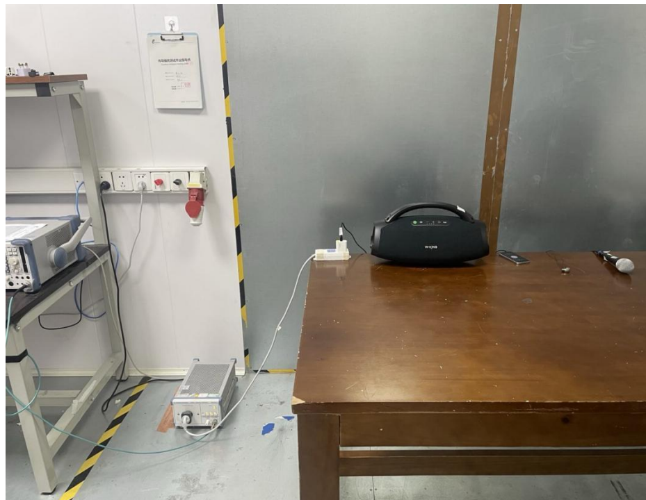
Conducted emissions at AC power line (150kHz-30MHz)
