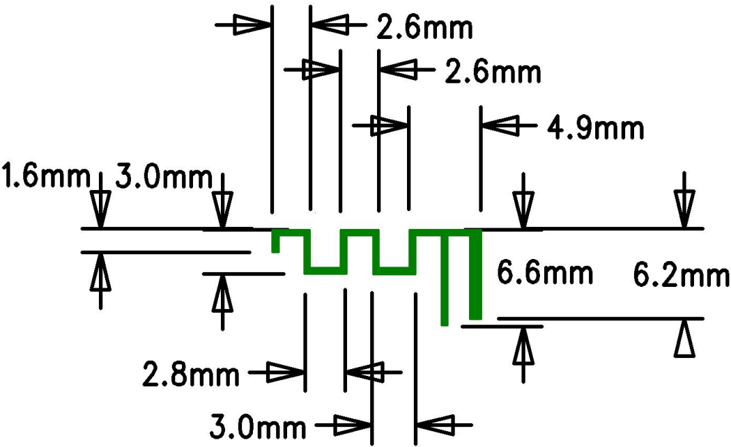
Picture of antenna
