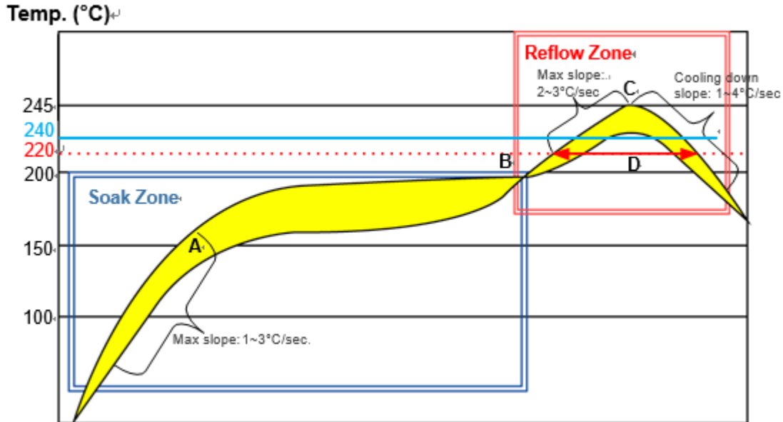
Figure 45 Recommended Reflow Temperature Profile
