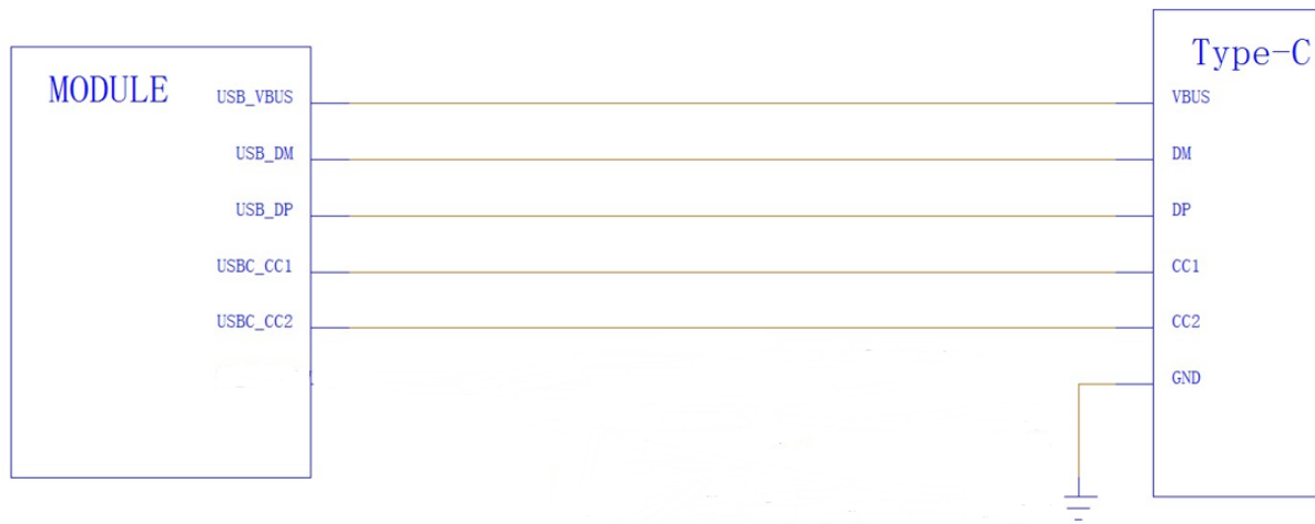
Figure 10 USB Type-C Reference Design
