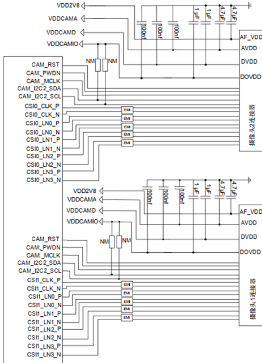
Figure 17 2-Way Camera Reference Design
