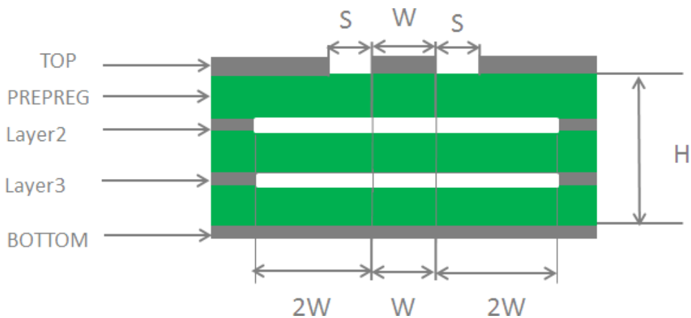
Figure 33 Four-layer PCB Coplanar Waveguide Structure (Reference Ground Is The Fourth Layer)
