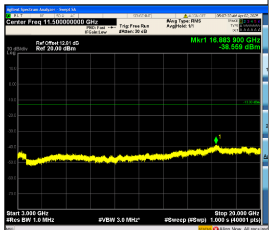
Band4_1.4MHz_QPSK_20175_6RB#0_3000~20 000_3000~20000
