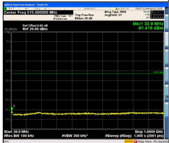
Band4_1.4MHz_QPSK_20175_6RB#0_30~1000 _30~1000
