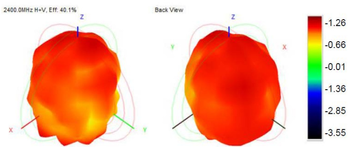
Gain test chart (unit: dBi)
