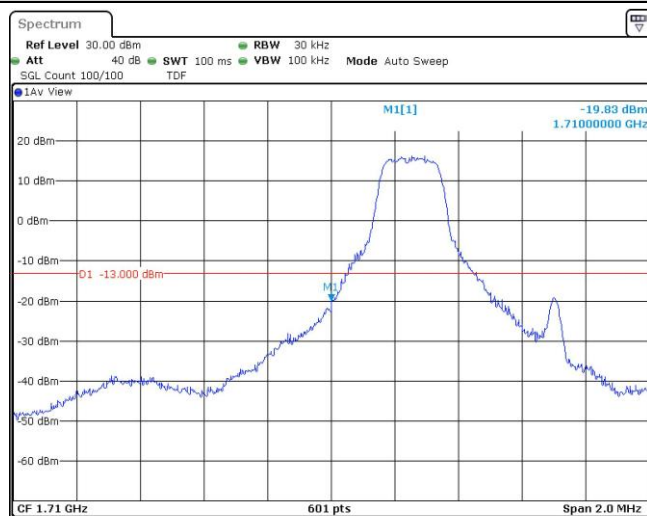
Band4-1.4MHz-QPSK-19957-1RB#5
