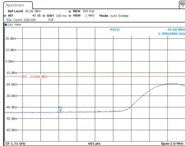
Band4-15MHz-QPSK-20025-75RB#0
