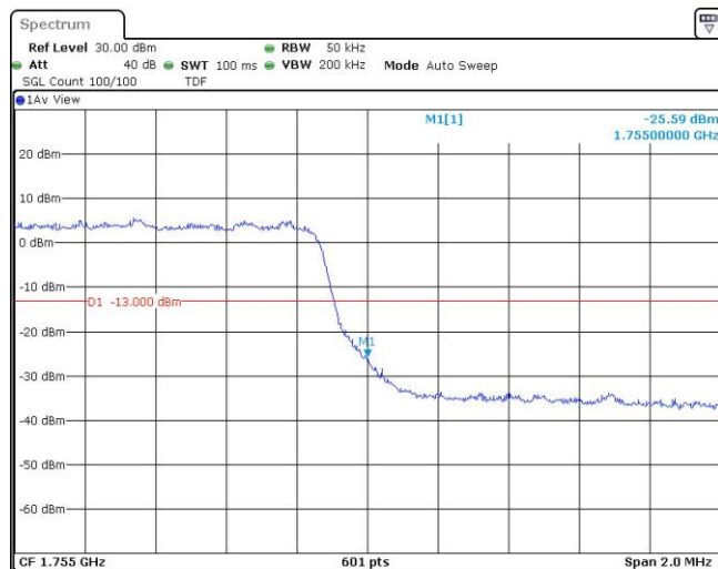
Band4-3MHz-16QAM-19965-1RB#0
