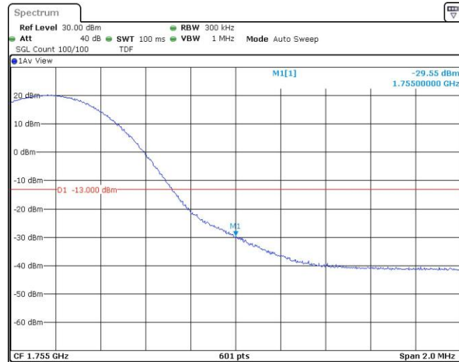
Band4-15MHz-QPSK-20325-75RB#0
