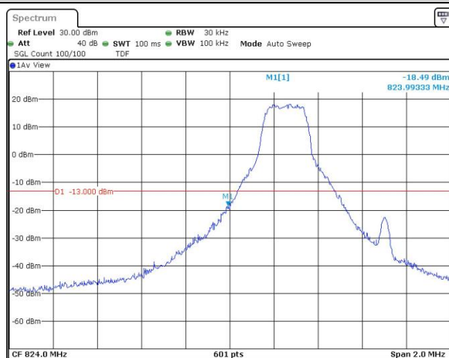
Band5-1.4MHz-QPSK-20407-1RB#5
