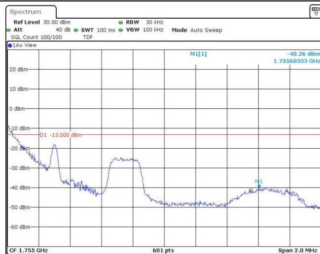
Band4-1.4MHz-16QAM-20393-1RB#5
