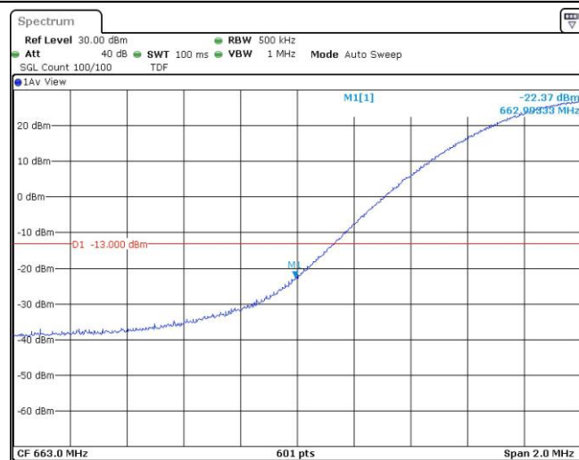
Band71-20MHz-16QAM-133222-1RB#99
