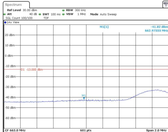
Band71-15MHz-QPSK-133197-75RB#0
