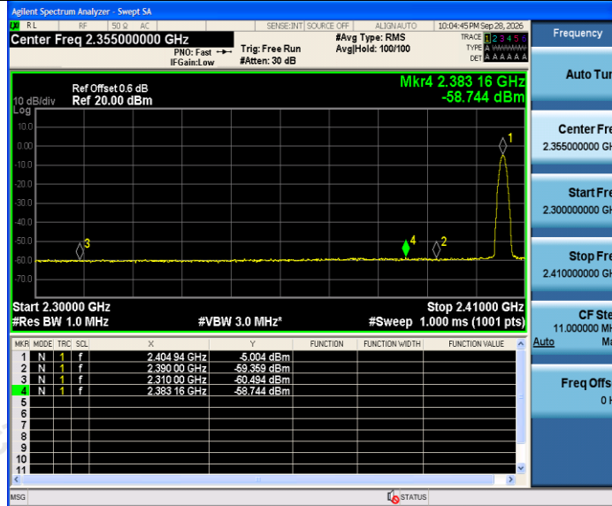
2.4G Ant1 Low 2405 Peak
