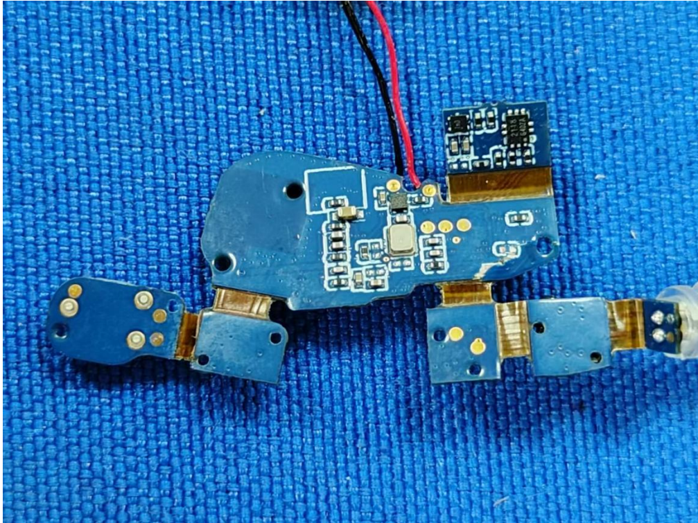
Figure 10. PCB view of Hearing Aids (R)
