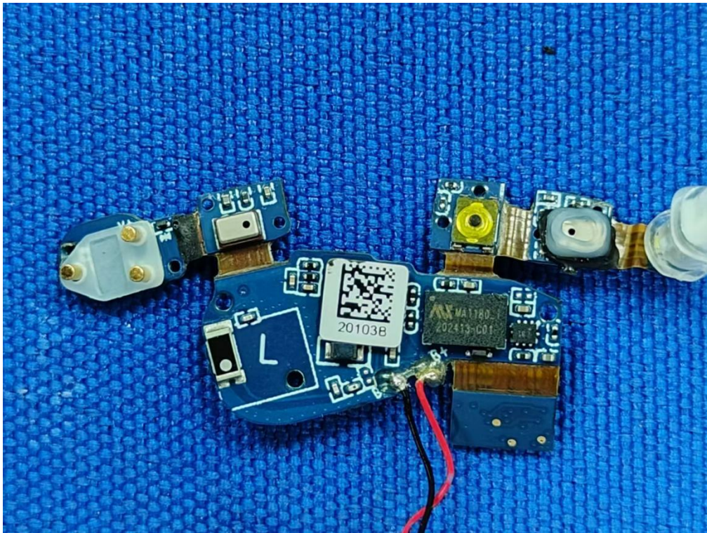
Figure 7. PCB view of Hearing Aids (L)
