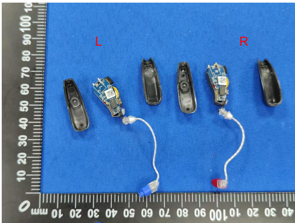
Figure 2. Internal view of Hearing Aids
