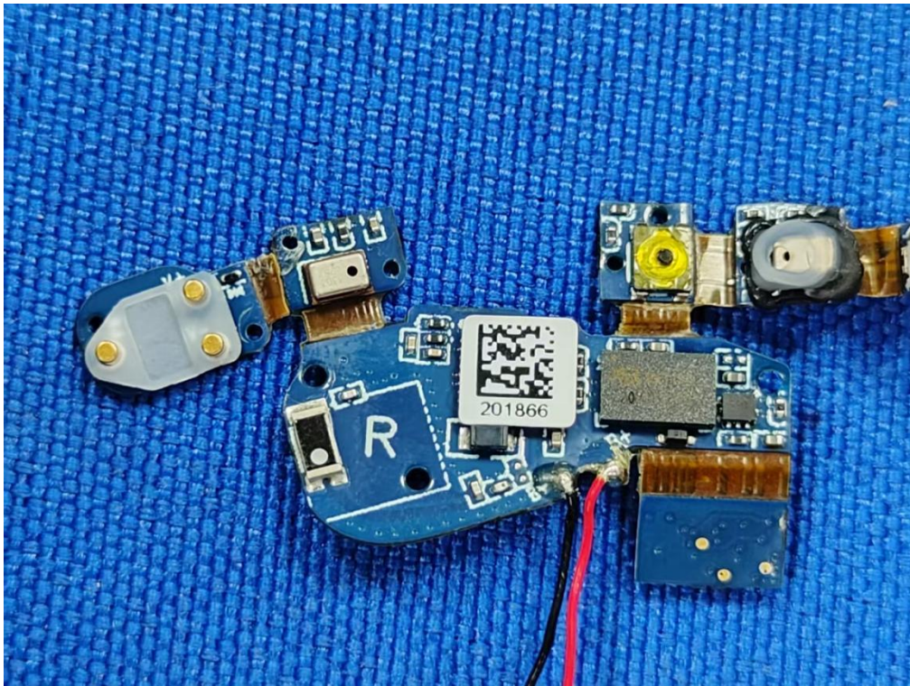
Figure 9. PCB view of Hearing Aids (R)
