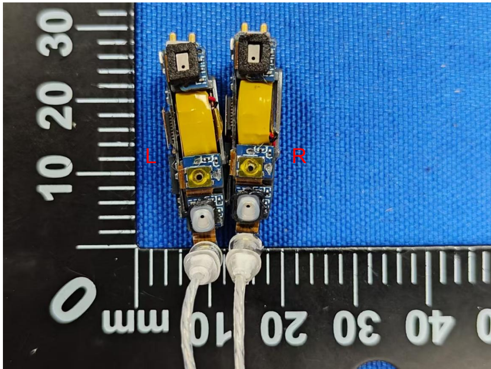
Figure 3. Internal view of Hearing Aids
