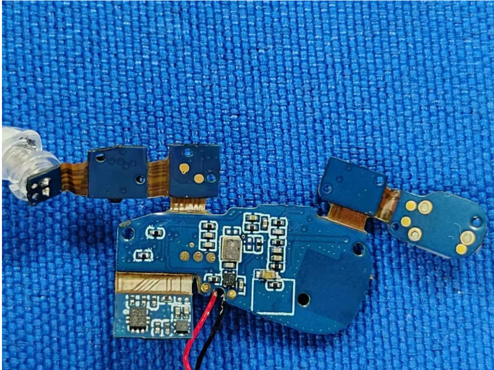
Figure 8. PCB view of Hearing Aids (L)
