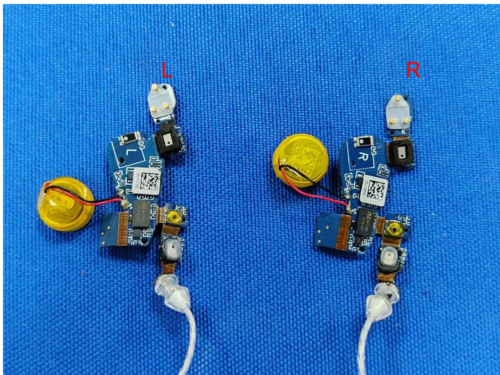
Figure 4. Internal view of Hearing Aids
