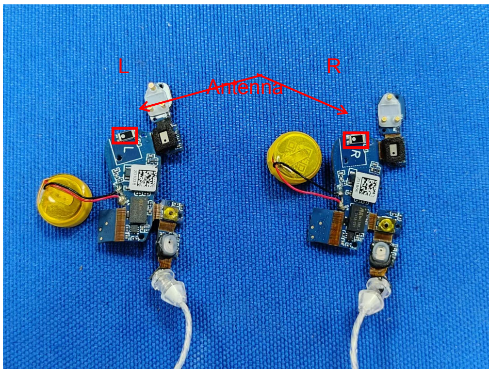
Figure 5. PCB view of Hearing Aids
