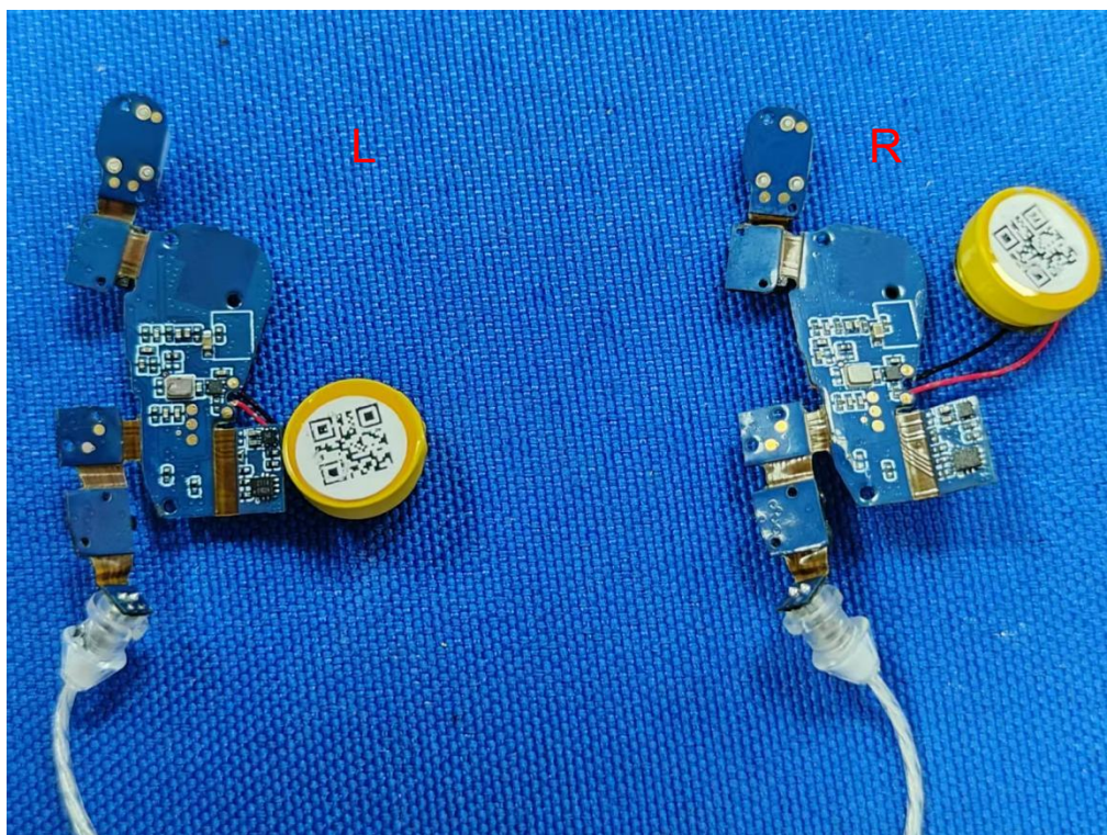
Figure 6. PCB view of Hearing Aids
