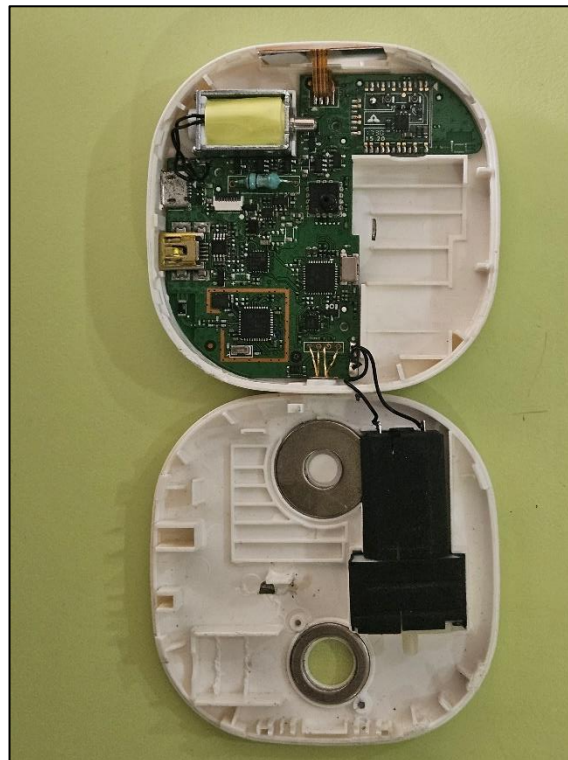
Device with enclosure opened
