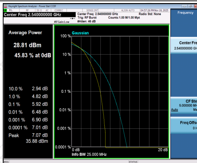
Band41-10MHz-16QAM-40090-50RB#0
