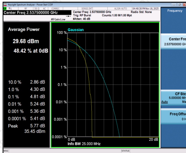
Band41-5MHz-16QAM-40065-1RB#0
