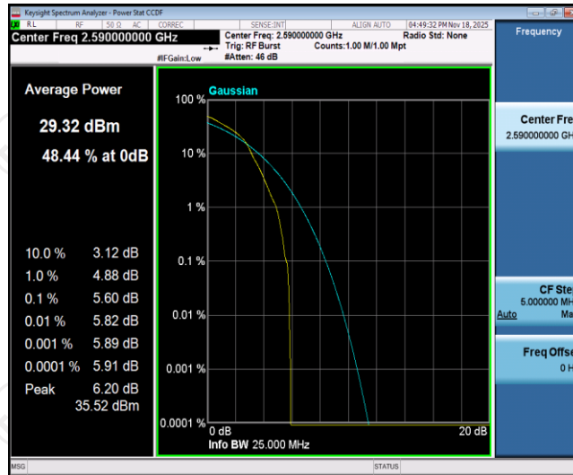
Band41-5MHz-16QAM-40590-1RB#0
