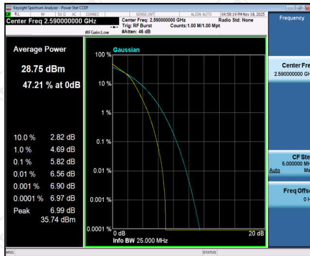
Band41-10MHz-16QAM-40590-50RB#0
