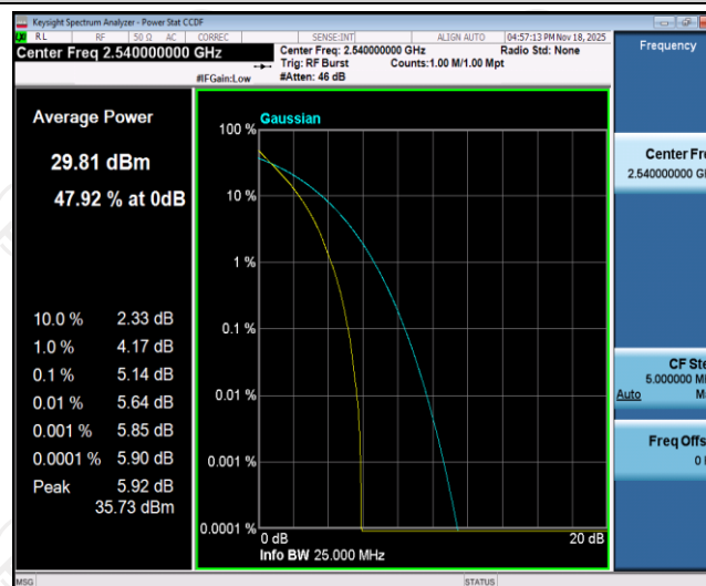
Band41-10MHz-QPSK-40090-50RB#0
