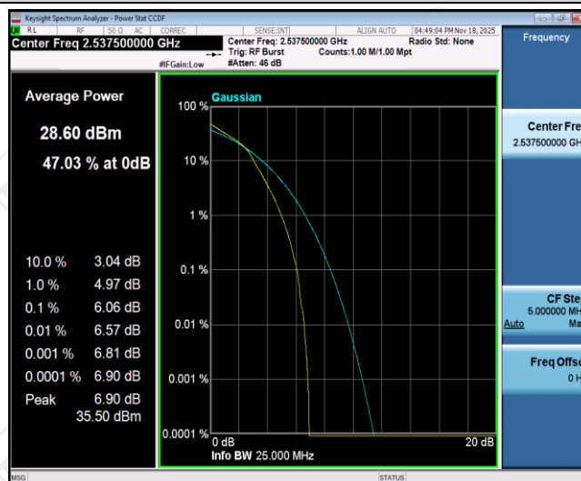
Band41-5MHz-16QAM-40065-25RB#0
