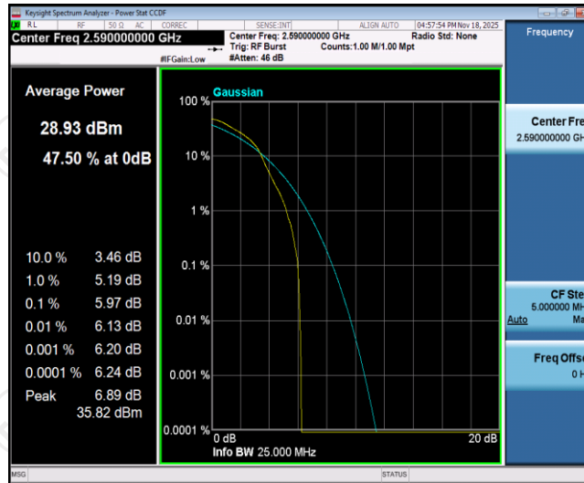
Band41-10MHz-16QAM-40590-1RB#0
