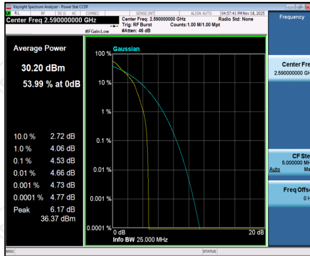
Band41-10MHz-QPSK-40590-1RB#0
