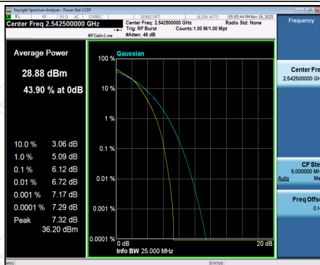
Band41-15MHz-16QAM-40115-75RB#0
