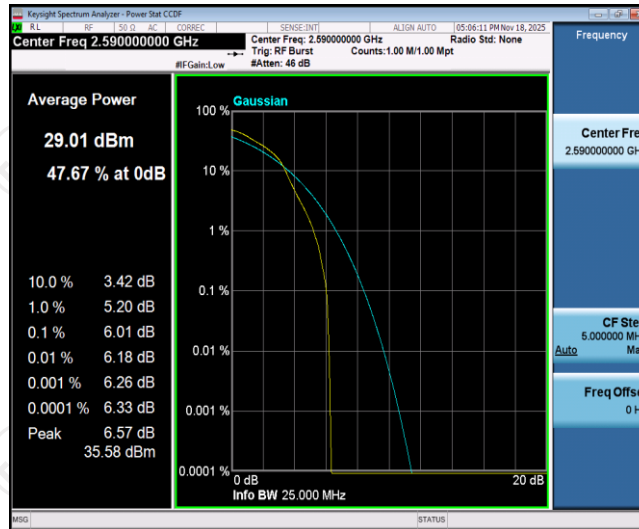
Band41-15MHz-16QAM-40590-1RB#0
