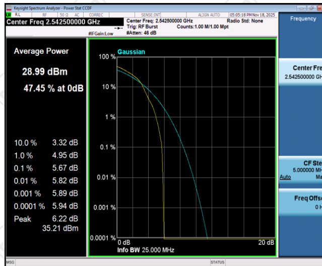
Band41-15MHz-16QAM-40115-1RB#0
