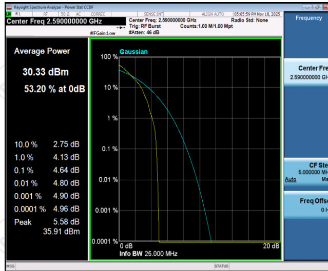
Band41-15MHz-QPSK-40590-1RB#0
