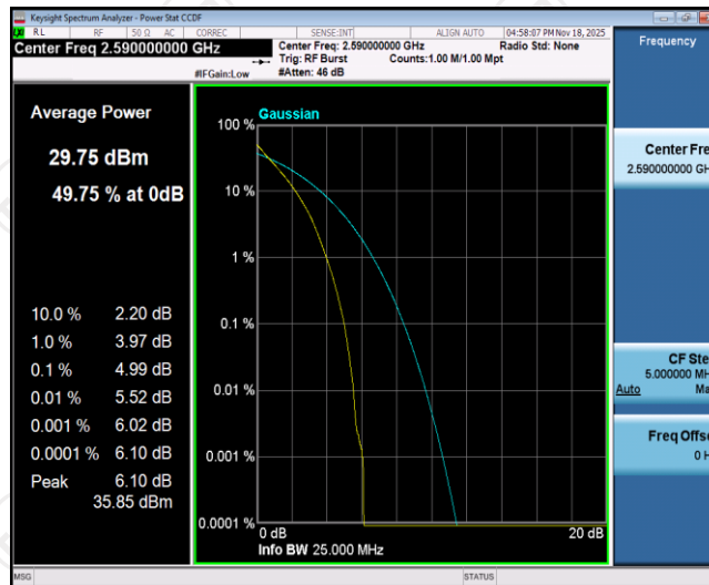
Band41-10MHz-QPSK-40590-50RB#0
