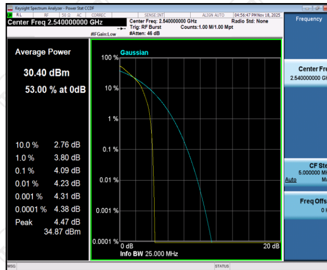
Band41-10MHz-QPSK-40090-1RB#0
