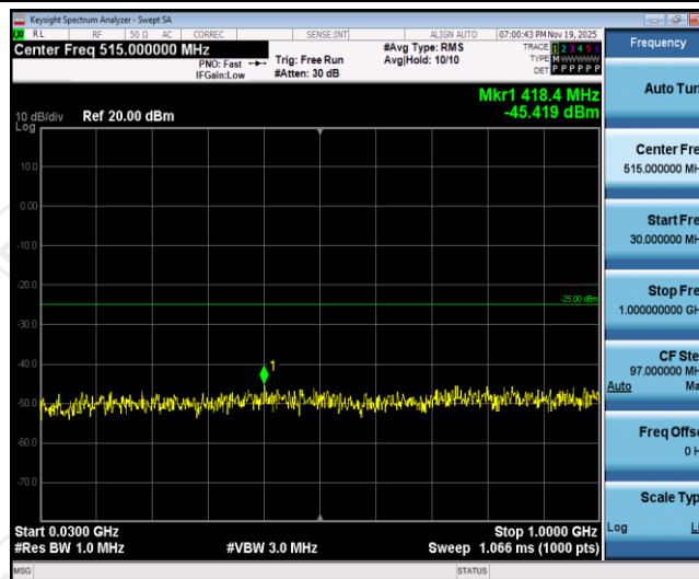
Band41-5MHz-QPSK-40590-1RB#0-Range1:30~1000MHz
