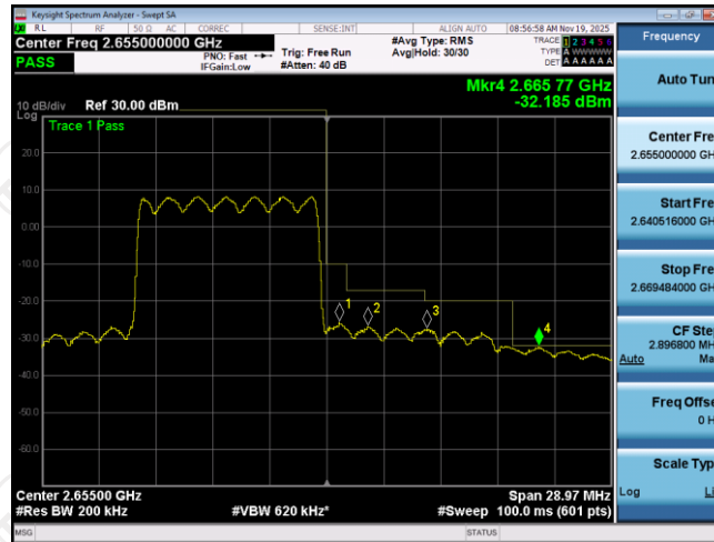
Band41-10MHz-16QAM-41190-50RB#0
