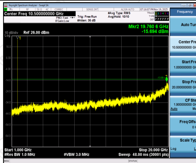
Band66-1.4MHz-QPSK-131979-1RB#0-Range2:1000~20000MHz
