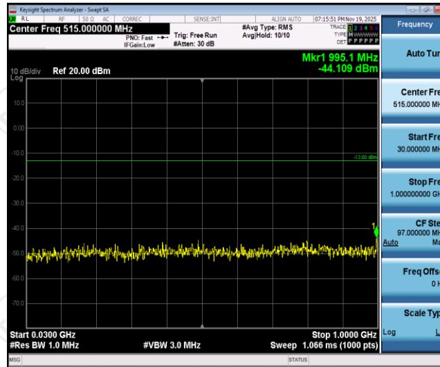
Band66-1.4MHz-QPSK-131979-1RB#0-Range1:30~1000MHz
