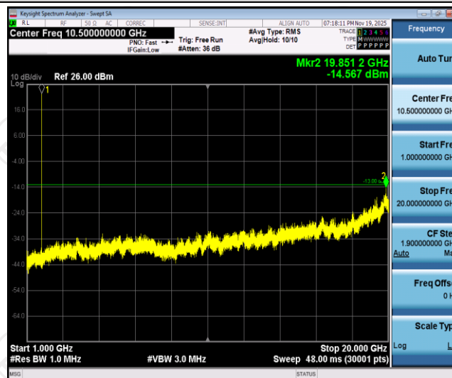
Band66-1.4MHz-QPSK-132665-1RB#0-Range2:1000~20000MHz
