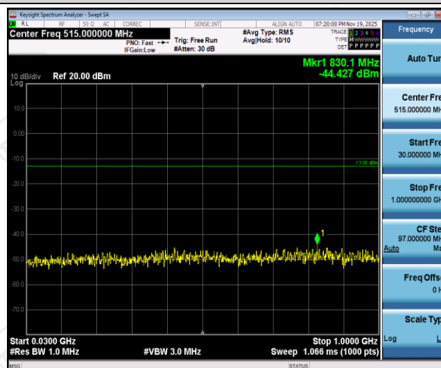
Band66-3MHz-QPSK-132322-1RB#0-Range1:30~1000MHz
