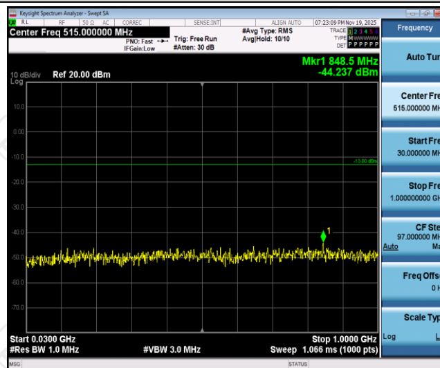
Band66-5MHz-QPSK-132322-1RB#0-Range1:30~1000MHz
