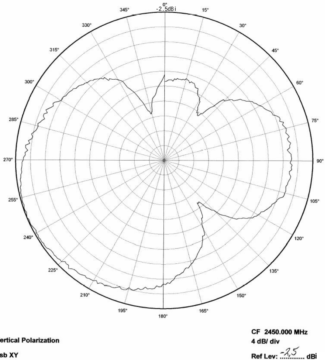
Figure 7: USB Dongle XY Plane
