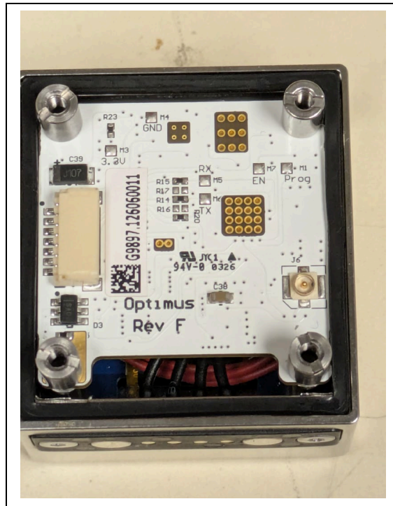
Board Bottom
