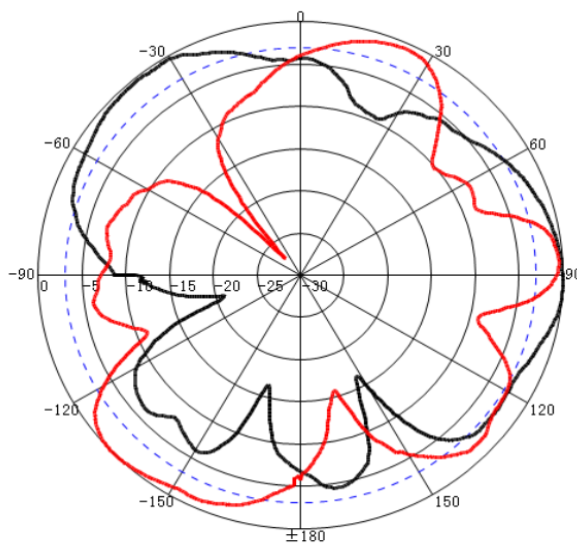
Antenna Radiation Pattern VS Gain
