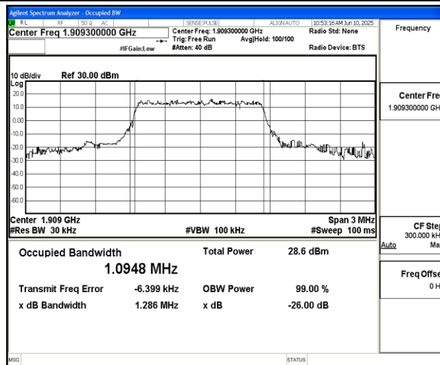
Band2-1.4MHz-16QAM-19193-6-0-High-1.0948-1.286-PASS
