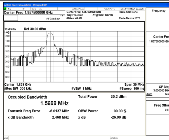
Band2-15MHz-QPSK-18675-6-0-Low-1.5699-2.468-PASS
