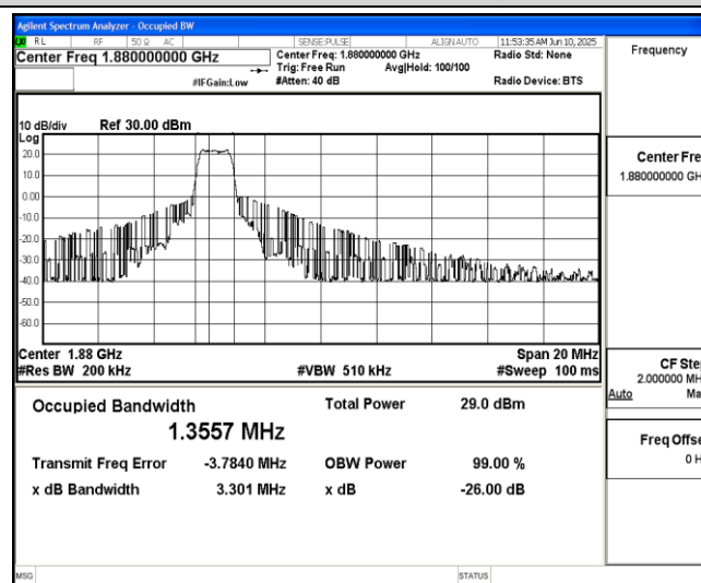
Band2-10MHz-16QAM-18900-6-0-Low-1.3557-3.301-PASS
