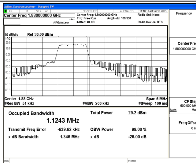
Band2-3MHz-QPSK-18900-6-0-Low-1.1243-1.346-PASS
