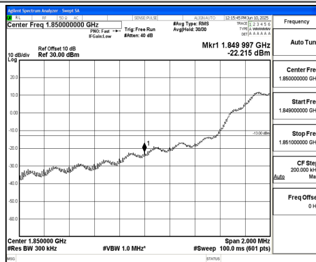
Band2-15MHz-QPSK-18675-6-0-Low--22.22-PASS
