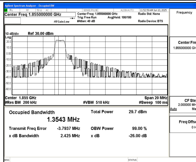
Band2-10MHz-16QAM-18650-6-0-Low-1.3543-2.425-PASS
