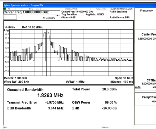
Band2-15MHz-16QAM-18900-6-0-Low-1.8263-3.644-PASS
