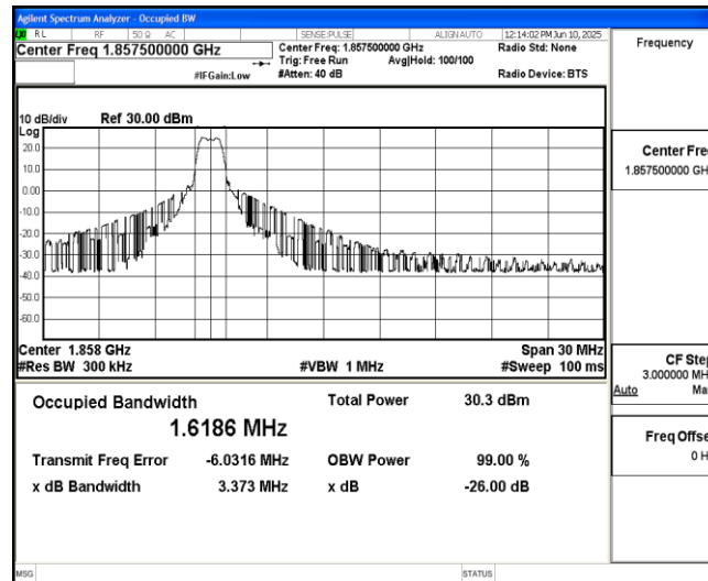
Band2-15MHz-16QAM-18675-6-0-Low-1.6186-3.373-PASS
