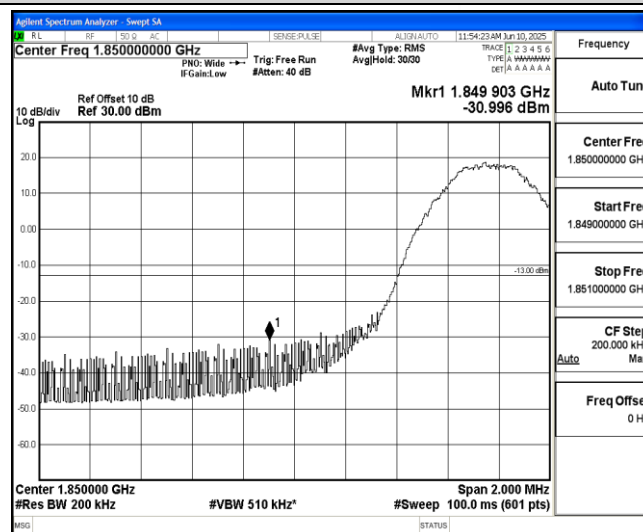
Band2-10MHz-QPSK-18650-1-0-Low--31.00-PASS
