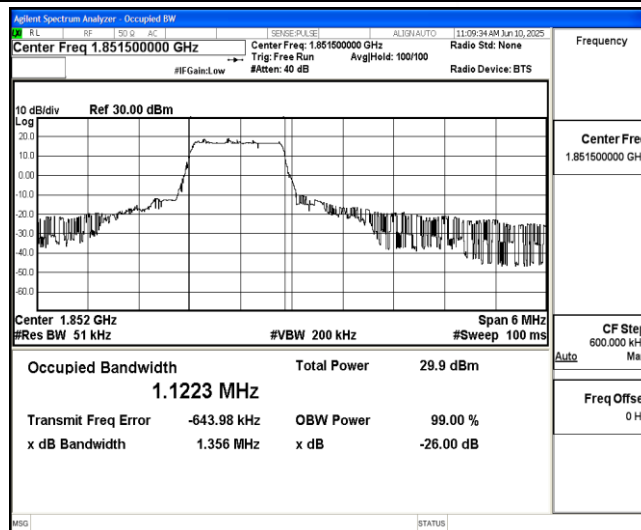
Band2-3MHz-QPSK-18615-6-0-Low-1.1223-1.356-PASS
