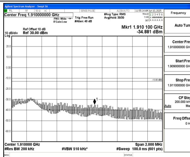
Band2-10MHz-16QAM-19150-1-0-High--34.88-PASS
