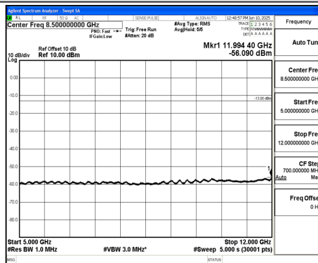
Band2-20MHz-16QAM-19100-1-0-High-5000-12000--56.09-PASS
