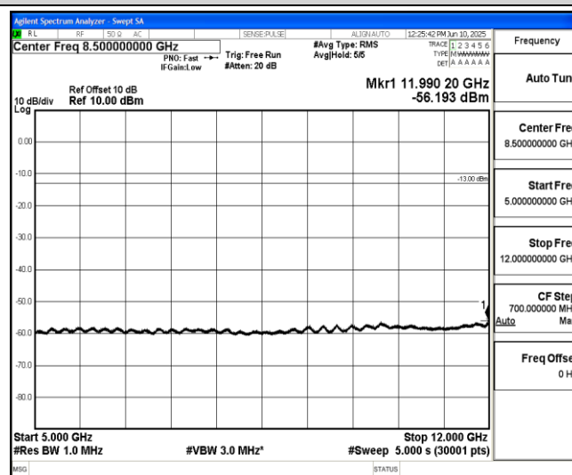
Band2-15MHz-QPSK-19125-1-0-High-5000-12000--56.19-PASS
