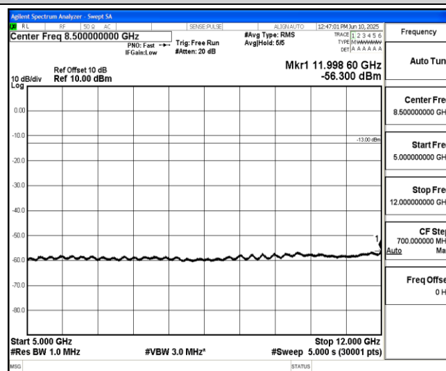
Band2-20MHz-QPSK-19100-1-0-High-5000-12000--56.3-PASS
