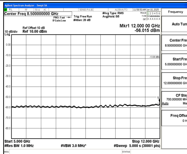
Band2-10MHz-16QAM-18650-1-0-Low-5000-12000--56.02-PASS
