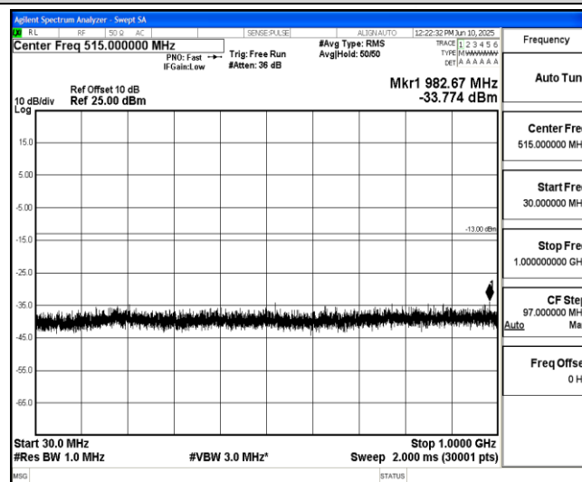
Band2-15MHz-16QAM-18900-1-0-Low-30-1000--33.77-PASS
