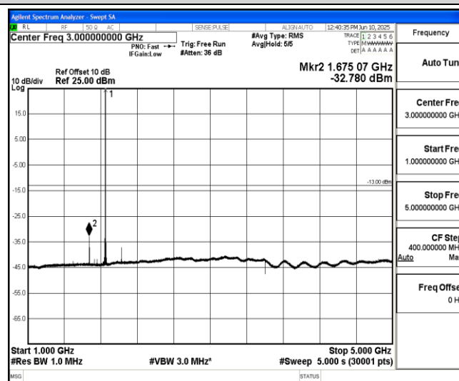
Band2-20MHz-16QAM-18700-1-0-Low-1000-5000--32.78-PASS
