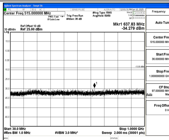
Band2-10MHz-16QAM-18900-1-0-Low-30-1000--34.28-PASS
