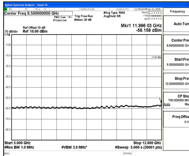
Band2-20MHz-16QAM-18900-1-0-Low-5000-12000--56.16-PASS
