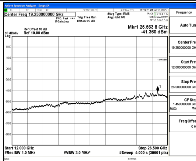
Band2-10MHz-16QAM-18650-1-0-Low-12000-26500--41.36-PASS
