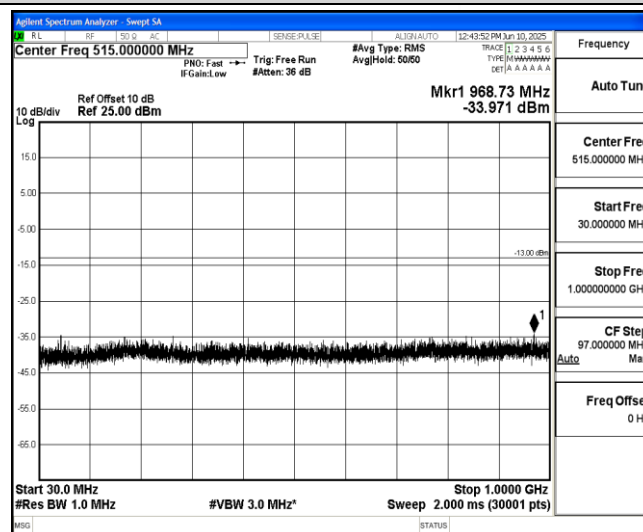
Band2-20MHz-16QAM-18900-1-0-Low-30-1000--33.97-PASS
