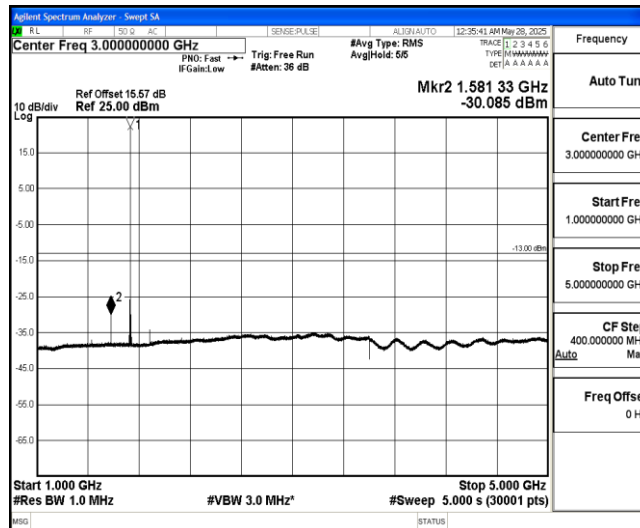
Band4-1.4MHz-QPSK-20175-1-0-Low-1000-5000--30.09-PASS
