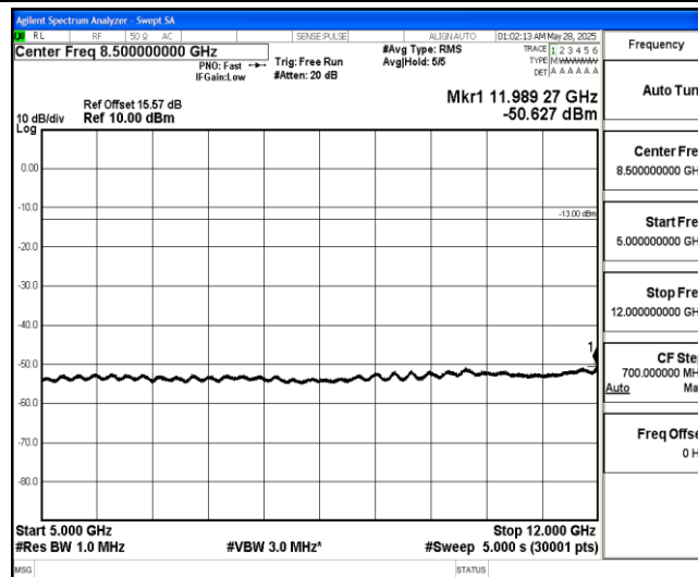
Band4-3MHz-16QAM-19965-1-0-Low-5000-12000--50.63-PASS
