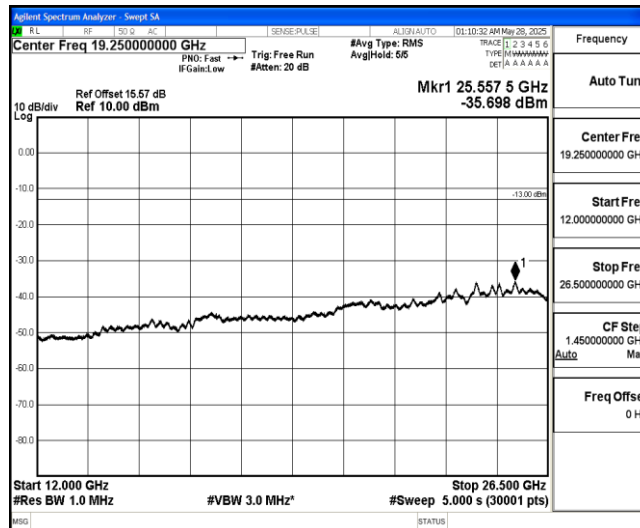
Band4-3MHz-16QAM-20385-1-0-High-12000-26500--35.7-PASS
