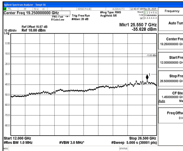
Band4-1.4MHz-QPSK-20393-1-0-High-12000-26500--35.63-PASS
