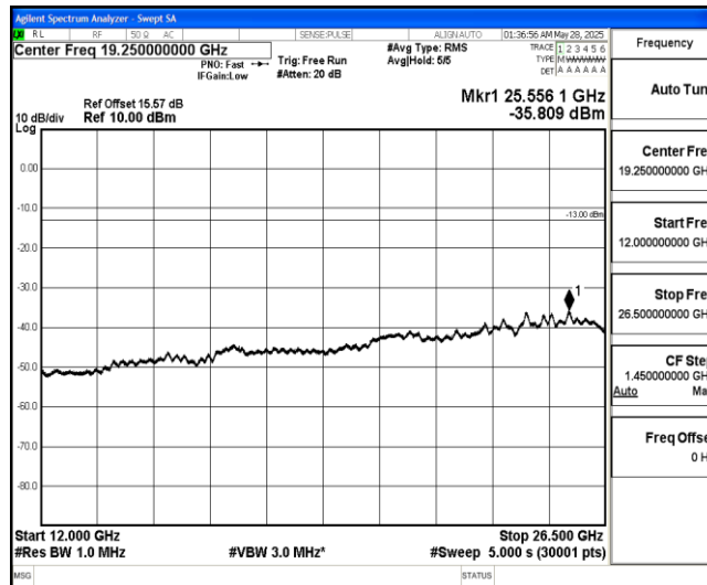
Band4-5MHz-QPSK-20375-1-0-High-12000-26500--35.81-PASS
