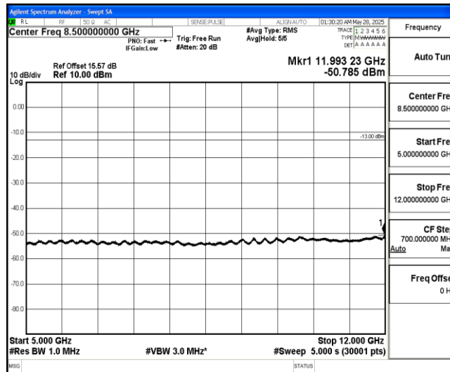
Band4-5MHz-16QAM-19975-1-0-Low-5000-12000--50.79-PASS
