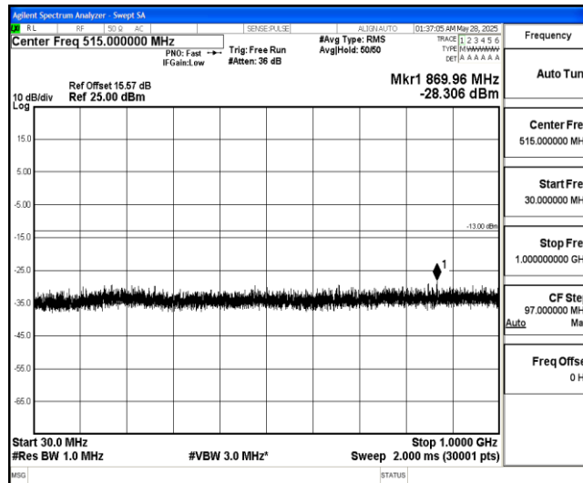
Band4-5MHz-16QAM-20375-1-0-High-30-1000--28.31-PASS
