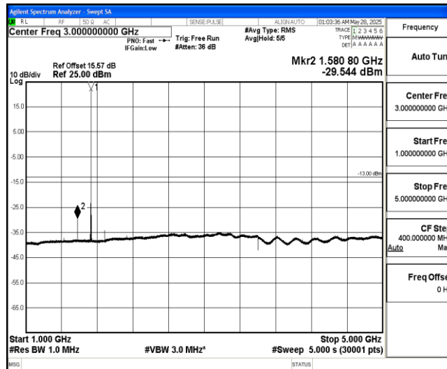
Band4-3MHz-QPSK-20175-1-0-Low-1000-5000--29.54-PASS
