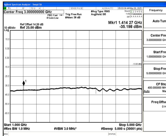
Band12-1.4MHz-16QAM-23095-1-0-Low-1000-5000--35.2-PASS
