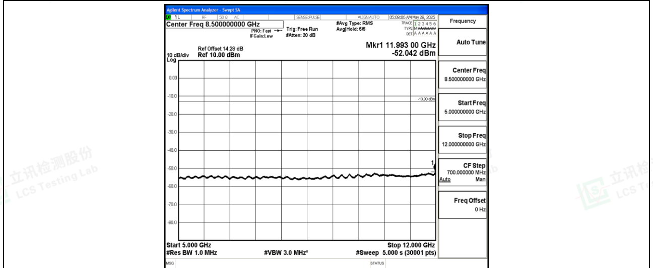
Band12-1.4MHz-16QAM-23173-1-0-High-5000-12000--52.04-PASS
