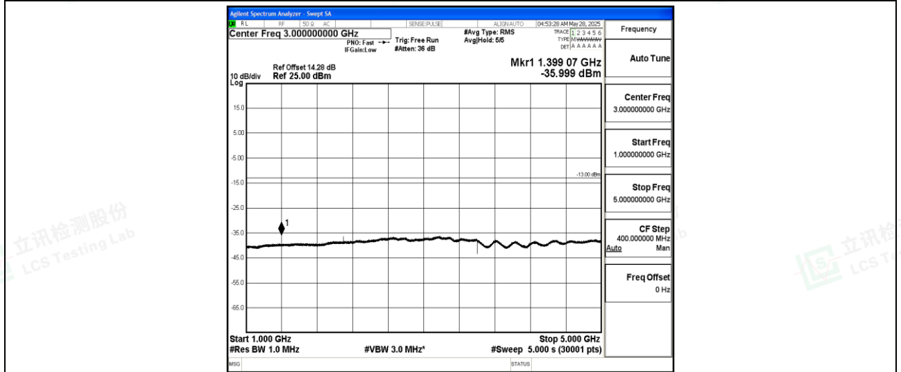
Band12-3MHz-16QAM-23025-1-0-Low-1000-5000--36-PASS
