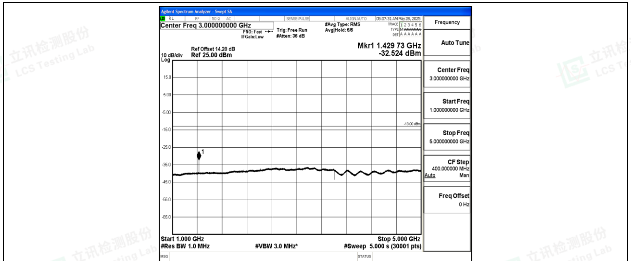
Band12-1.4MHz-16QAM-23173-1-0-High-1000-5000--32.52-PASS
