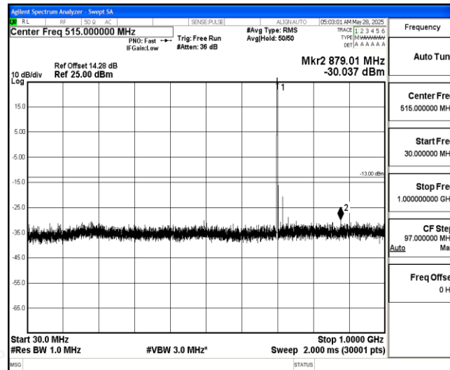
Band12-1.4MHz-16QAM-23095-1-0-Low-30-1000--30.04-PASS
