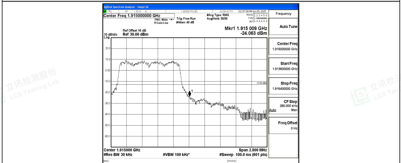
Band25-1.4MHz-QPSK-26683-6-0-High--24.06-PASS
