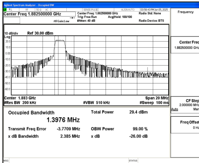
Band25-10MHz-16QAM-26365-6-0-Low-1.3976-2.385-PASS
