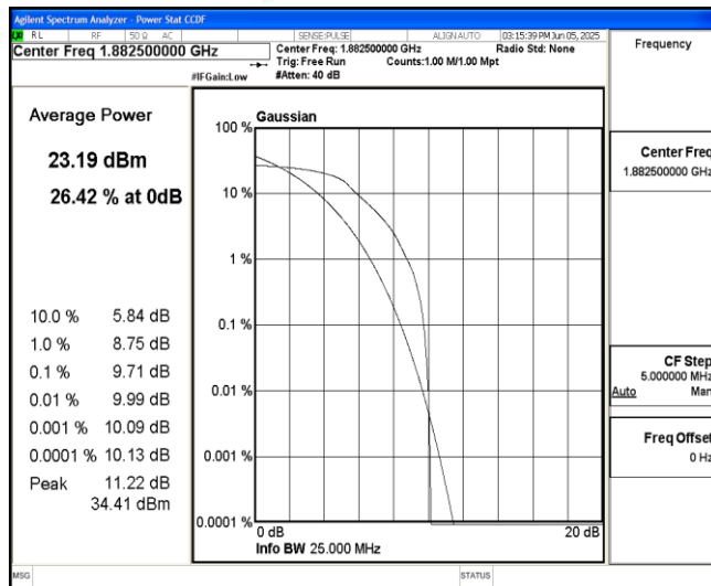
Band25-5MHz-QPSK-26365-6-0-Low-9.71-≤13-PASS
