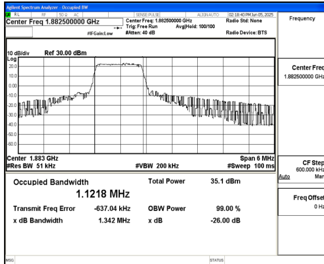
Band25-3MHz-QPSK-26365-6-0-Low-1.1218-1.342-PASS
