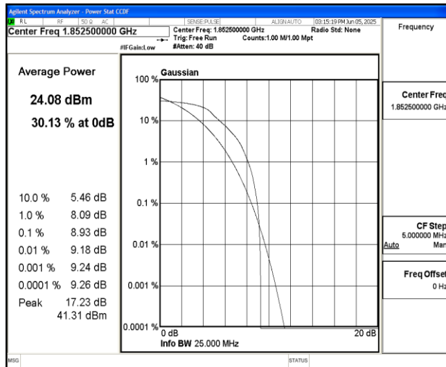
Band25-5MHz-QPSK-26065-6-0-Low-8.93-≤13-PASS
