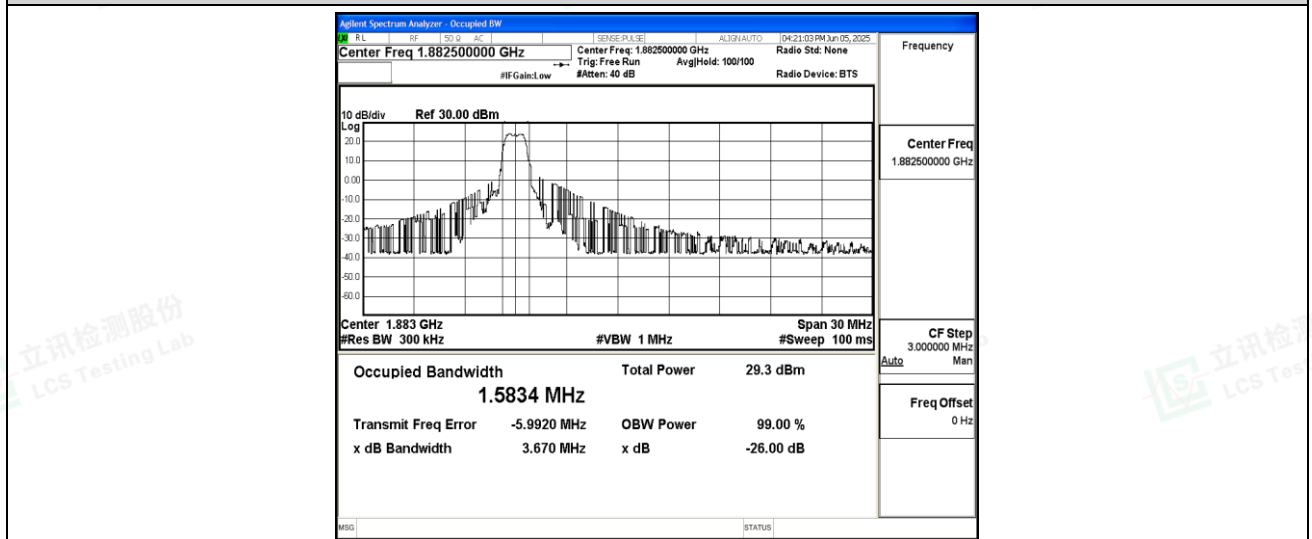
Band25-15MHz-16QAM-26365-6-0-Low-1.5834-3.670-PASS
