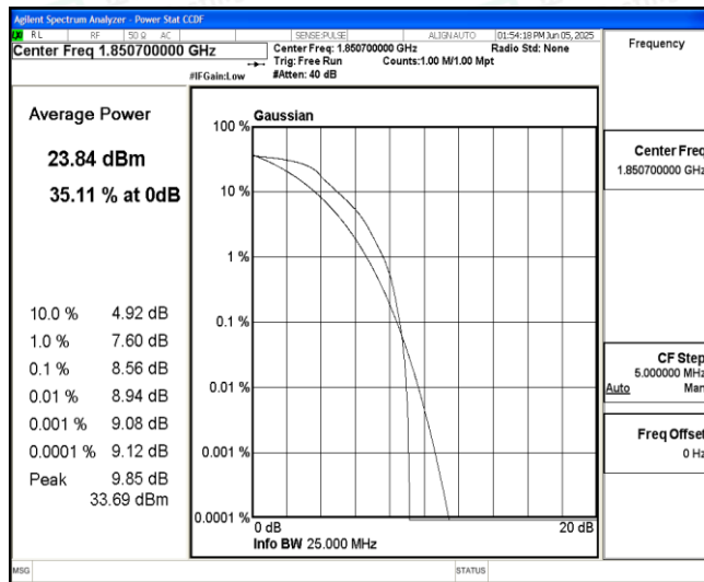
Band25-1.4MHz-QPSK-26047-6-0-Low-8.56-&lt;=13-PASS
