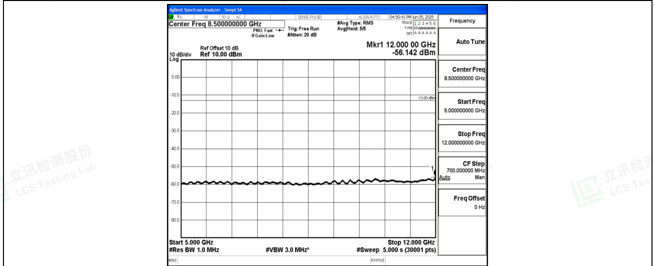
Band25-20MHz-16QAM-26365-1-0-Low-5000-12000--56.14-PASS
