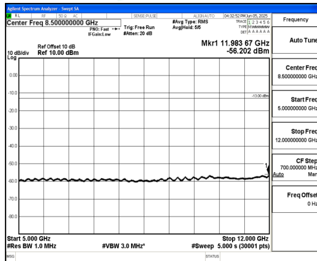
Band25-15MHz-16QAM-26615-1-0-High-5000-12000--56.2-PASS
