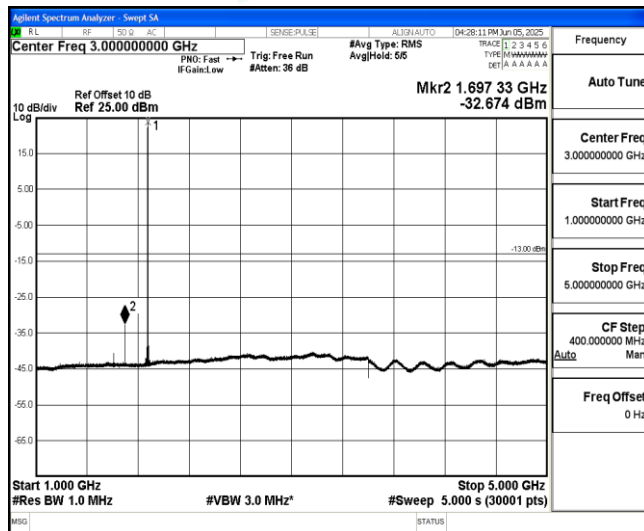
Band25-15MHz-16QAM-26365-1-0-Low-1000-5000--32.67-PASS
