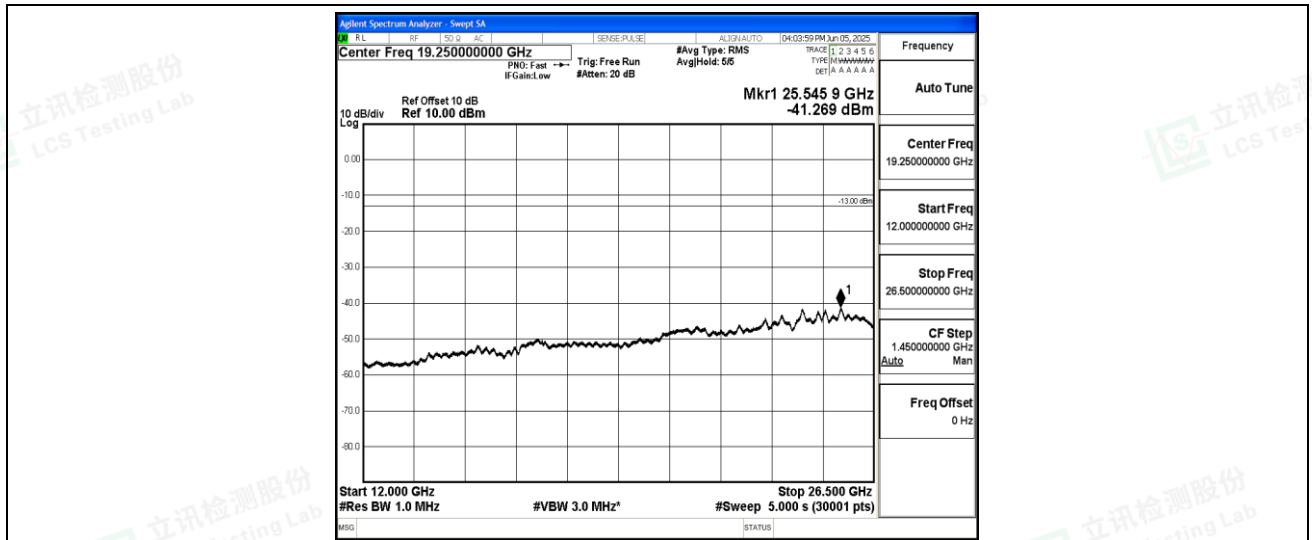
Band25-10MHz-16QAM-26090-1-0-Low-12000-26500--41.27-PASS
