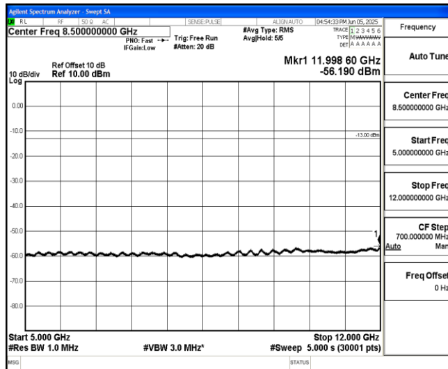
Band25-20MHz-16QAM-26590-1-0-High-5000-12000--56.19-PASS
