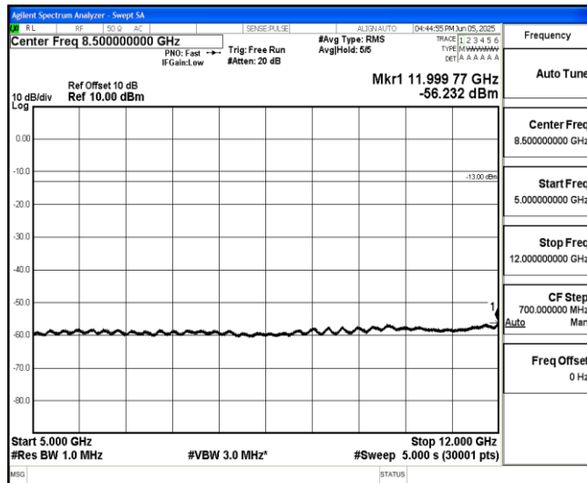
Band25-20MHz-QPSK-26140-1-0-Low-5000-12000--56.23-PASS
