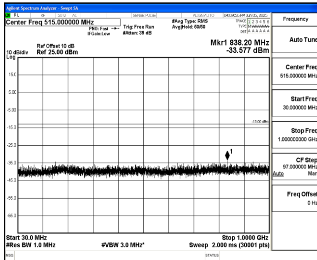
Band25-10MHz-16QAM-26640-1-0-High-30-1000--33.58-PASS
