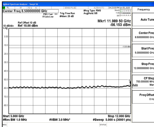
Band25-15MHz-QPSK-26115-1-0-Low-5000-12000--56.15-PASS
