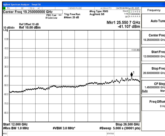
Band25-20MHz-16QAM-26590-1-0-High-12000-26500--41.11-PASS
