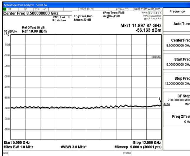
Band25-10MHz-QPSK-26640-1-0-High-5000-12000--56.16-PASS
