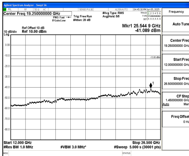
Band25-20MHz-QPSK-26140-1-0-Low-12000-26500--41.09-PASS
