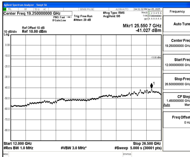
Band25-15MHz-QPSK-26615-1-0-High-12000-26500--41.03-PASS
