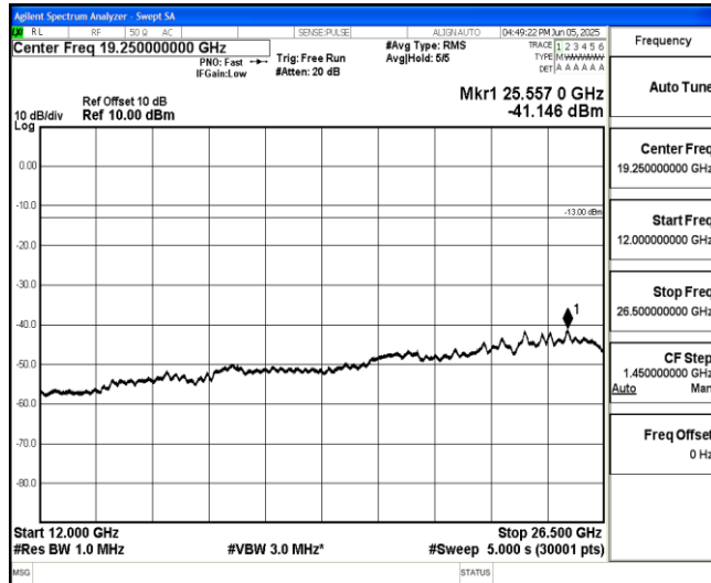
Band25-20MHz-QPSK-26365-1-0-Low-12000-26500--41.15-PASS
