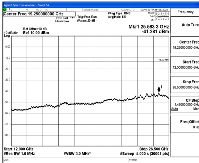
Band25-5MHz-16QAM-26365-1-0-Low-12000-26500--41.28-PASS
