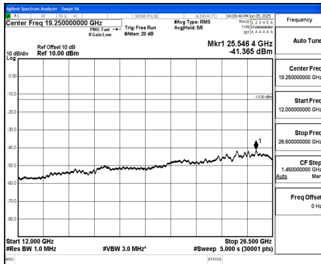
Band25-10MHz-QPSK-26640-1-0-High-12000-26500--41.37-PASS
