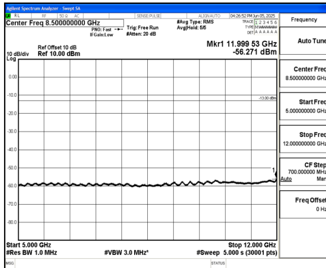
Band25-15MHz-QPSK-26365-1-0-Low-5000-12000--56.27-PASS
