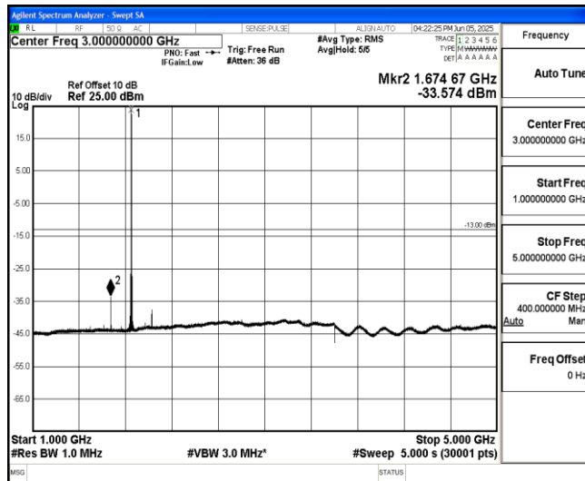
Band25-15MHz-QPSK-26115-1-0-Low-1000-5000--33.57-PASS
