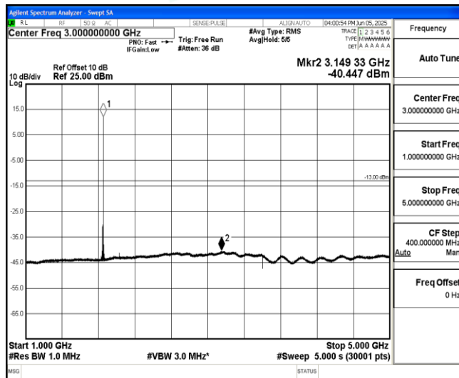
Band25-10MHz-QPSK-26090-1-0-Low-1000-5000--40.45-PASS
