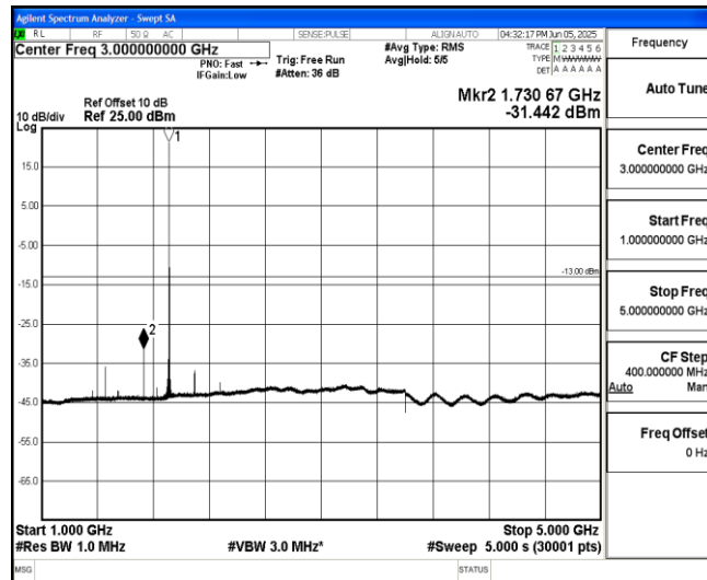
Band25-15MHz-16QAM-26615-1-0-High-1000-5000--31.44-PASS
