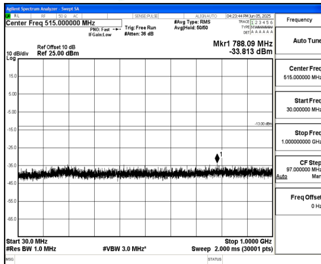
Band25-15MHz-16QAM-26115-1-0-Low-30-1000--33.81-PASS
