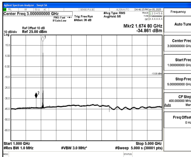
Band25-20MHz-16QAM-26140-1-0-Low-1000-5000--34.86-PASS
