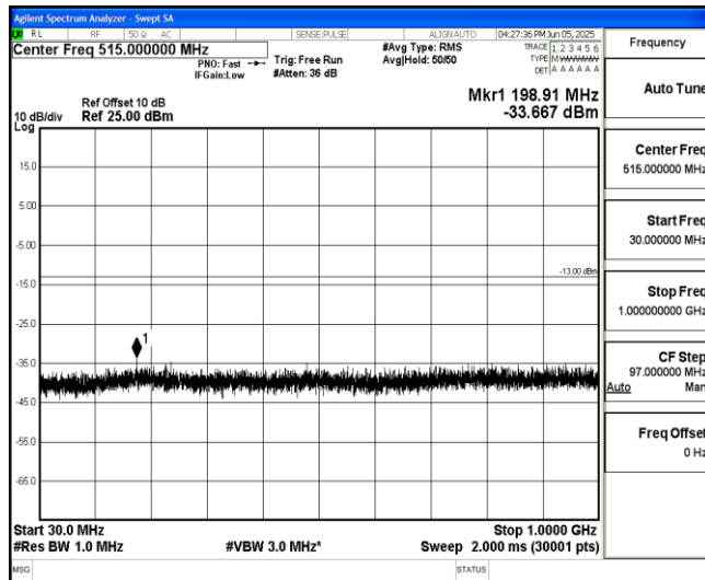
Band25-15MHz-16QAM-26365-1-0-Low-30-1000--33.67-PASS
