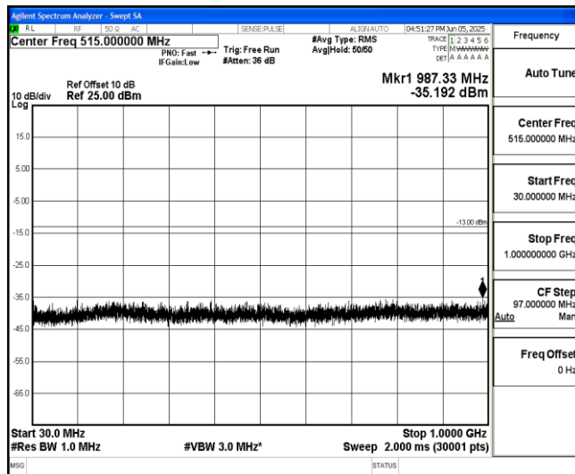
Band25-20MHz-QPSK-26590-1-0-High-30-1000--35.19-PASS
