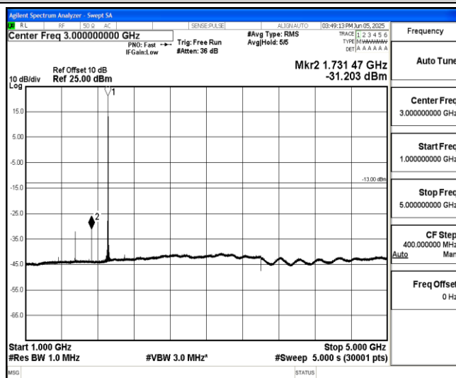
Band25-5MHz-16QAM-26665-1-0-High-30-1000--33.85-PASS
