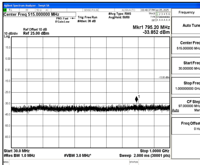
Band25-5MHz-16QAM-26665-1-0-High-30-1000--33.85-PASS
