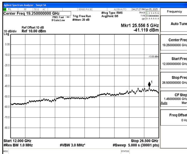
Band25-15MHz-QPSK-26365-1-0-Low-12000-26500--41.12-PASS
