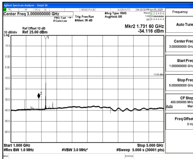
Band25-10MHz-16QAM-26640-1-0-High-1000-5000--34.12-PASS
