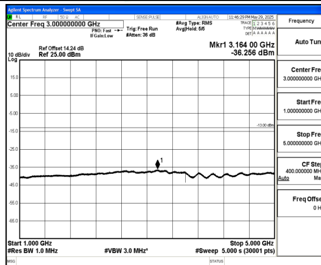
Band26-3MHz-16QAM-26775-1-0-High-1000-5000--36.26-PASS
