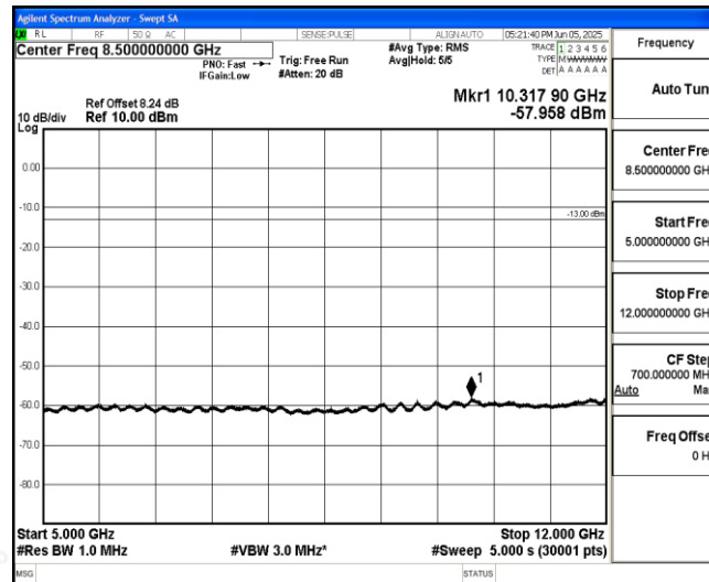
Band26-5MHz-16QAM-26715-1-0-Low-5000-12000--57.96-PASS
