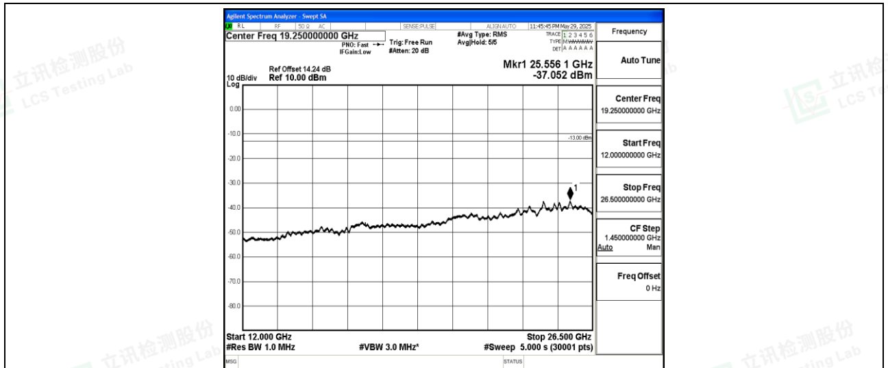
Band26-3MHz-QPSK-26775-1-0-High-12000-26500--37.05-PASS
