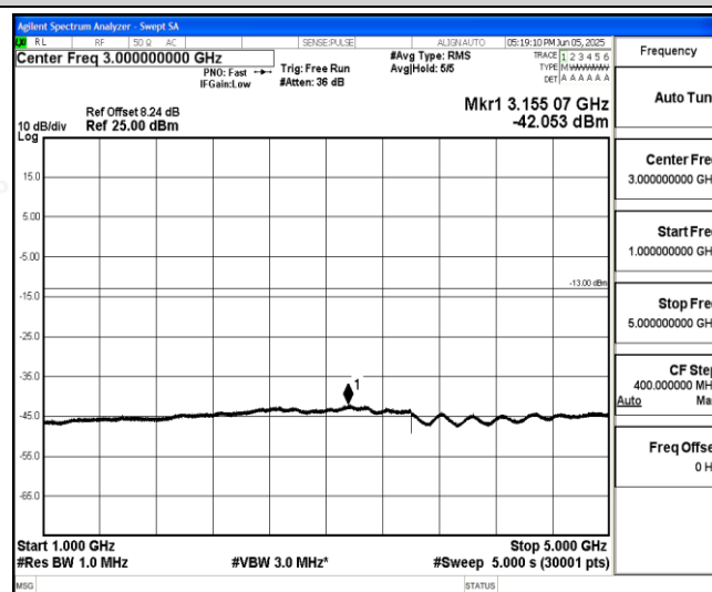
Band26-5MHz-QPSK-26715-1-0-Low-1000-5000--42.05-PASS
