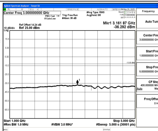
Band26-1.4MHz-16QAM-26697-1-0-Low-1000-5000--36.29-PASS
