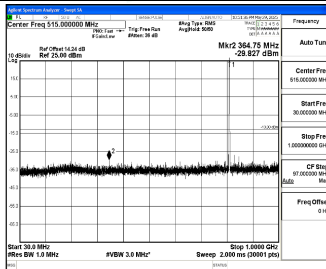
Band26-1.4MHz-16QAM-26697-1-0-Low-30-1000--29.83-PASS
