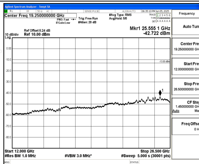
Band26-10MHz-16QAM-26740-1-0-Low-12000-26500--42.72-PASS
