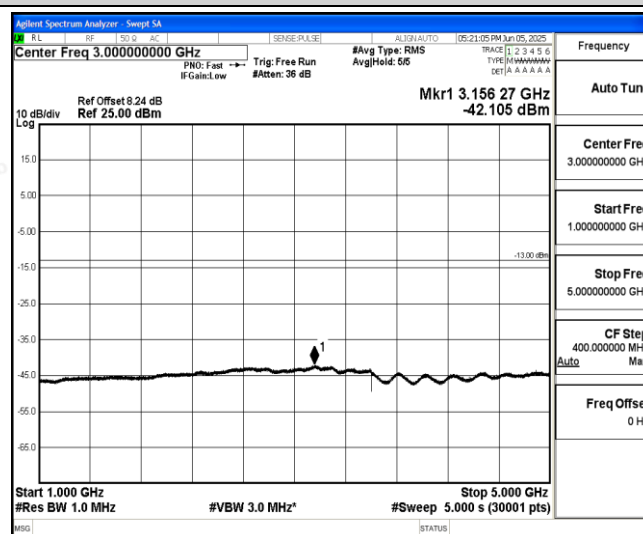
Band26-5MHz-16QAM-26715-1-0-Low-1000-5000--42.11-PASS
