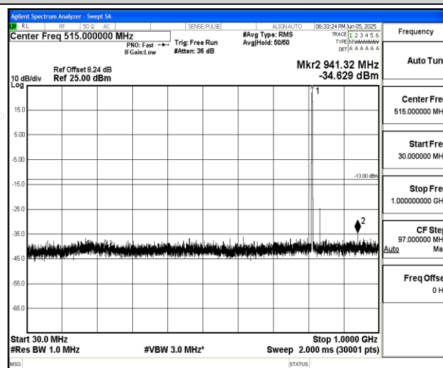
Band26-10MHz-16QAM-26740-1-0-Low-30-1000--34.63-PASS
