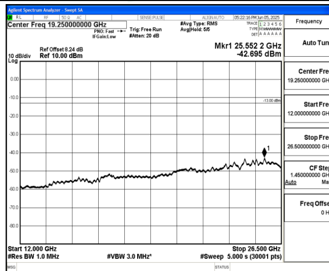
Band26-5MHz-16QAM-26715-1-0-Low-12000-26500--42.7-PASS
