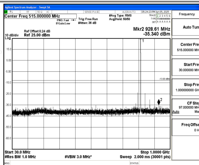
Band26-5MHz-16QAM-26740-1-0-Low-30-1000--35.34-PASS
