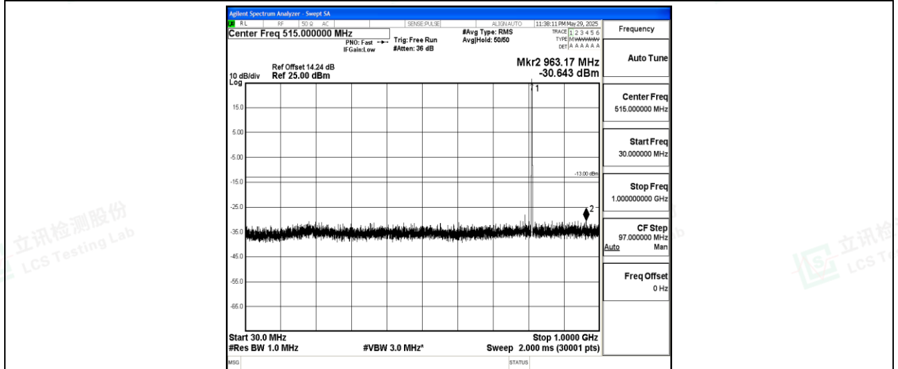
Band26-3MHz-16QAM-26705-1-0-Low-30-1000--30.64-PASS
