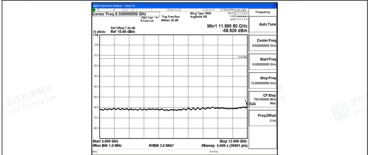
Band26-3MHz-16QAM-26915-1-0-Low-5000-12000--58.93-PASS
