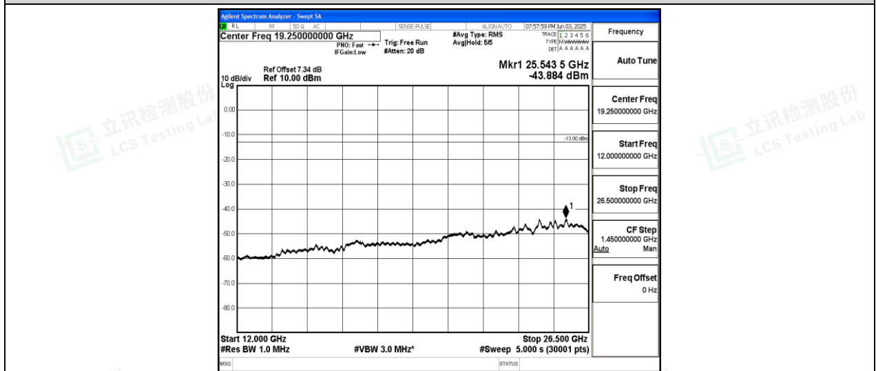
Band26-3MHz-QPSK-26915-1-0-Low-12000-26500--43.88-PASS
