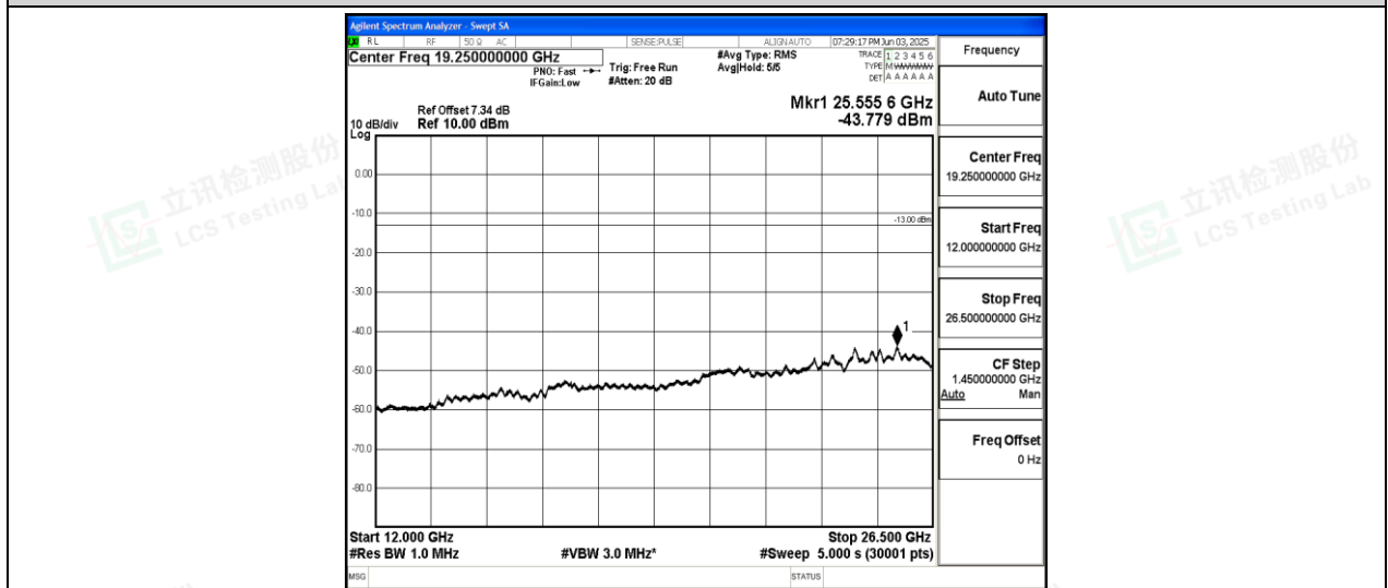
Band26-1.4MHz-16QAM-26915-1-0-Low-12000-26500--43.78-PASS
