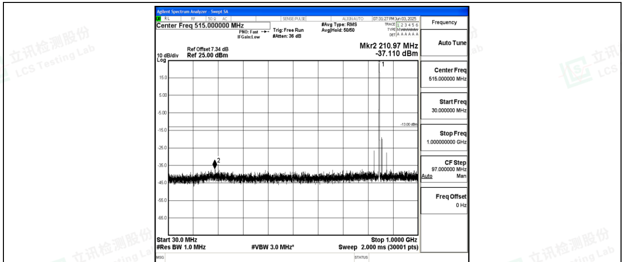
Band26-1.4MHz-16QAM-27033-1-0-High-30-1000--37.11-PASS
