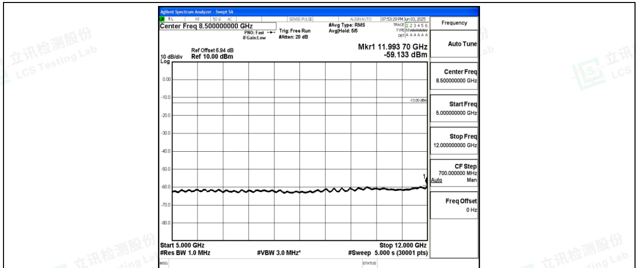
Band26-3MHz-QPSK-26805-1-0-Low-5000-12000--59.13-PASS
