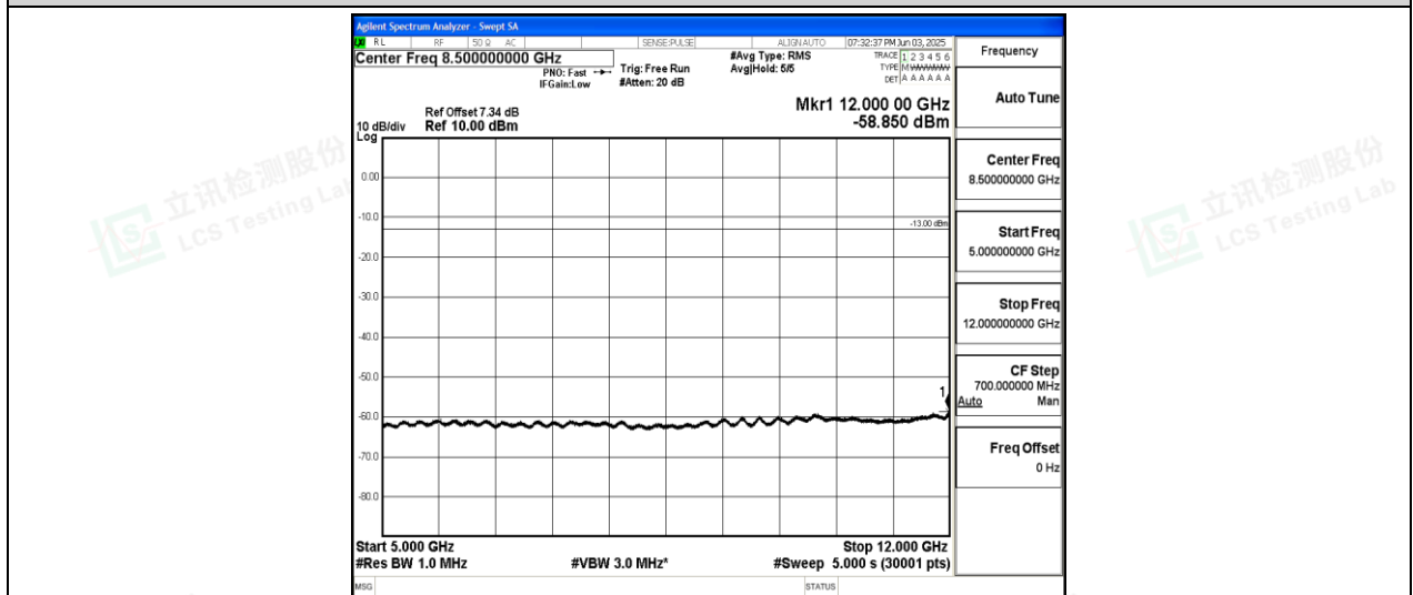
Band26-1.4MHz-16QAM-27033-1-0-High-5000-12000--58.85-PASS
