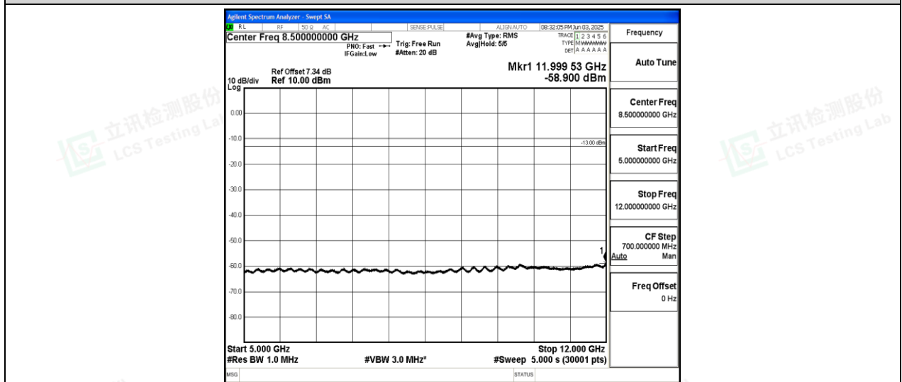
Band26-5MHz-QPSK-27015-1-0-High-5000-12000--58.9-PASS
