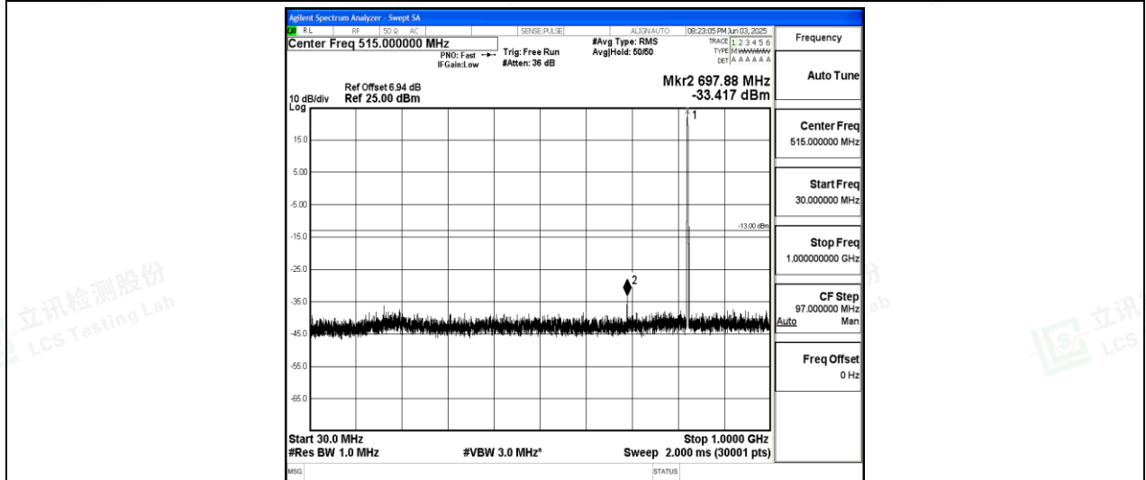
Band26-5MHz-QPSK-26815-1-0-Low-30-1000--33.42-PASS
