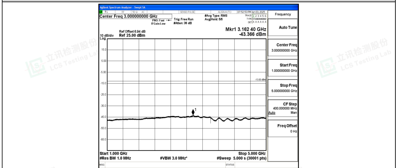
Band26-3MHz-QPSK-26805-1-0-Low-1000-5000--43.37-PASS
