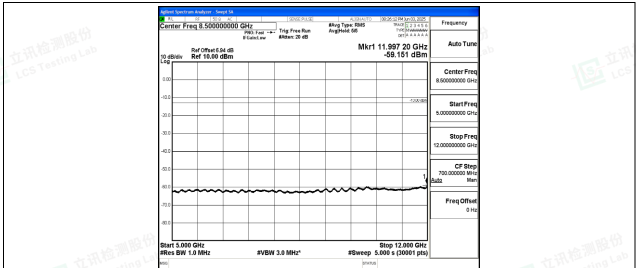
Band26-5MHz-16QAM-26815-1-0-Low-5000-12000--59.15-PASS
