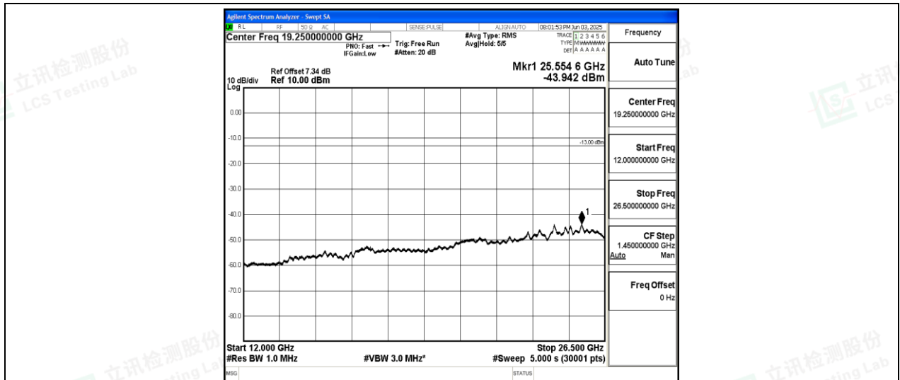
Band26-3MHz-QPSK-27025-1-0-High-12000-26500--43.94-PASS
