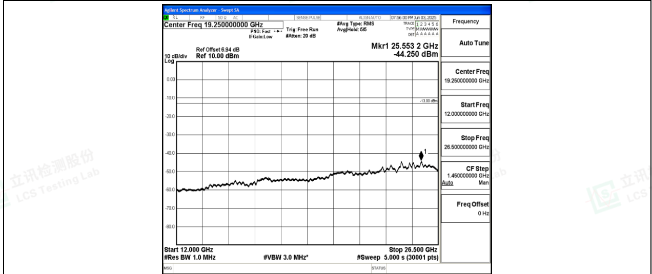
Band26-3MHz-16QAM-26805-1-0-Low-12000-26500--44.25-PASS
