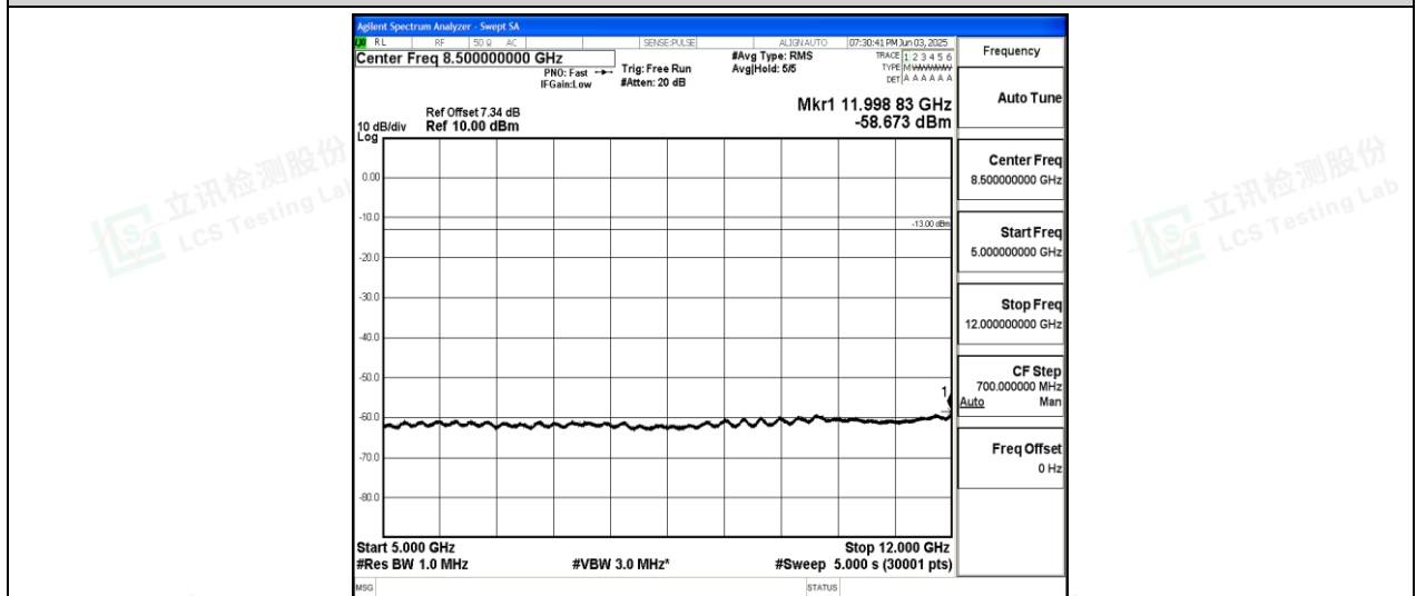
Band26-1.4MHz-QPSK-27033-1-0-High-5000-12000--58.67-PASS
