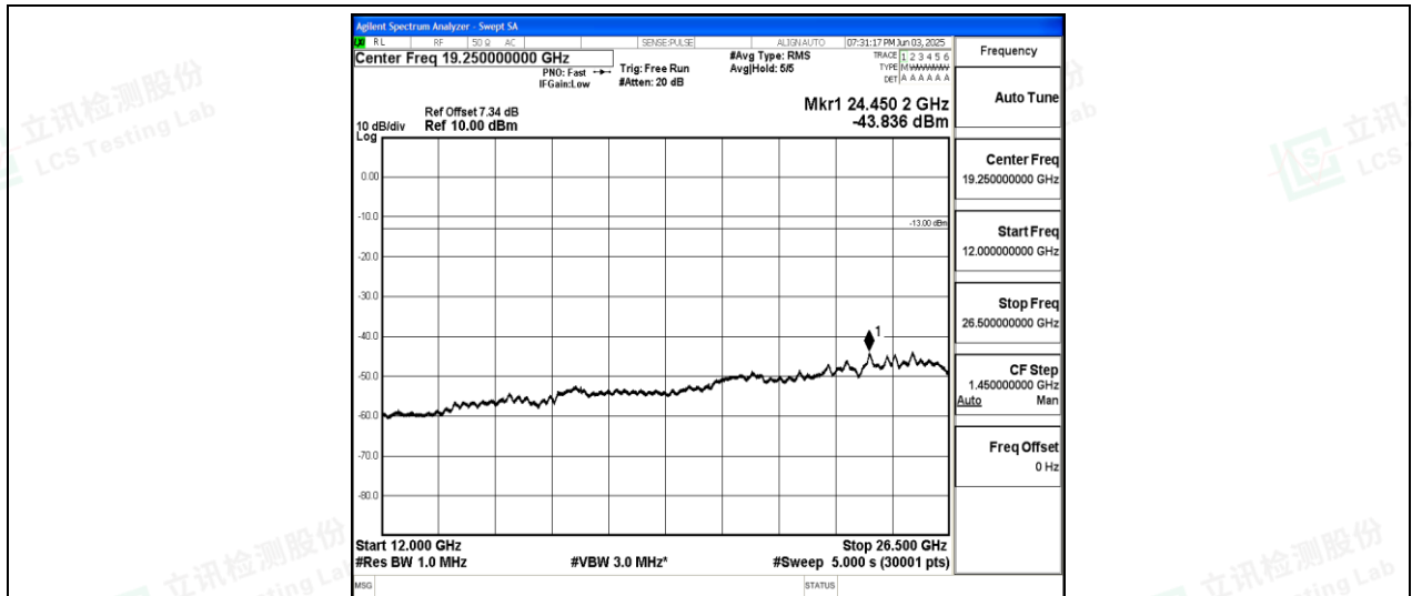
Band26-1.4MHz-QPSK-27033-1-0-High-12000-26500--43.84-PASS
