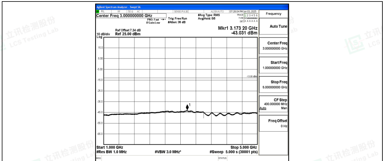
Band26-1.4MHz-16QAM-26915-1-0-Low-1000-5000--43.03-PASS
