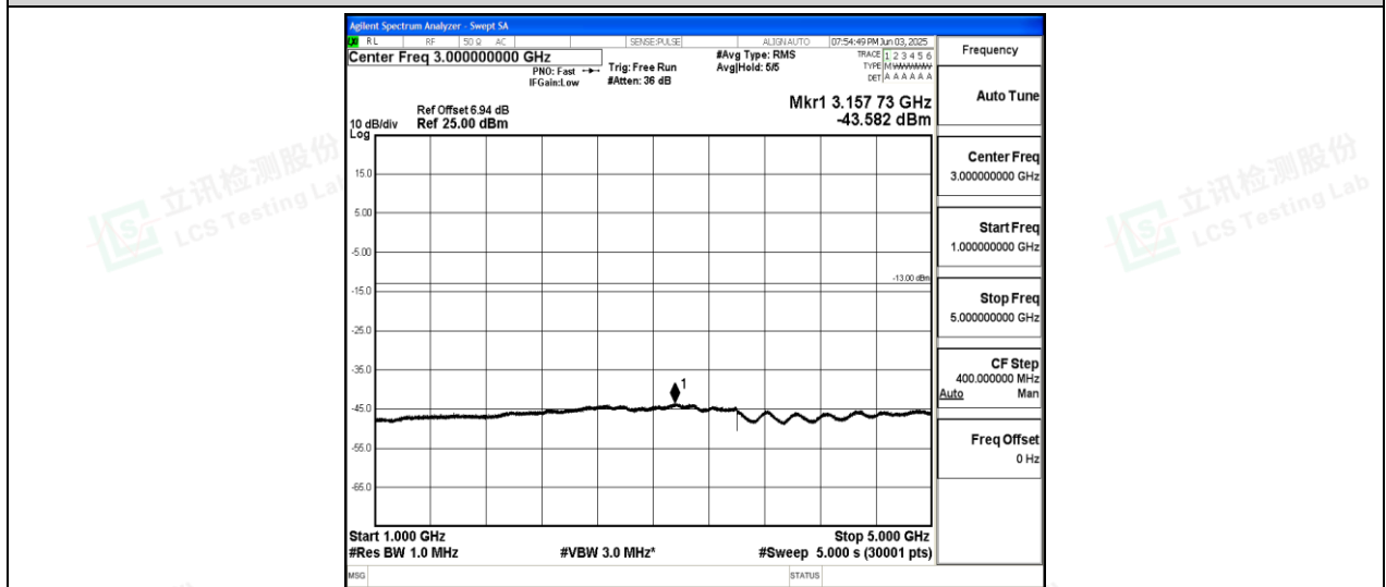
Band26-3MHz-16QAM-26805-1-0-Low-1000-5000--43.58-PASS
