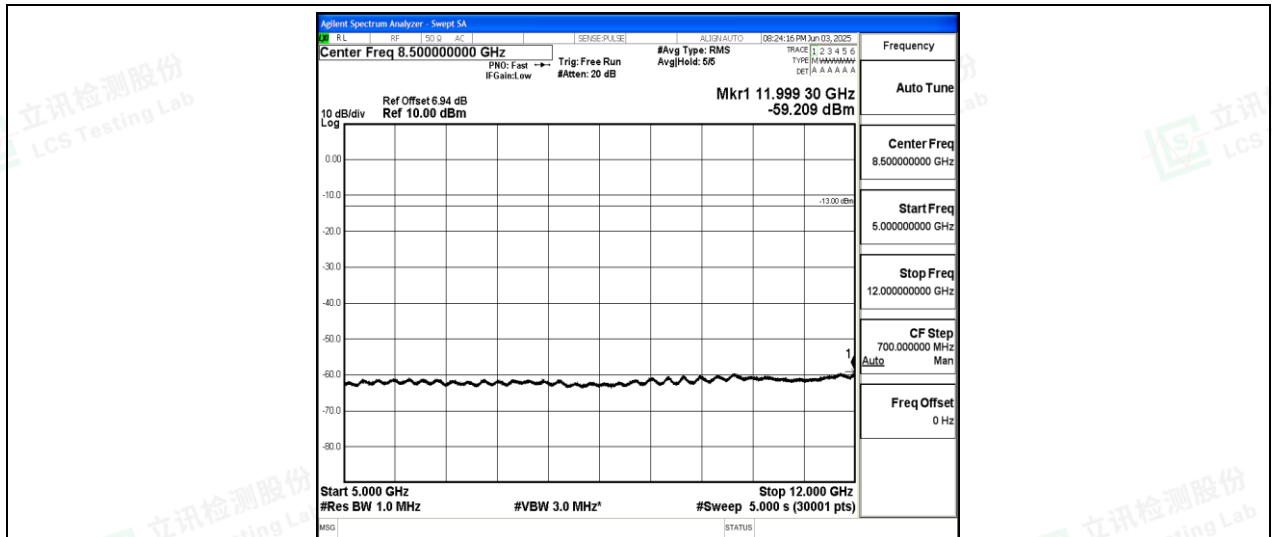
Band26-5MHz-QPSK-26815-1-0-Low-5000-12000--59.21-PASS
