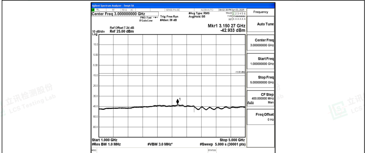
Band26-3MHz-16QAM-27025-1-0-High-1000-5000--42.93-PASS
