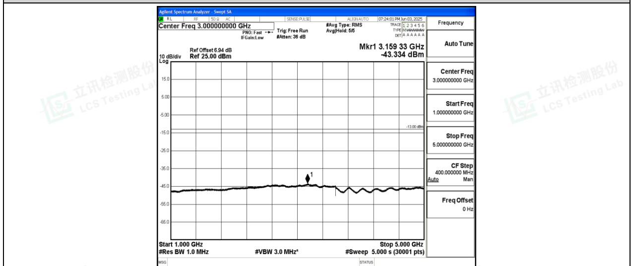
Band26-1.4MHz-16QAM-26797-1-0-Low-1000-5000--43.33-PASS
