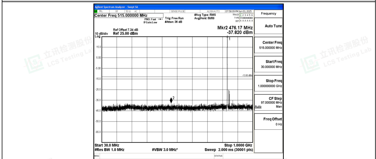
Band26-3MHz-16QAM-26915-1-0-Low-30-1000--37.82-PASS
