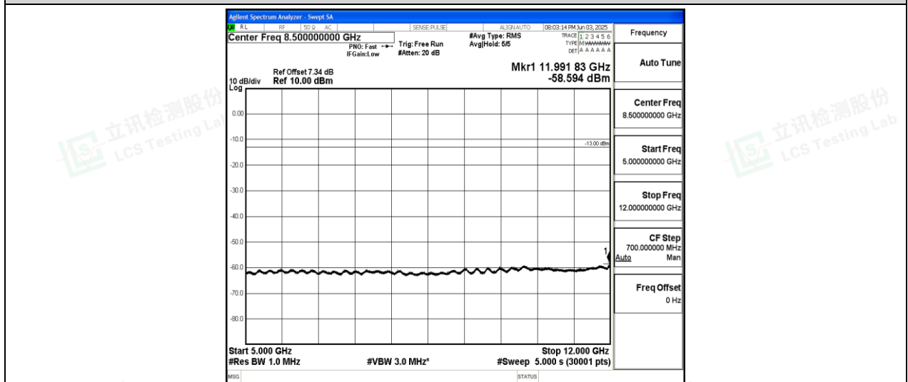
Band26-3MHz-16QAM-27025-1-0-High-5000-12000--58.59-PASS
