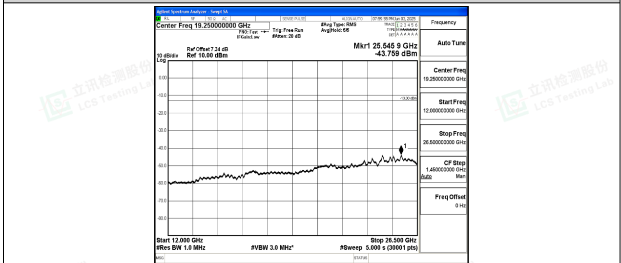
Band26-3MHz-16QAM-26915-1-0-Low-12000-26500--43.76-PASS
