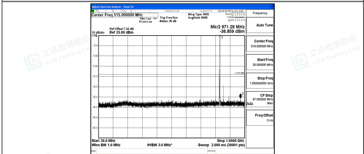
Band26-5MHz-16QAM-26915-1-0-Low-30-1000--36.86-PASS
