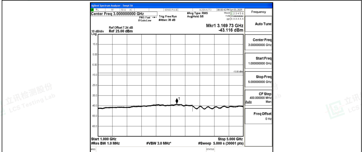
Band26-3MHz-QPSK-27025-1-0-High-1000-5000--43.12-PASS
