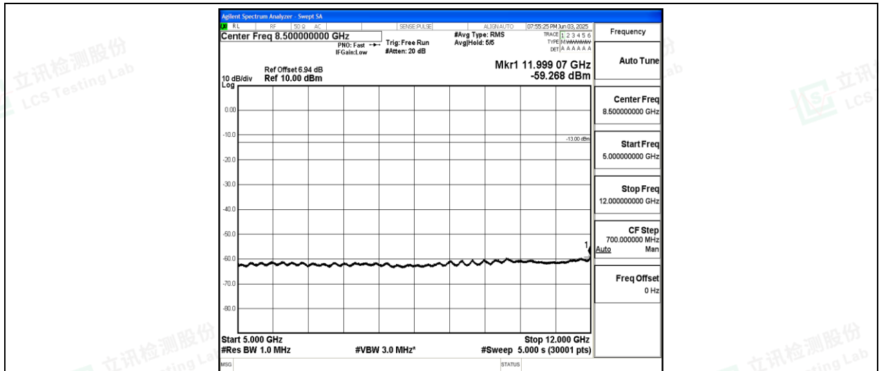
Band26-3MHz-16QAM-26805-1-0-Low-5000-12000--59.27-PASS
