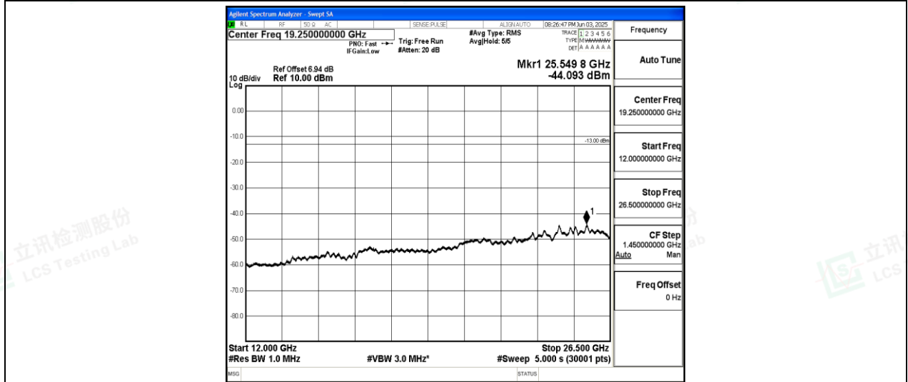
Band26-5MHz-16QAM-26815-1-0-Low-12000-26500--44.09-PASS
