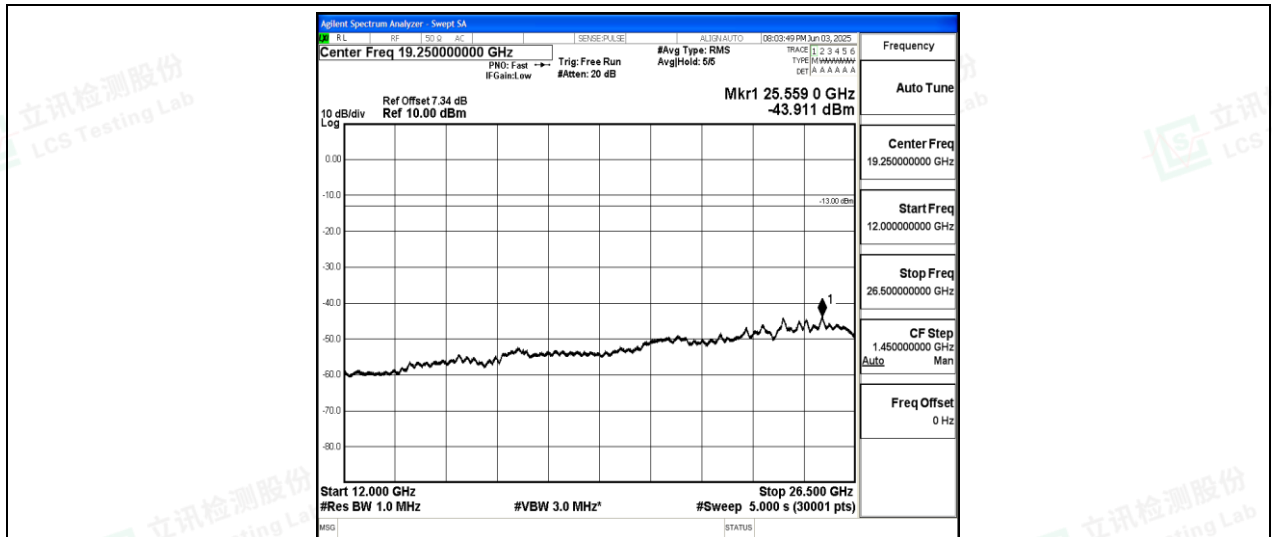
Band26-3MHz-16QAM-27025-1-0-High-12000-26500--43.91-PASS
