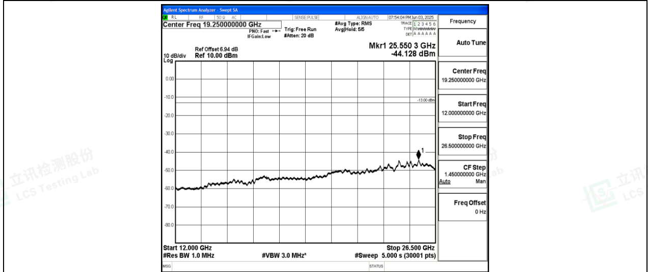
Band26-3MHz-QPSK-26805-1-0-Low-12000-26500--44.13-PASS
