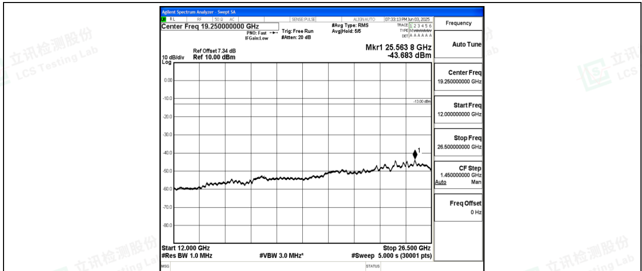
Band26-1.4MHz-16QAM-27033-1-0-High-12000-26500--43.68-PASS
