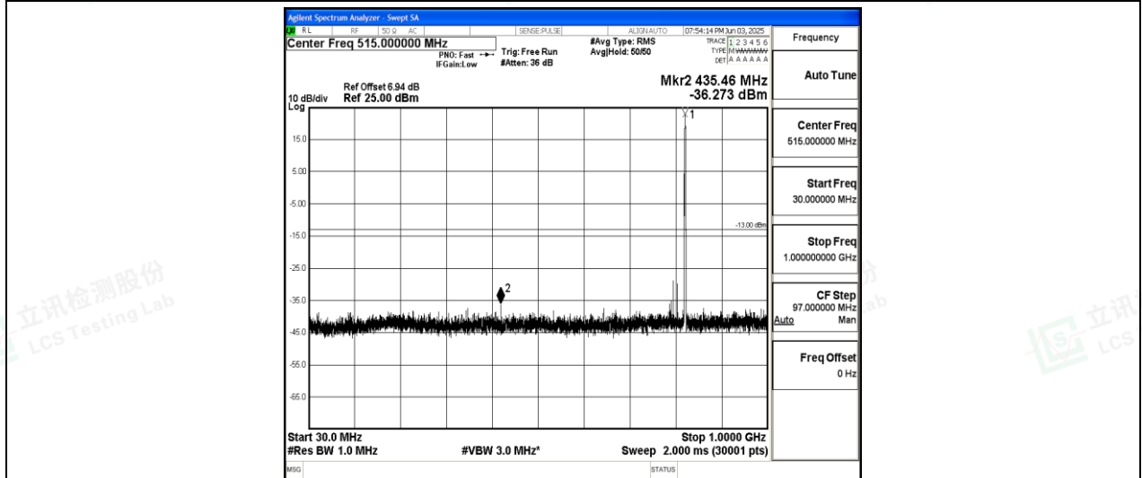
Band26-3MHz-16QAM-26805-1-0-Low-30-1000--36.27-PASS
