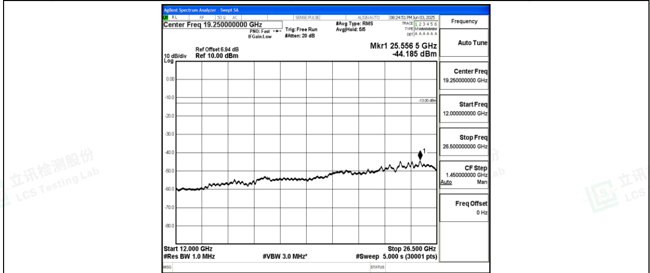
Band26-5MHz-QPSK-26815-1-0-Low-12000-26500--44.19-PASS
