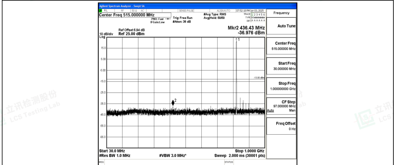
Band26-3MHz-QPSK-26805-1-0-Low-30-1000--36.98-PASS
