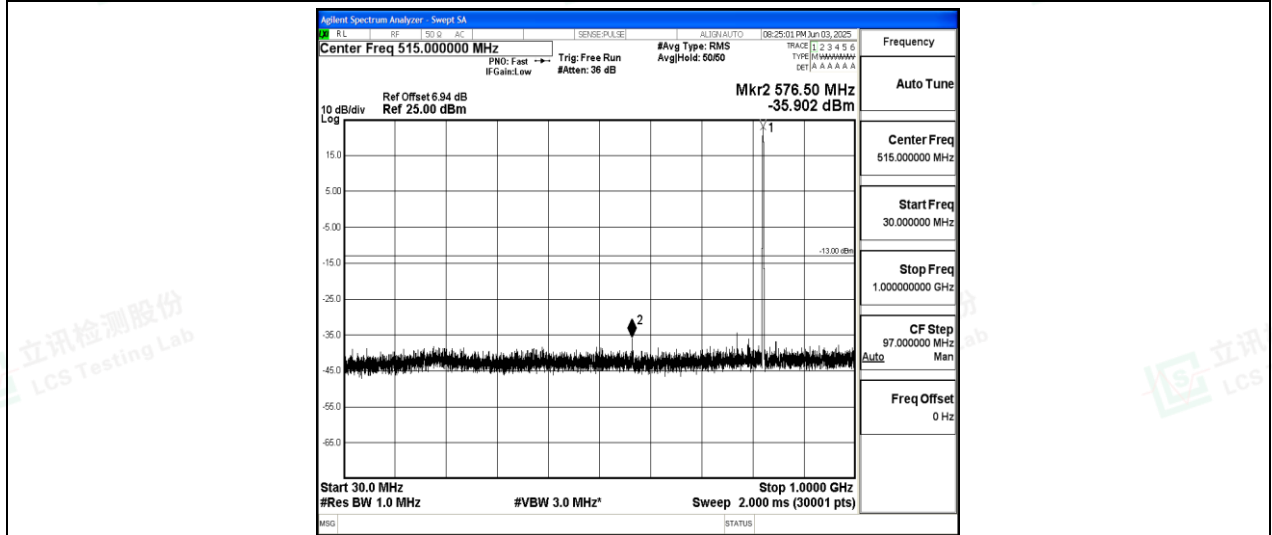
Band26-5MHz-16QAM-26815-1-0-Low-30-1000--35.9-PASS
