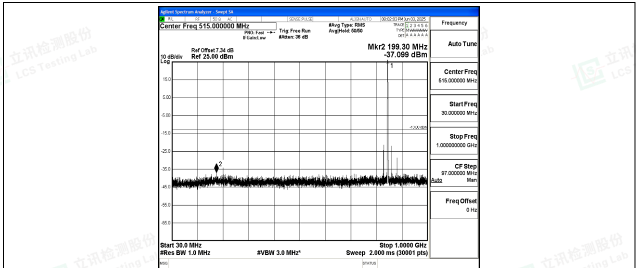
Band26-3MHz-16QAM-27025-1-0-High-30-1000--37.1-PASS
