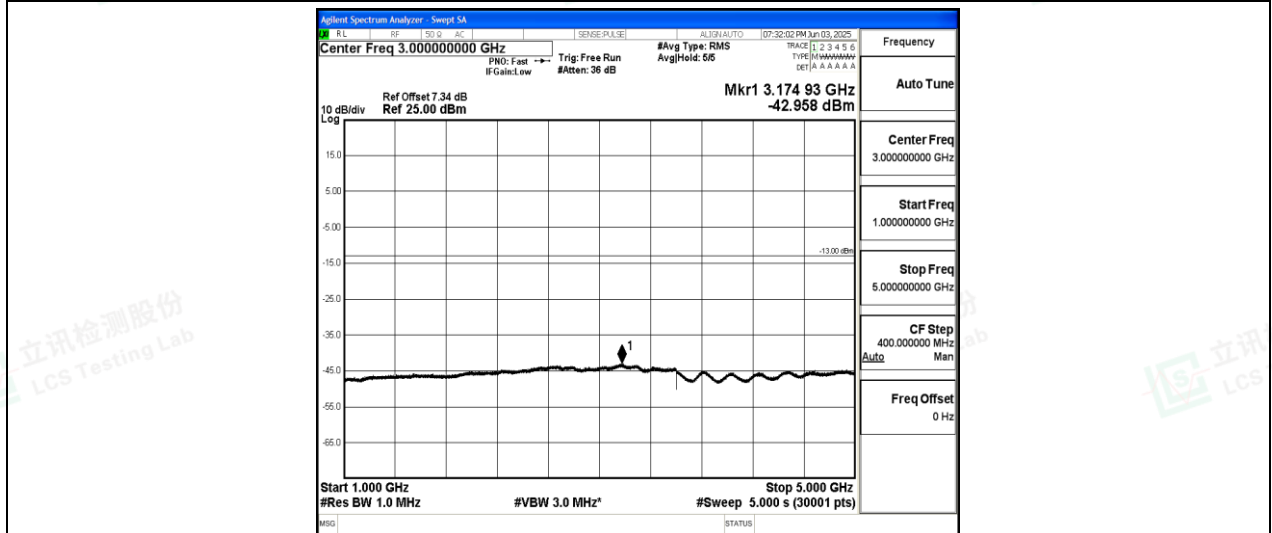
Band26-1.4MHz-16QAM-27033-1-0-High-1000-5000--42.96-PASS
