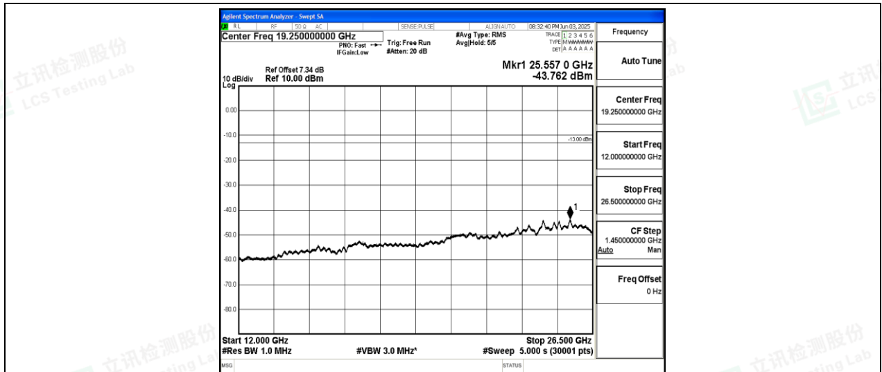
Band26-5MHz-QPSK-27015-1-0-High-12000-26500--43.76-PASS
