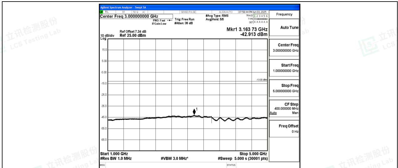
Band26-3MHz-16QAM-26915-1-0-Low-1000-5000--42.91-PASS
