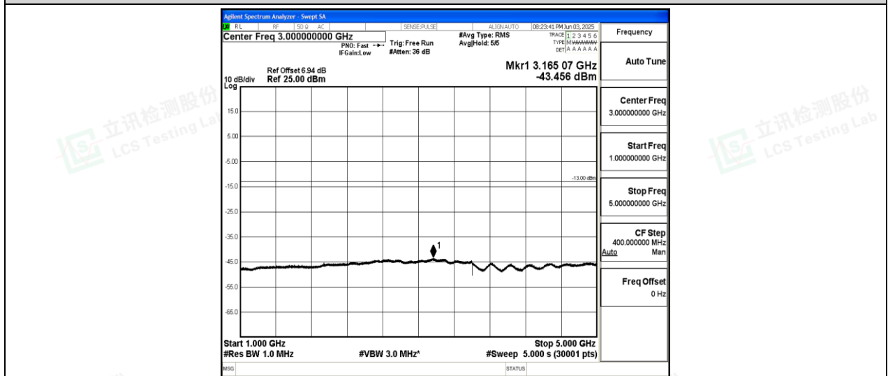
Band26-5MHz-QPSK-26815-1-0-Low-1000-5000--43.46-PASS
