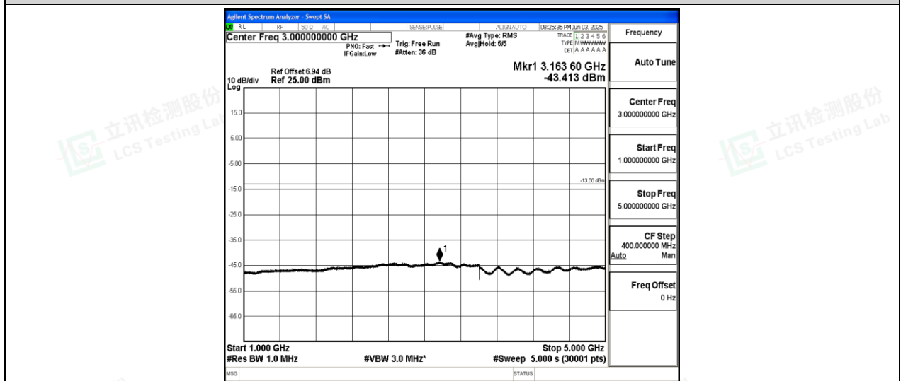
Band26-5MHz-16QAM-26815-1-0-Low-1000-5000--43.41-PASS
