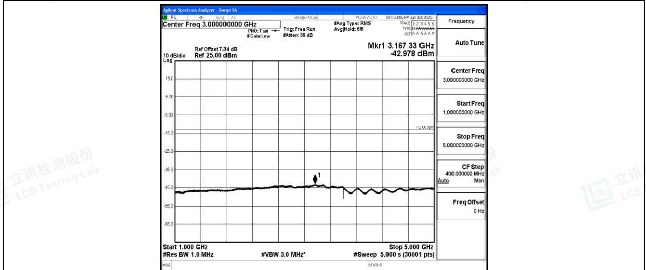
Band26-1.4MHz-QPSK-27033-1-0-High-1000-5000--42.98-PASS
