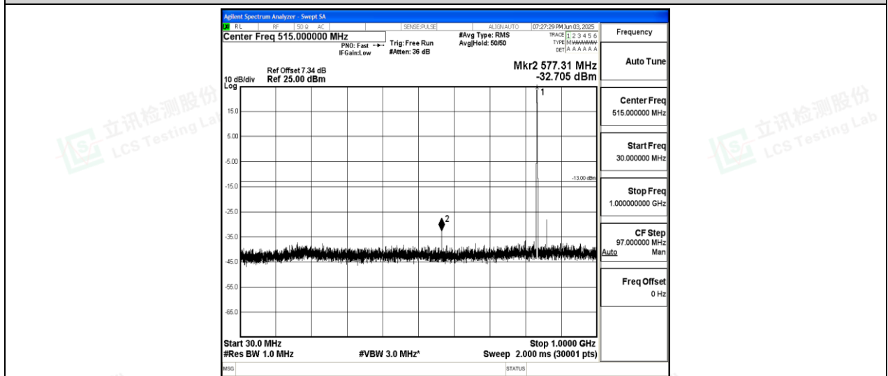
Band26-1.4MHz-16QAM-26915-1-0-Low-30-1000--32.71-PASS
