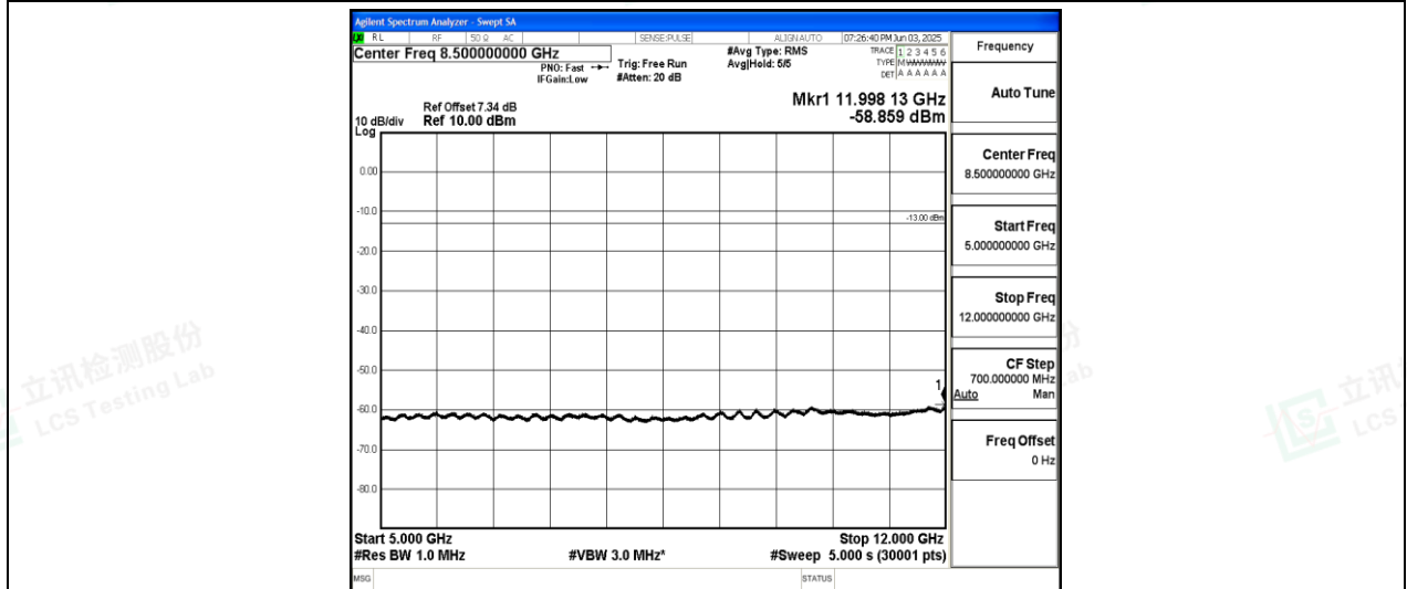
Band26-1.4MHz-QPSK-26915-1-0-Low-5000-12000--58.86-PASS
