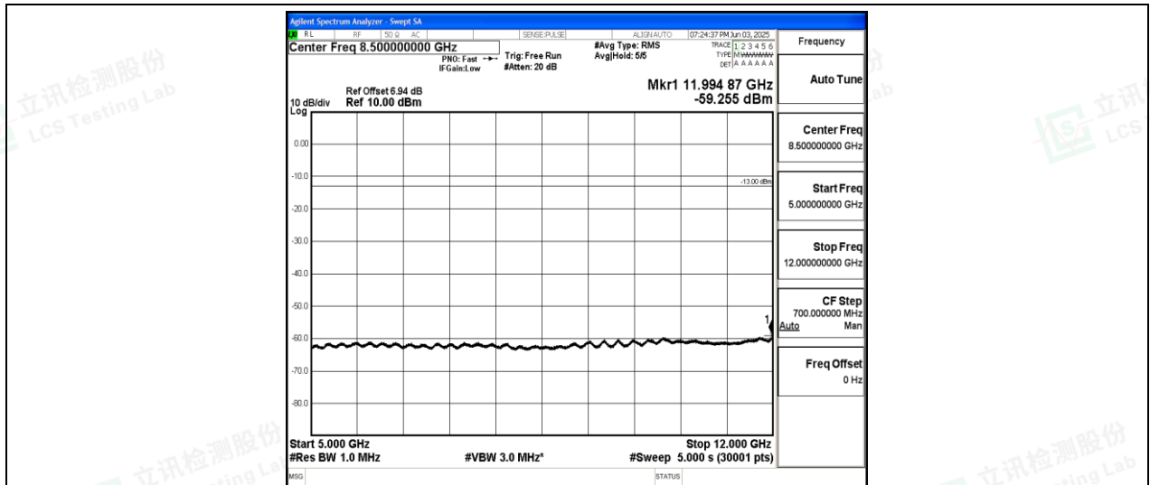
Band26-1.4MHz-16QAM-26797-1-0-Low-5000-12000--59.26-PASS
