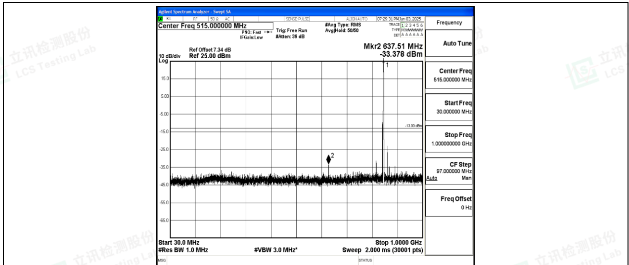
Band26-1.4MHz-QPSK-27033-1-0-High-30-1000--33.38-PASS
