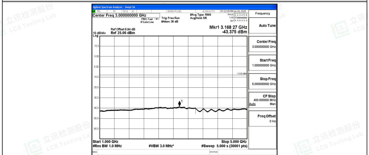
Band26-1.4MHz-QPSK-26797-1-0-Low-1000-5000--43.38-PASS
