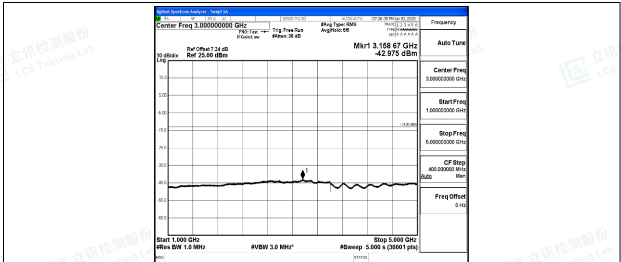
Band26-1.4MHz-QPSK-26915-1-0-Low-1000-5000--42.98-PASS
