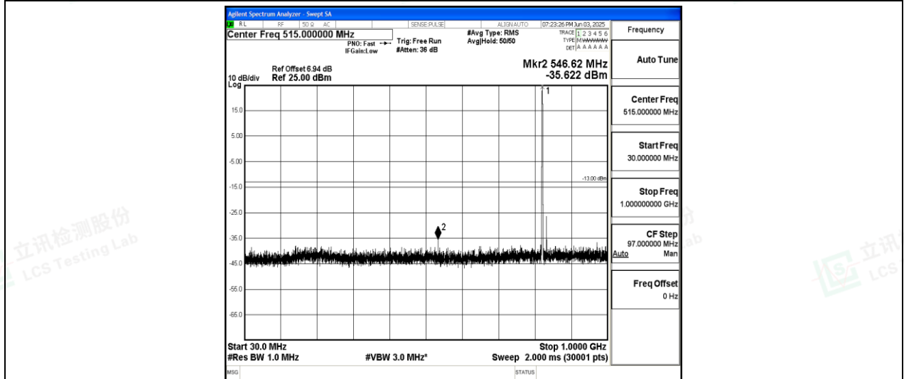
Band26-1.4MHz-16QAM-26797-1-0-Low-30-1000--35.62-PASS
