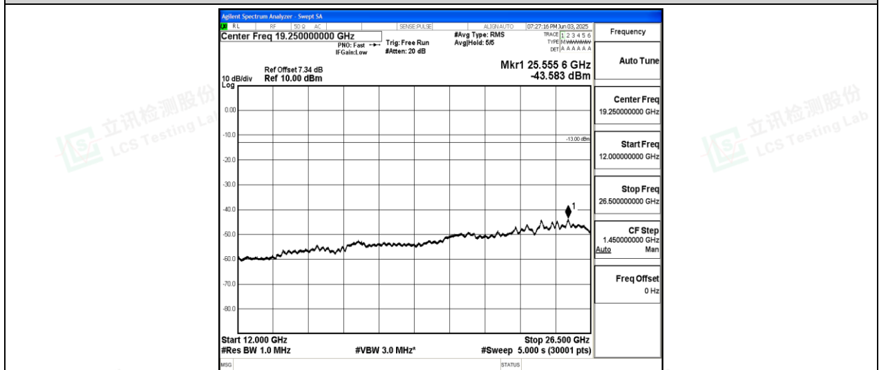
Band26-1.4MHz-QPSK-26915-1-0-Low-12000-26500--43.58-PASS
