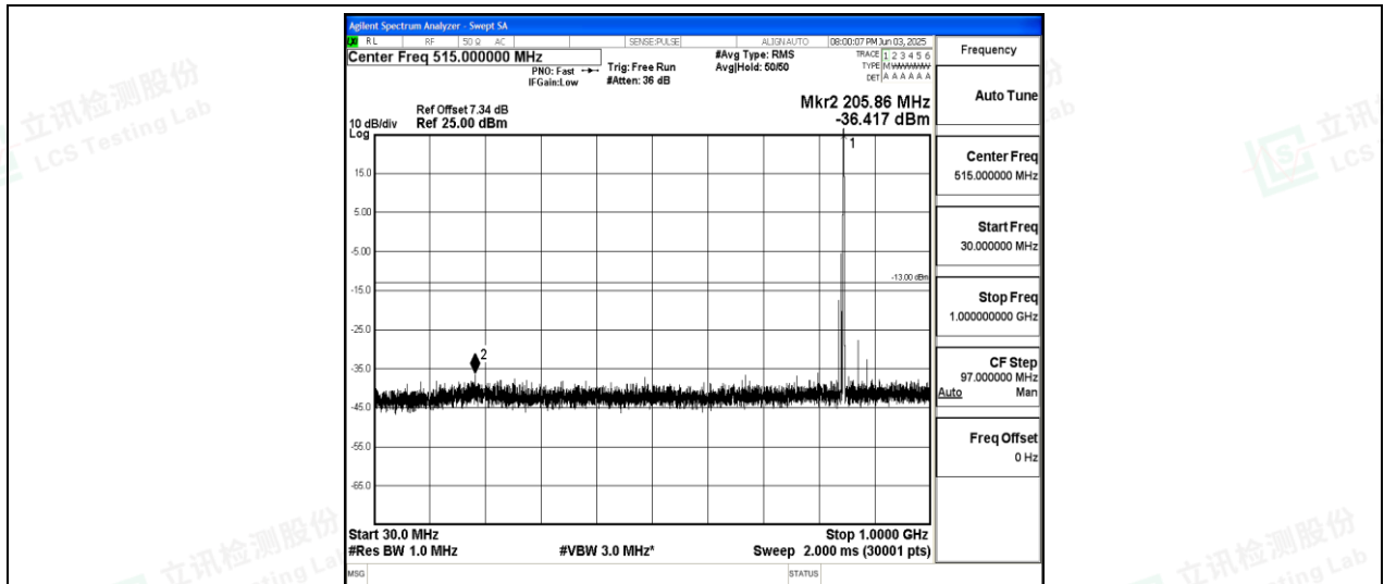
Band26-3MHz-QPSK-27025-1-0-High-30-1000--36.42-PASS
