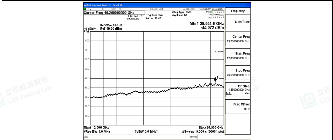
Band26-1.4MHz-16QAM-26797-1-0-Low-12000-26500--44.07-PASS
