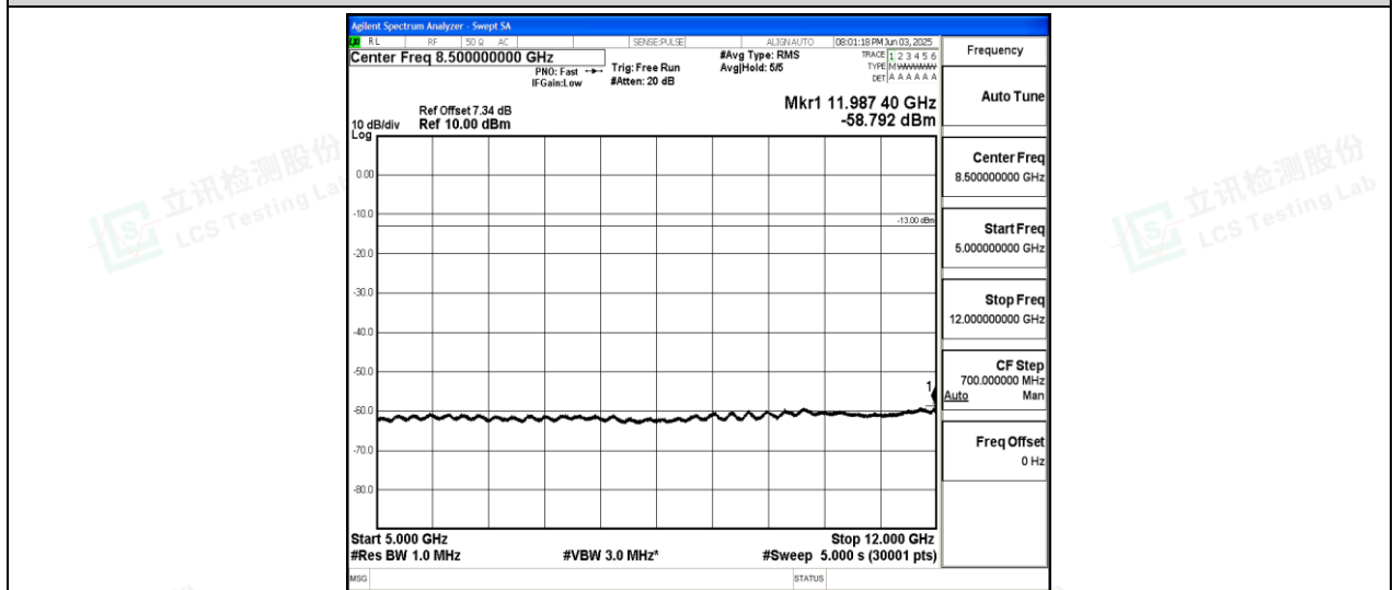
Band26-3MHz-QPSK-27025-1-0-High-5000-12000--58.79-PASS
