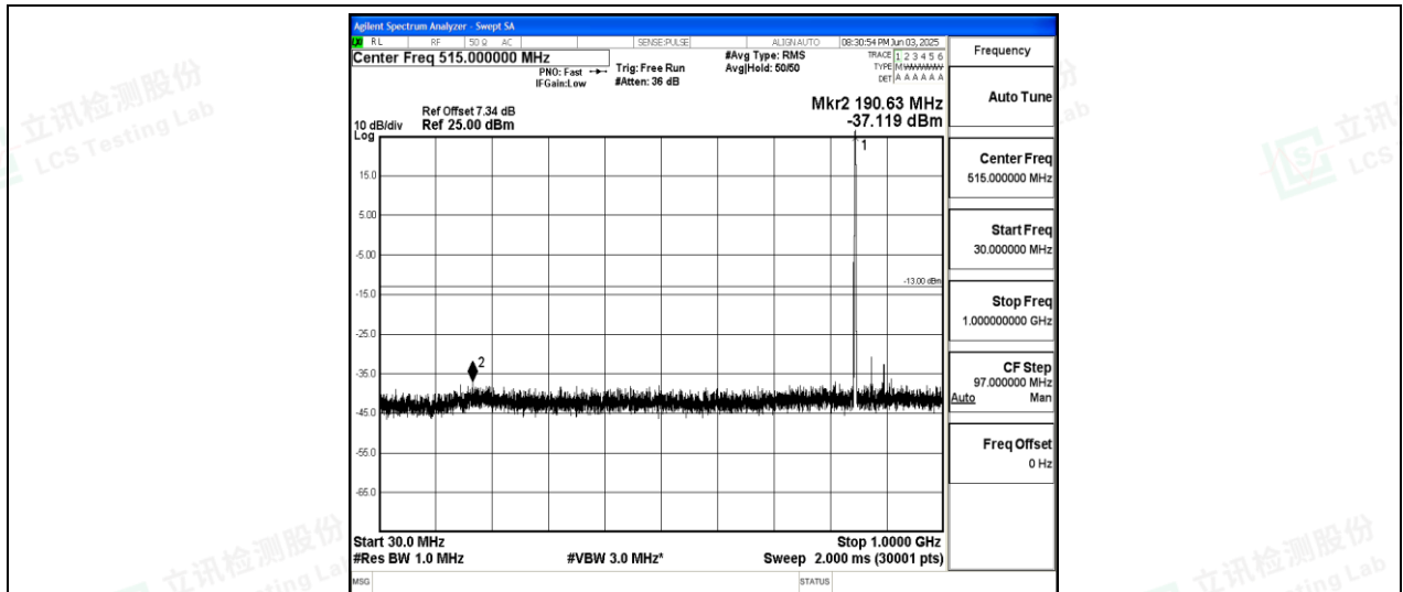
Band26-5MHz-QPSK-27015-1-0-High-30-1000--37.12-PASS
