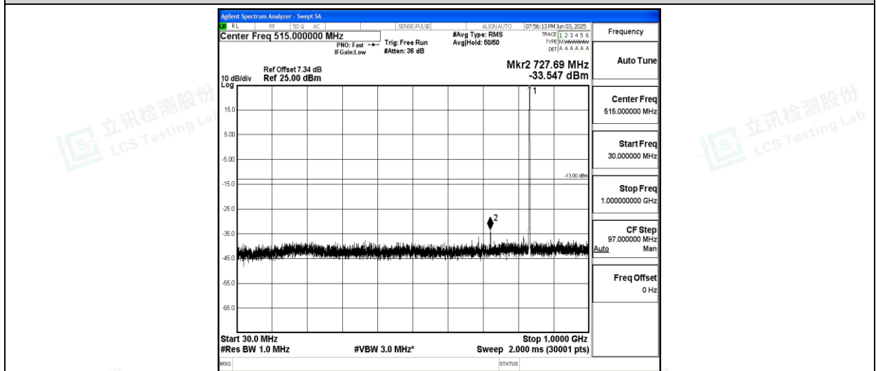
Band26-3MHz-QPSK-26915-1-0-Low-30-1000--33.55-PASS
