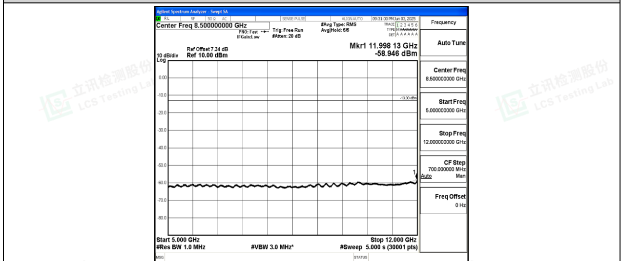
Band26-15MHz-16QAM-26965-1-0-High-5000-12000--58.95-PASS
