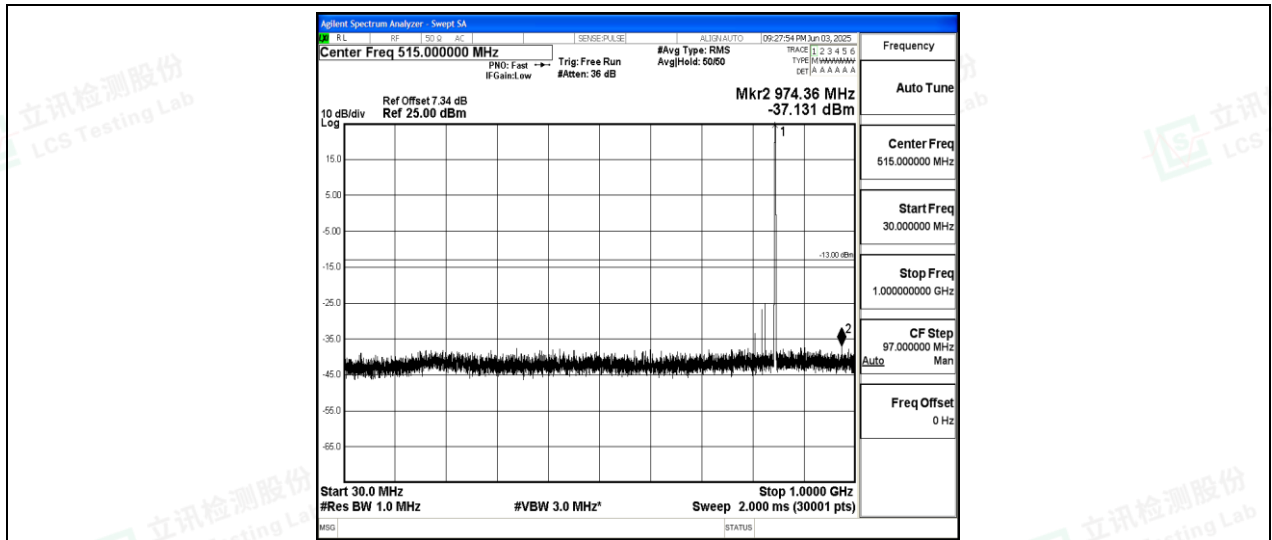
Band26-15MHz-QPSK-26965-1-0-High-30-1000--37.13-PASS
