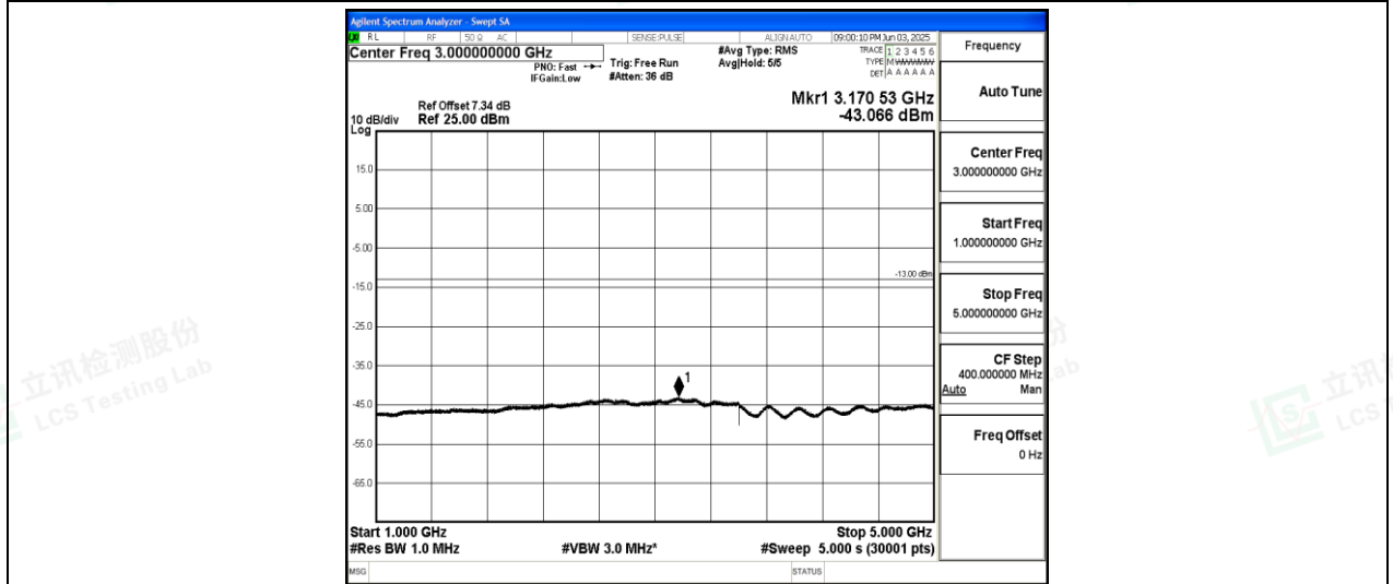
Band26-10MHz-QPSK-26990-1-0-High-1000-5000--43.07-PASS
