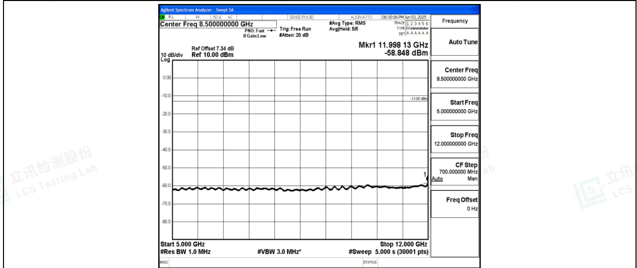
Band26-5MHz-16QAM-26915-1-0-Low-5000-12000--58.85-PASS
