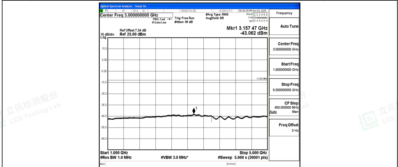
Band26-15MHz-16QAM-26965-1-0-High-1000-5000--43.06-PASS
