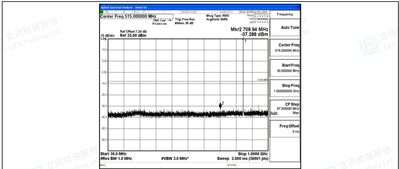
Band26-10MHz-16QAM-26990-1-0-High-30-1000--37.29-PASS
