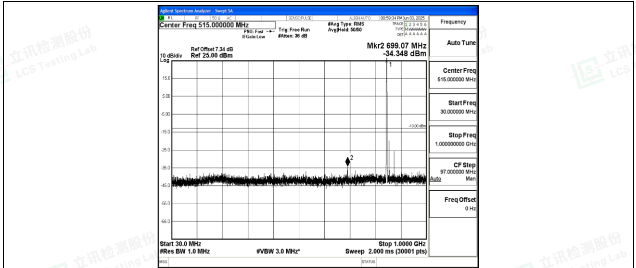
Band26-10MHz-QPSK-26990-1-0-High-30-1000--34.35-PASS
