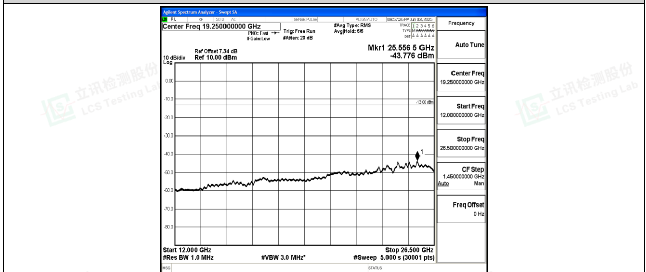
Band26-10MHz-QPSK-26915-1-0-Low-12000-26500--43.78-PASS
