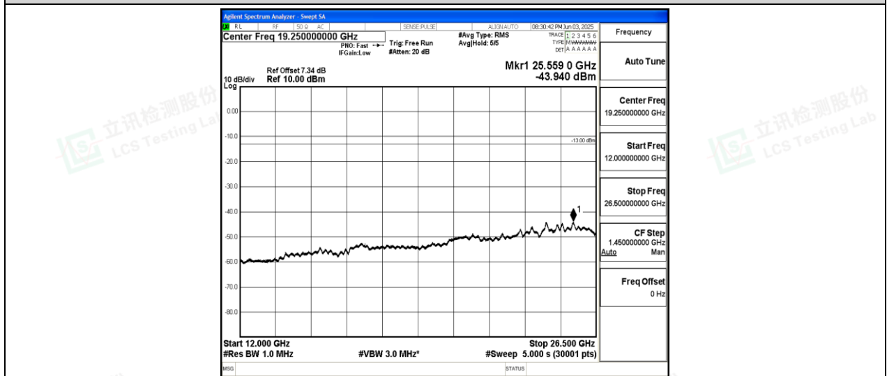
Band26-5MHz-16QAM-26915-1-0-Low-12000-26500--43.94-PASS
