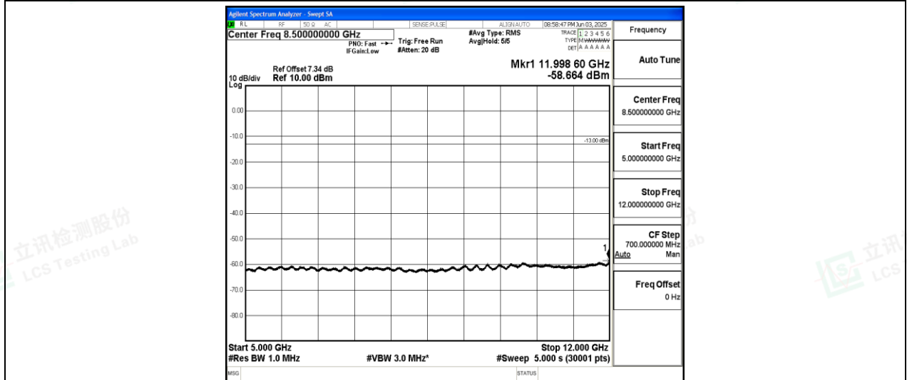
Band26-10MHz-16QAM-26915-1-0-Low-5000-12000--58.66-PASS
