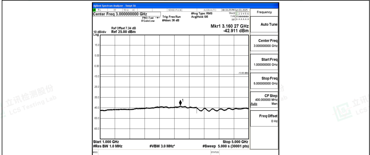
Band26-5MHz-16QAM-27015-1-0-High-1000-5000--42.91-PASS
