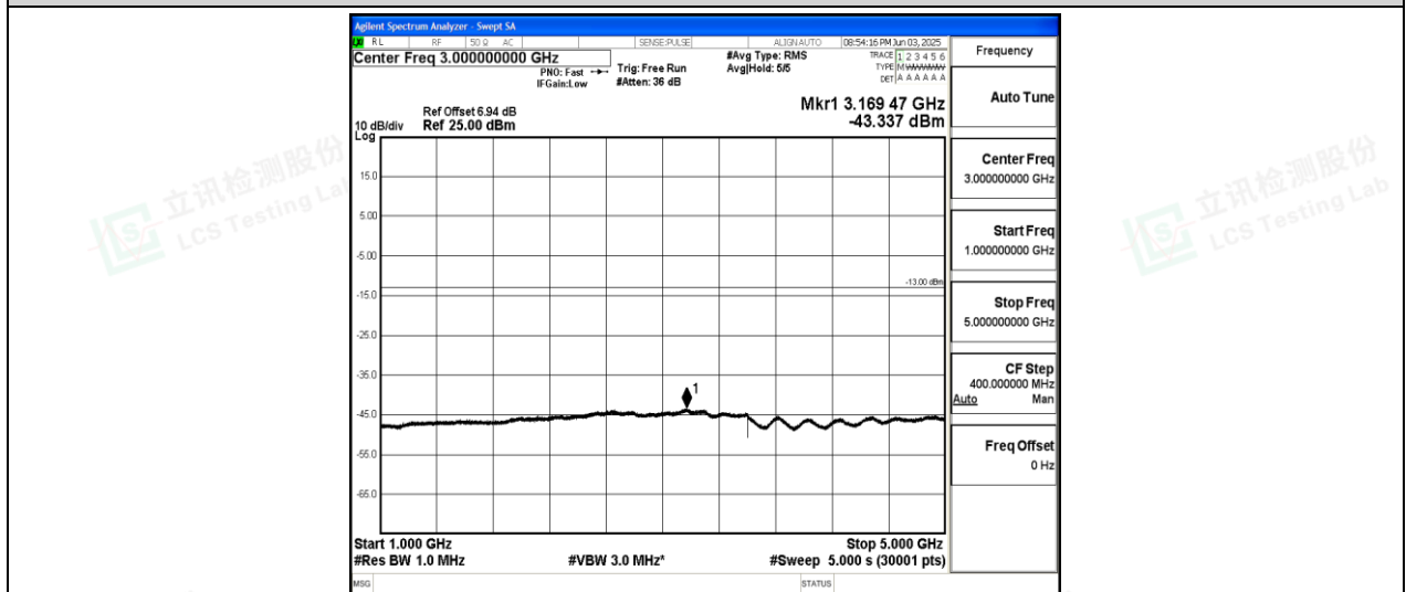
Band26-10MHz-16QAM-26840-1-0-Low-1000-5000--43.34-PASS
