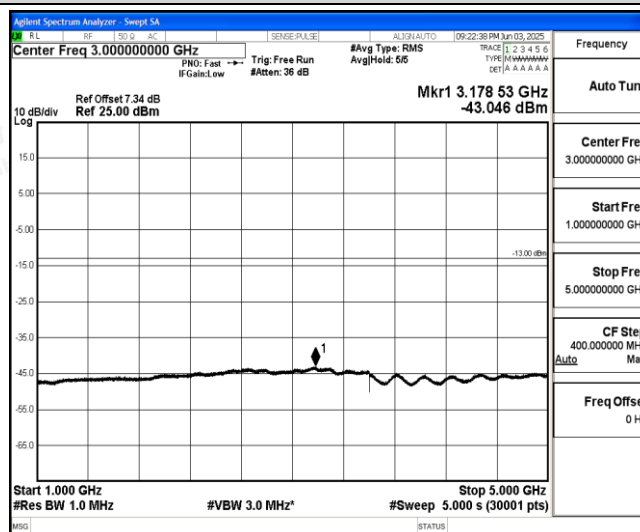
Band26-15MHz-16QAM-26865-1-0-Low-1000-5000--43.05-PASS
