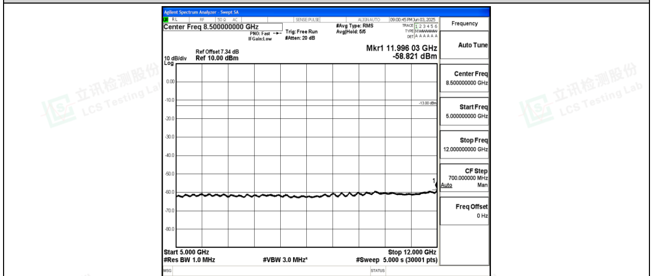
Band26-10MHz-QPSK-26990-1-0-High-5000-12000--58.82-PASS
