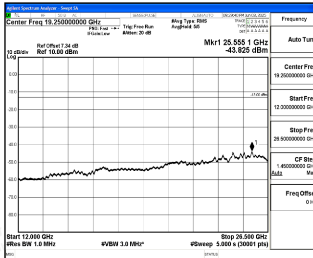
Band26-15MHz-QPSK-26965-1-0-High-12000-26500--43.83-PASS
