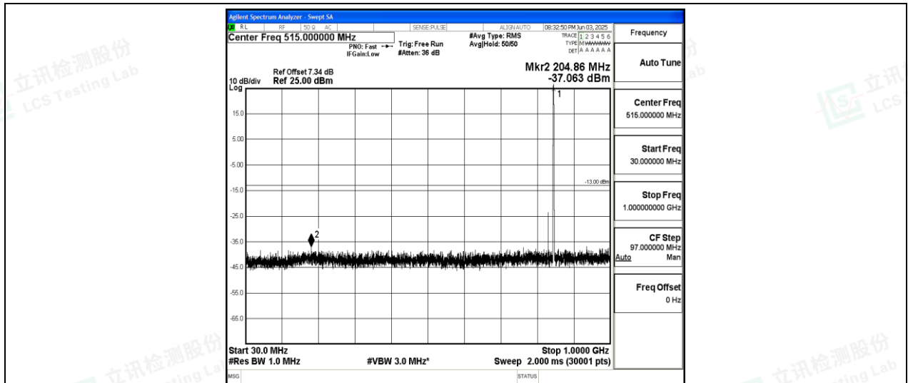
Band26-5MHz-16QAM-27015-1-0-High-30-1000--37.06-PASS
