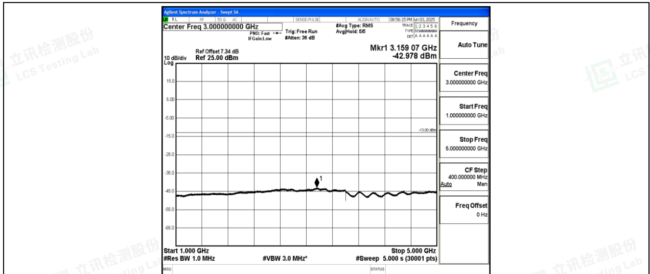
Band26-10MHz-QPSK-26915-1-0-Low-1000-5000--42.98-PASS
