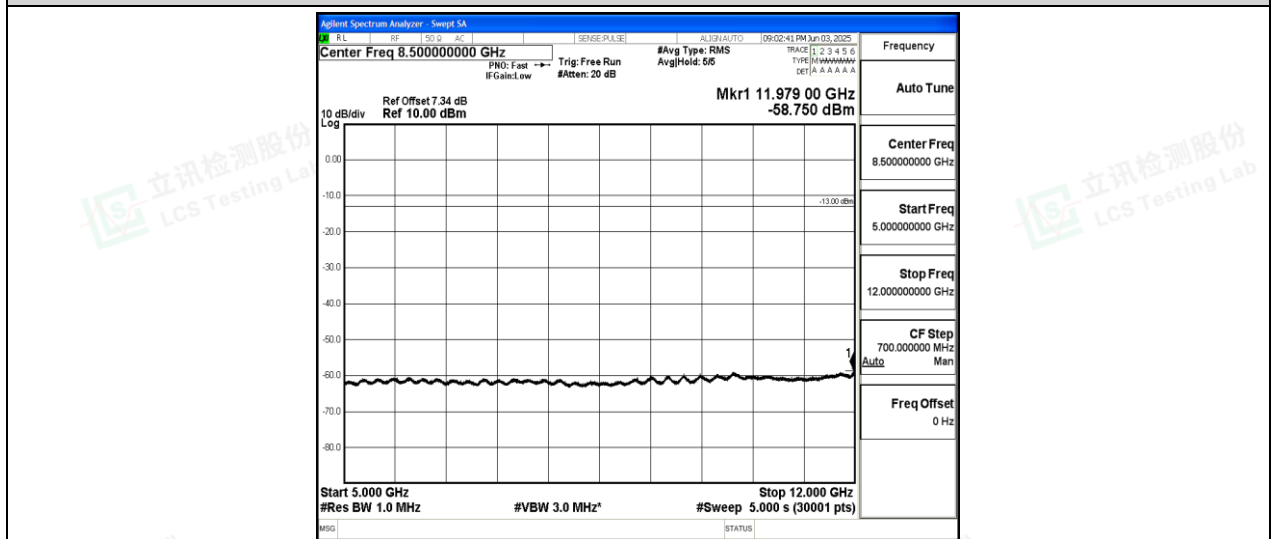
Band26-10MHz-16QAM-26990-1-0-High-5000-12000--58.75-PASS
