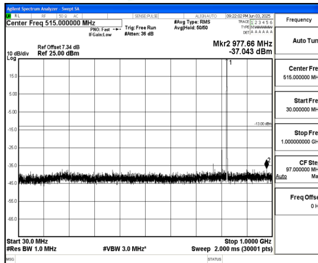
Band26-15MHz-16QAM-26865-1-0-Low-30-1000--37.04-PASS
