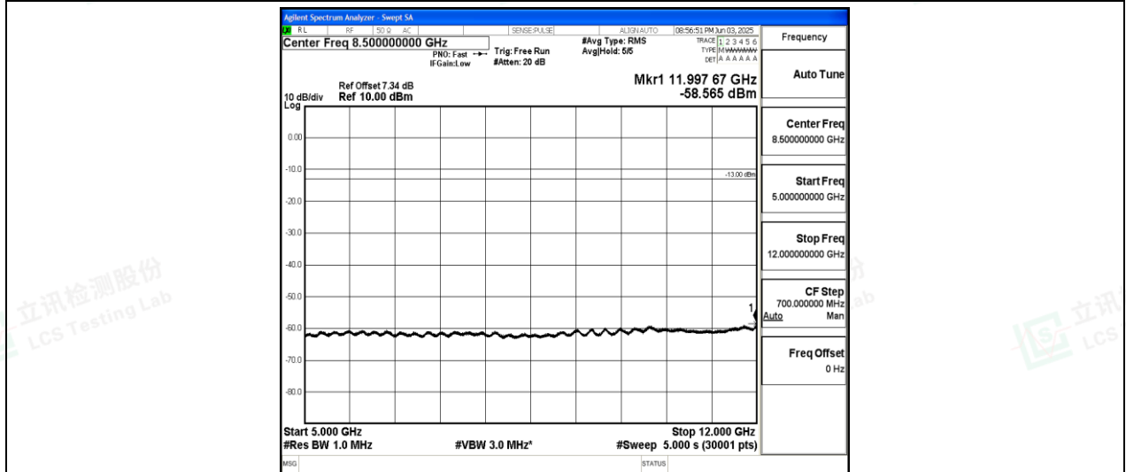
Band26-10MHz-QPSK-26915-1-0-Low-5000-12000--58.57-PASS
