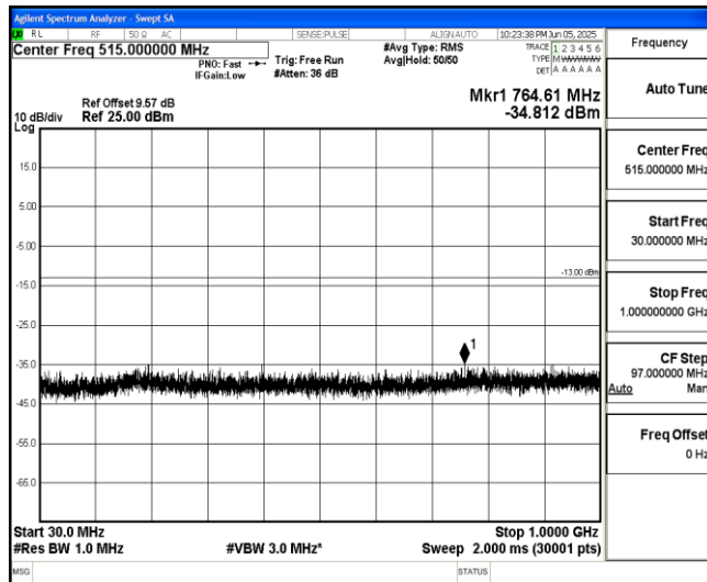
Band66-20MHz-16QAM-132572-1-0-High-30-1000--34.81-PASS
