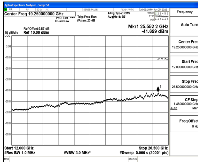
Band66-15MHz-16QAM-132597-1-0-High-12000-26500--41.7-PASS
