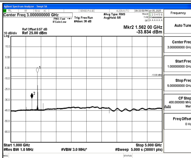
Band66-10MHz-QPSK-132022-1-0-Low-1000-5000--33.83-PASS
