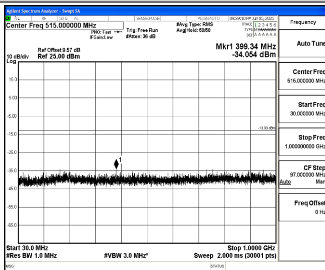
Band66-10MHz-16QAM-132322-1-0-Low-30-1000--34.05-PASS
