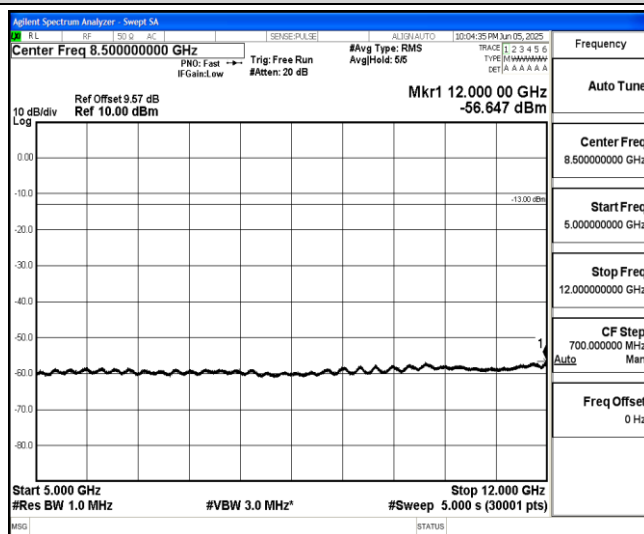
Band66-15MHz-16QAM-132597-1-0-High-5000-12000--56.65-PASS
