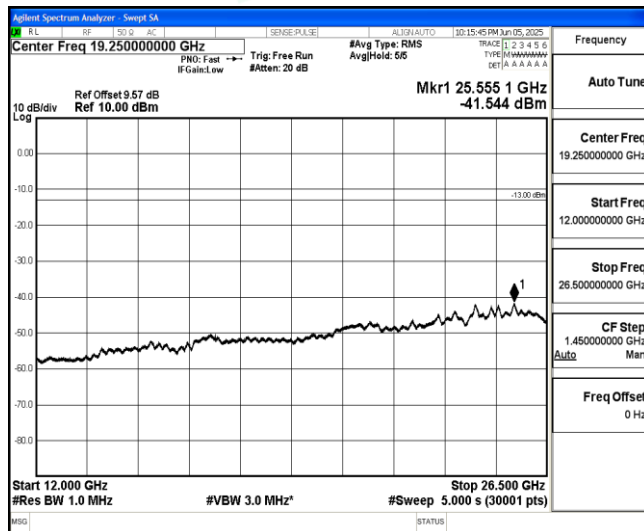
Band66-20MHz-QPSK-132072-1-0-Low-12000-26500--41.54-PASS
