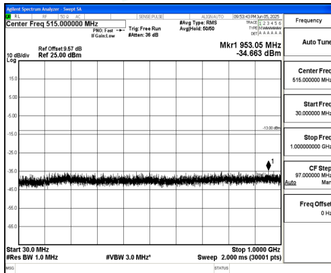
Band66-15MHz-QPSK-132047-1-0-Low-30-1000--34.66-PASS
