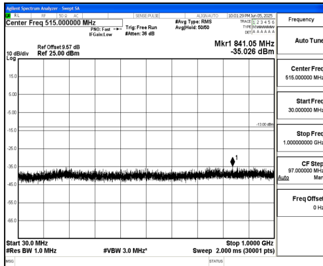
Band66-15MHz-QPSK-132597-1-0-High-30-1000--35.03-PASS
