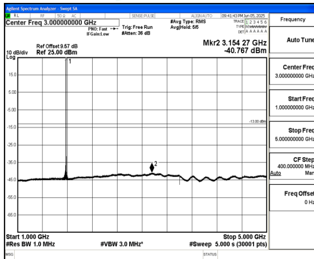
Band66-10MHz-QPSK-132622-1-0-High-1000-5000--40.77-PASS
