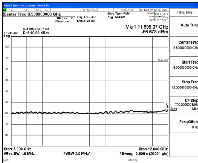
Band66-10MHz-16QAM-132322-1-0-Low-5000-12000--56.68-PASS
