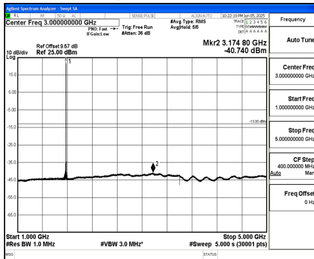
Band66-20MHz-QPSK-132572-1-0-High-1000-5000--40.74-PASS
