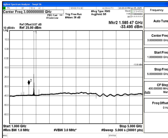
Band66-20MHz-16QAM-132322-1-0-Low-1000-5000--33.5-PASS
