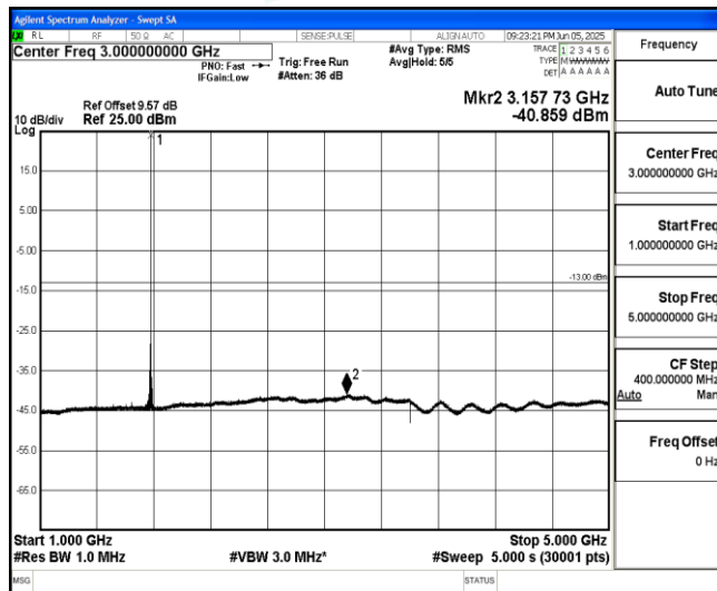
Band66-5MHz-16QAM-132647-1-0-High-1000-5000--40.86-PASS
