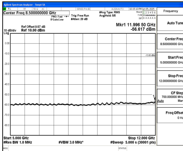
Band66-20MHz-QPSK-132072-1-0-Low-5000-12000--56.62-PASS
