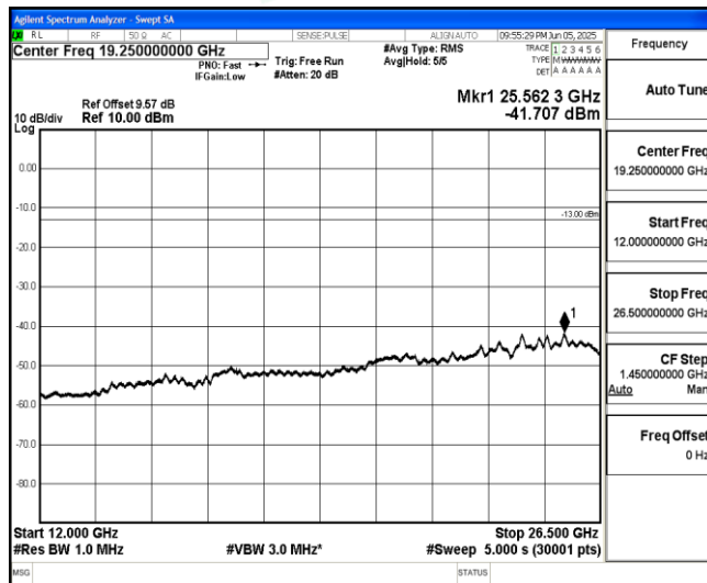
Band66-15MHz-QPSK-132047-1-0-Low-12000-26500--41.71-PASS
