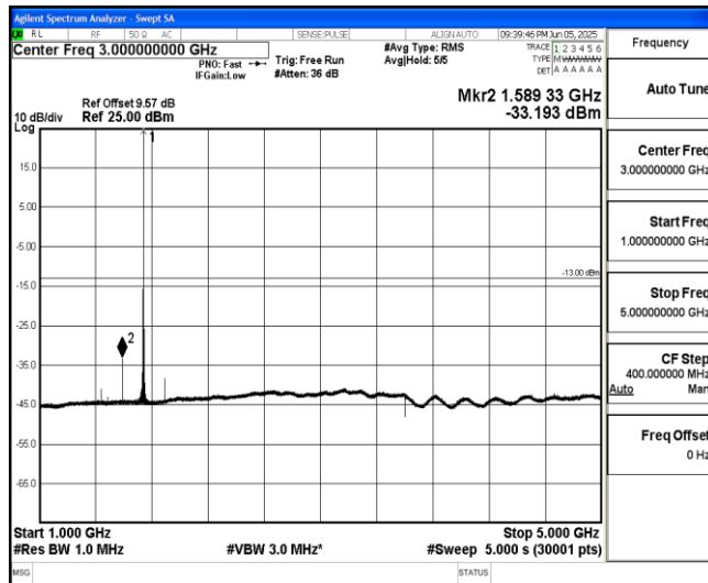
Band66-10MHz-16QAM-132322-1-0-Low-1000-5000--33.19-PASS
