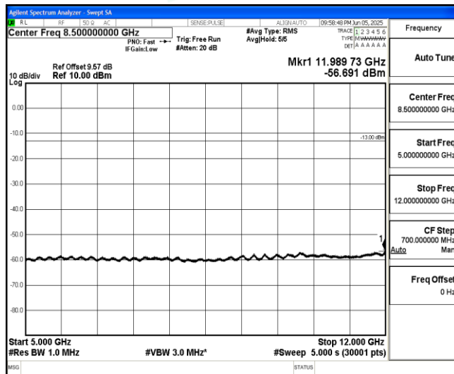
Band66-15MHz-QPSK-132322-1-0-Low-5000-12000--56.69-PASS
