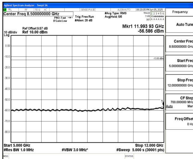
Band66-5MHz-16QAM-132322-1-0-Low-5000-12000--56.59-PASS
