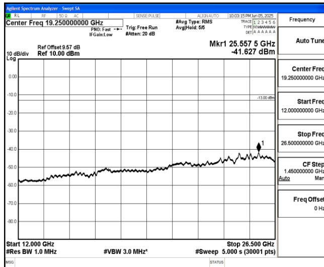
Band66-15MHz-QPSK-132597-1-0-High-12000-26500--41.63-PASS
