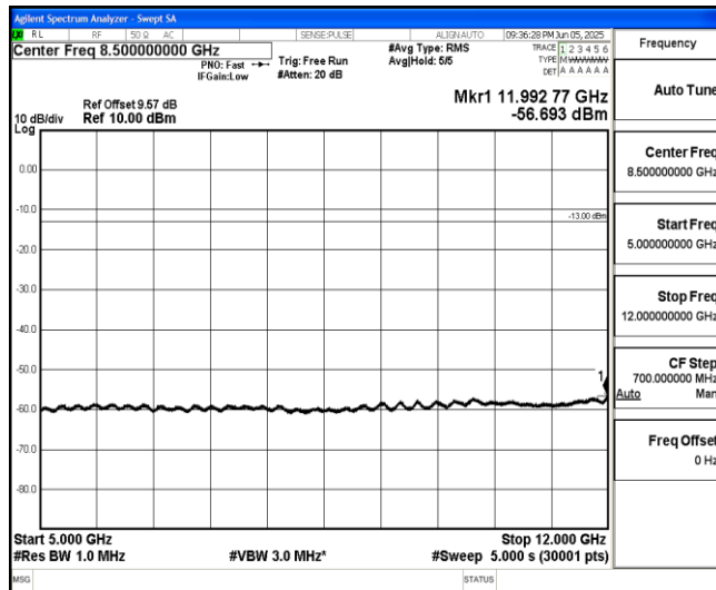
Band66-10MHz-16QAM-132022-1-0-Low-5000-12000--56.69-PASS
