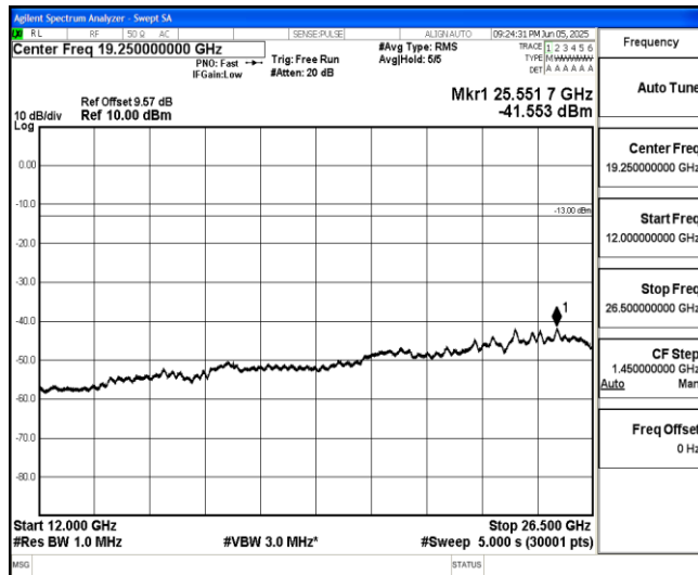
Band66-5MHz-16QAM-132647-1-0-High-12000-26500--41.55-PASS
