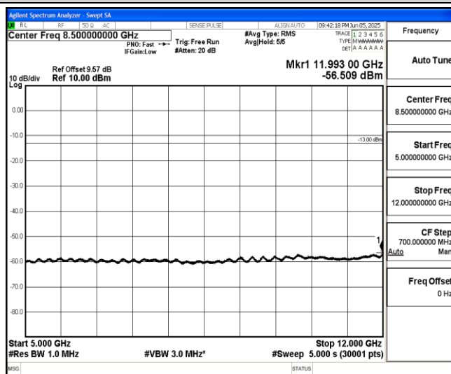
Band66-10MHz-QPSK-132622-1-0-High-5000-12000--56.51-PASS
