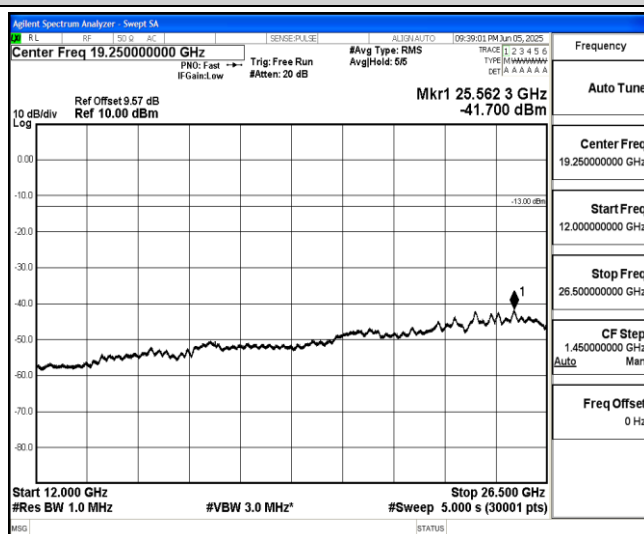
Band66-10MHz-QPSK-132322-1-0-Low-12000-26500--41.7-PASS
