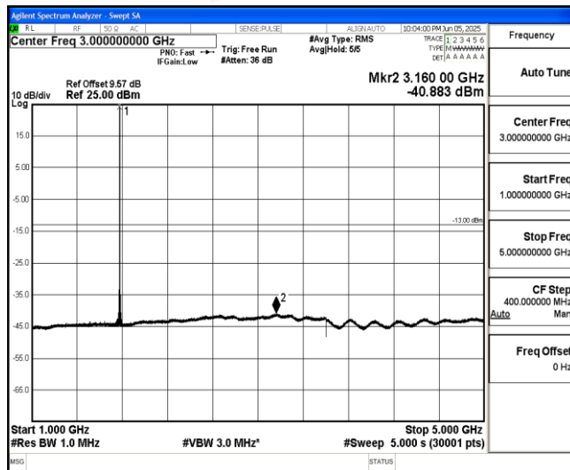
Band66-15MHz-16QAM-132597-1-0-High-1000-5000--40.88-PASS
