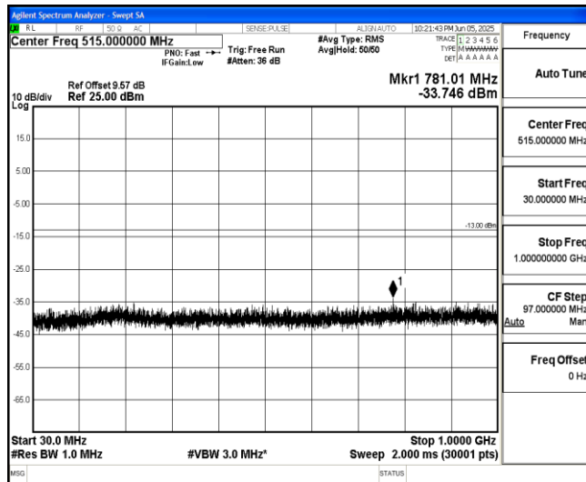
Band66-20MHz-QPSK-132572-1-0-High-30-1000--33.75-PASS
