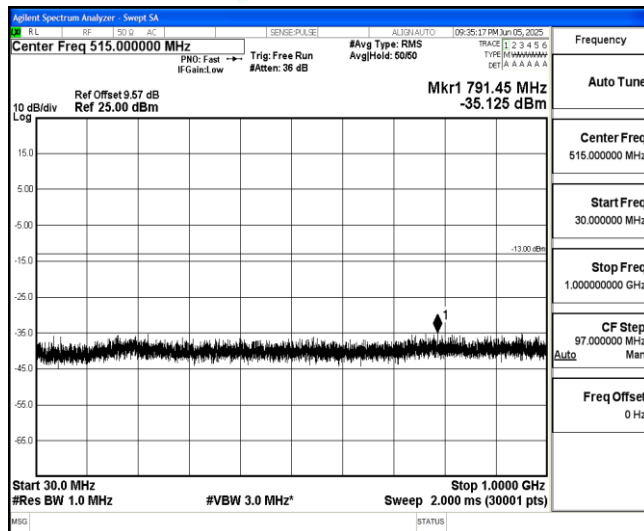
Band66-10MHz-16QAM-132022-1-0-Low-30-1000--35.13-PASS
