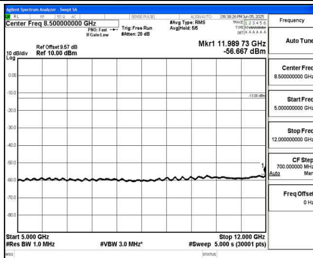
Band66-10MHz-QPSK-132322-1-0-Low-5000-12000--56.67-PASS
