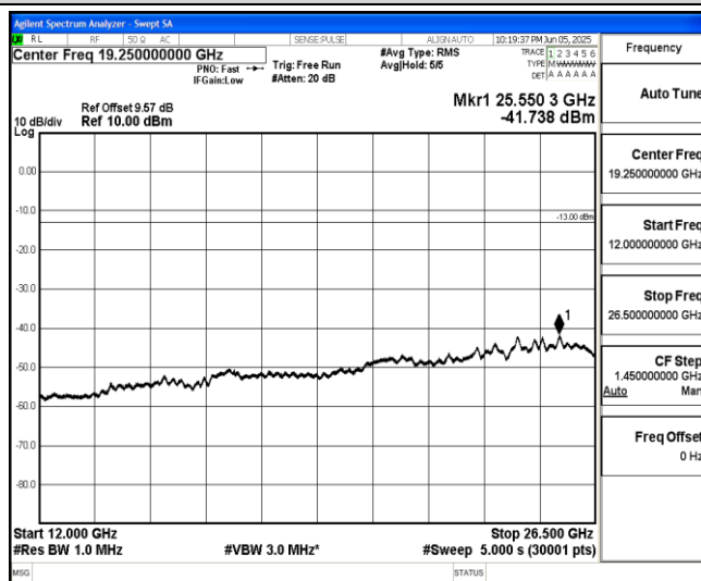
Band66-20MHz-QPSK-132322-1-0-Low-12000-26500--41.74-PASS
