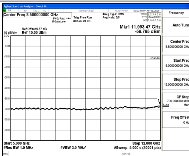
Band66-5MHz-16QAM-132647-1-0-High-5000-12000--56.77-PASS
