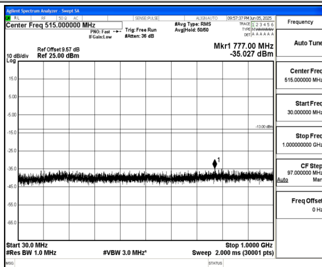
Band66-15MHz-QPSK-132322-1-0-Low-30-1000--35.03-PASS
