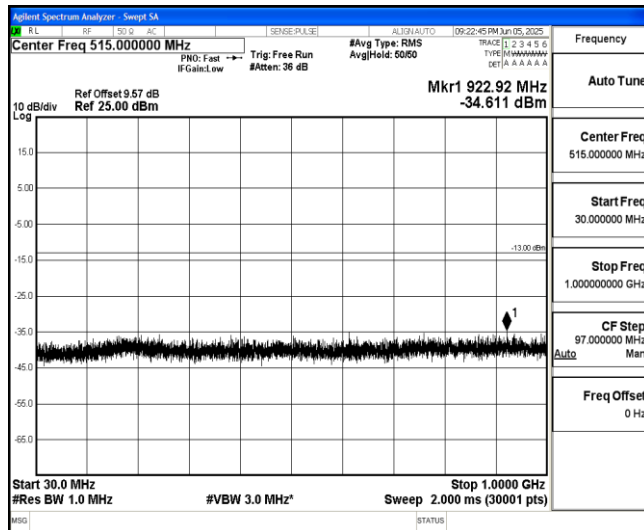
Band66-5MHz-16QAM-132647-1-0-High-30-1000--34.61-PASS
