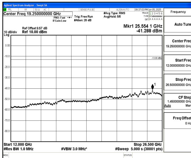
Band66-10MHz-16QAM-132022-1-0-Low-12000-26500--41.29-PASS
