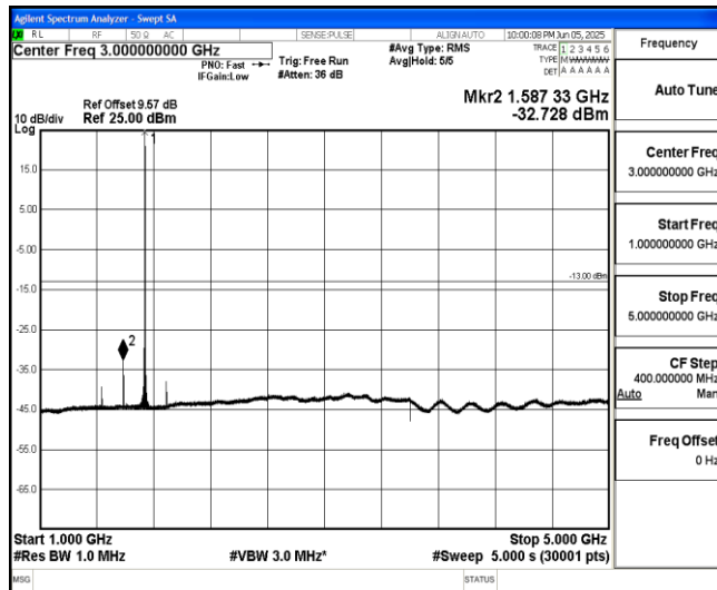
Band66-15MHz-16QAM-132322-1-0-Low-1000-5000--32.73-PASS
