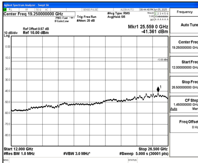
Band66-10MHz-16QAM-132622-1-0-High-12000-26500--41.36-PASS
