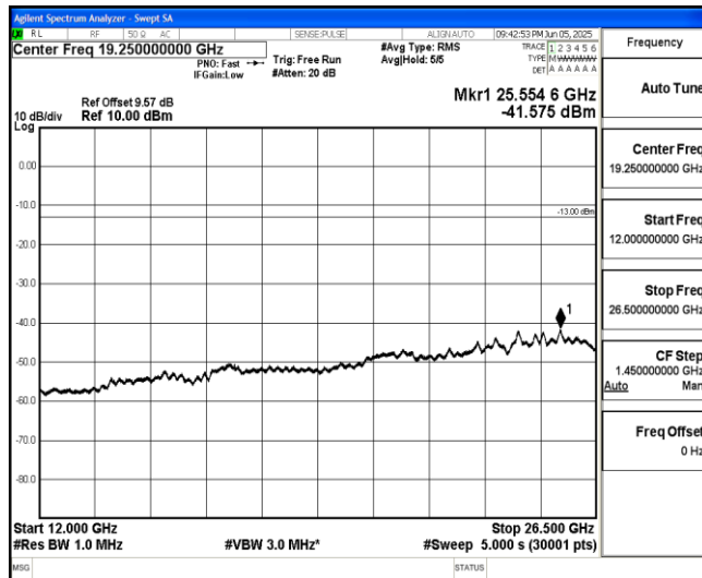
Band66-10MHz-QPSK-132622-1-0-High-12000-26500--41.58-PASS
