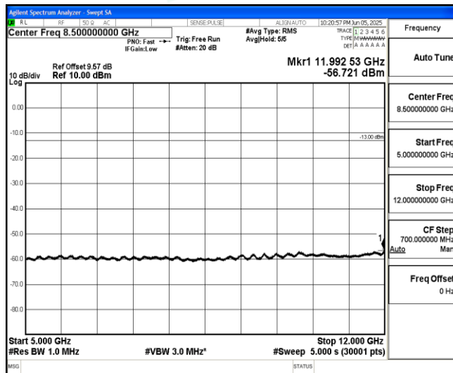
Band66-20MHz-16QAM-132322-1-0-Low-5000-12000--56.72-PASS
