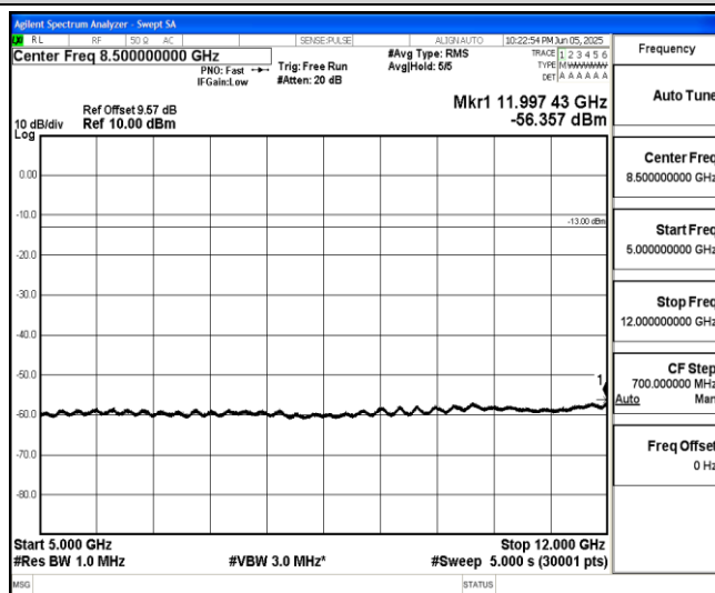
Band66-20MHz-QPSK-132572-1-0-High-5000-12000--56.36-PASS
