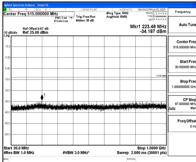
Band66-10MHz-16QAM-132622-1-0-High-30-1000--34.19-PASS
