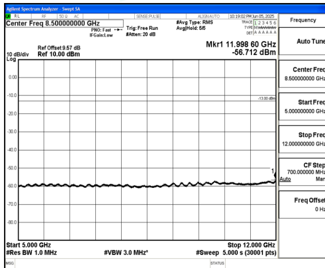
Band66-20MHz-QPSK-132322-1-0-Low-5000-12000--56.71-PASS
