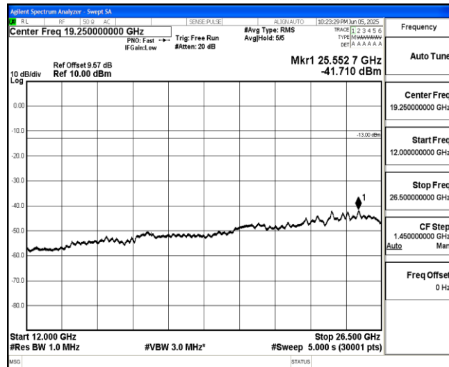
Band66-20MHz-QPSK-132572-1-0-High-12000-26500--41.71-PASS
