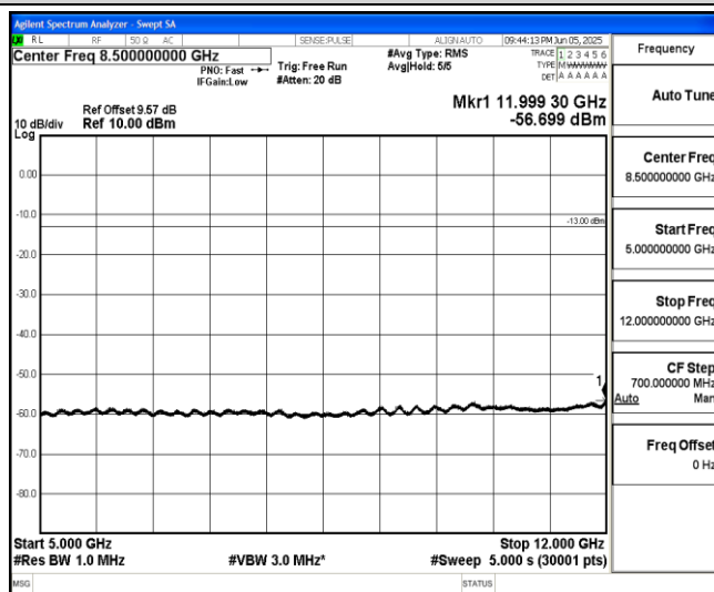
Band66-10MHz-16QAM-132622-1-0-High-5000-12000--56.7-PASS
