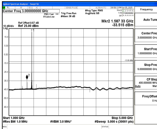
Band66-15MHz-QPSK-132322-1-0-Low-1000-5000--33.52-PASS
