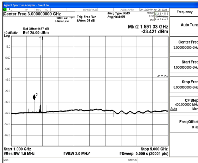
Band66-5MHz-16QAM-132322-1-0-Low-1000-5000--33.42-PASS
