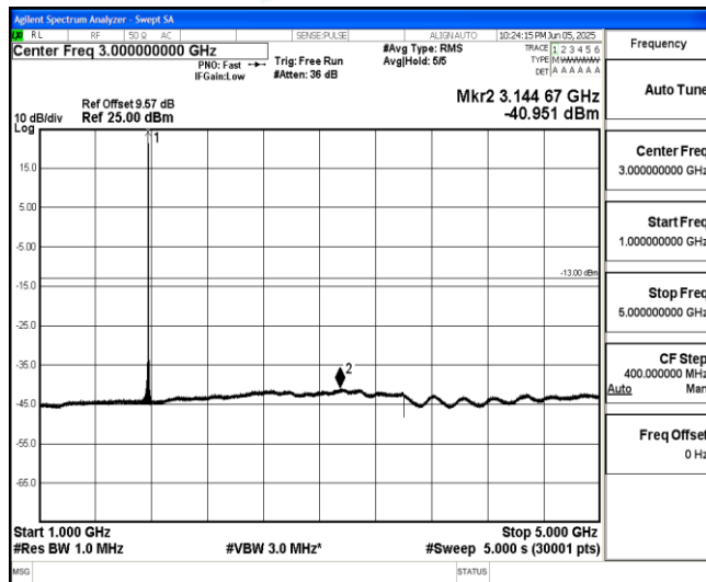
Band66-20MHz-16QAM-132572-1-0-High-1000-5000--40.95-PASS
