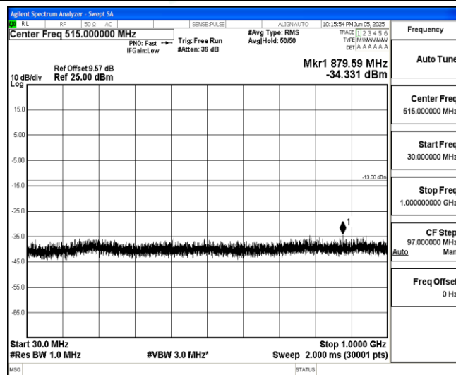
Band66-20MHz-16QAM-132072-1-0-Low-30-1000--34.33-PASS
