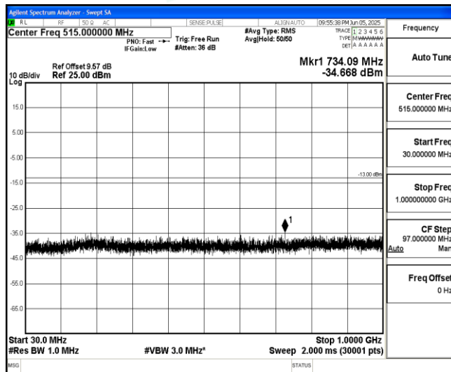
Band66-15MHz-16QAM-132047-1-0-Low-30-1000--34.67-PASS
