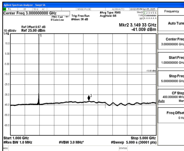
Band66-15MHz-QPSK-132597-1-0-High-1000-5000--41.01-PASS
