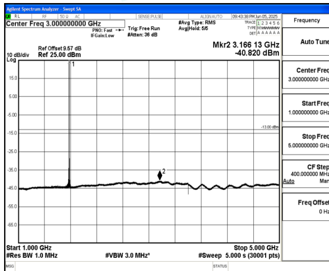
Band66-10MHz-16QAM-132622-1-0-High-1000-5000--40.82-PASS
