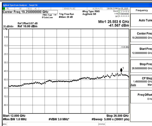
Band66-15MHz-QPSK-132322-1-0-Low-12000-26500--41.57-PASS
