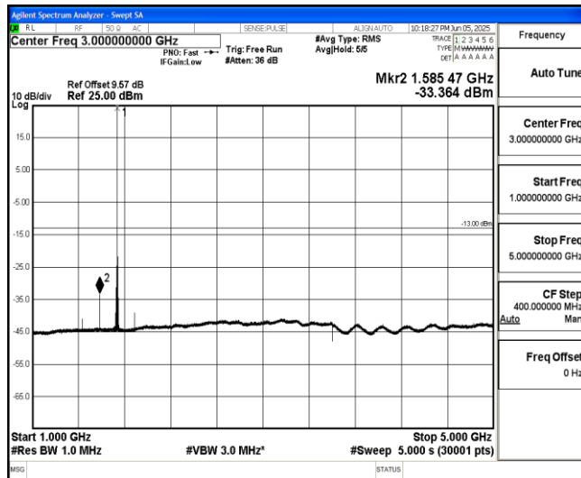
Band66-20MHz-QPSK-132322-1-0-Low-1000-5000--33.36-PASS
