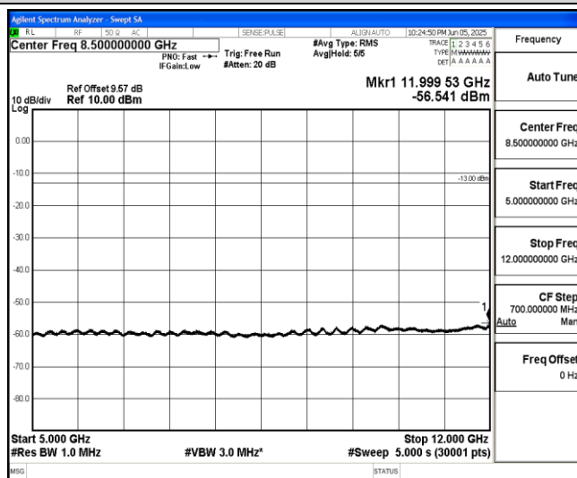
Band66-20MHz-16QAM-132572-1-0-High-5000-12000--56.54-PASS
