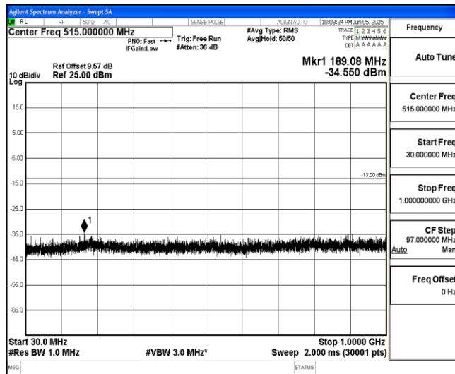
Band66-15MHz-16QAM-132597-1-0-High-30-1000--34.55-PASS
