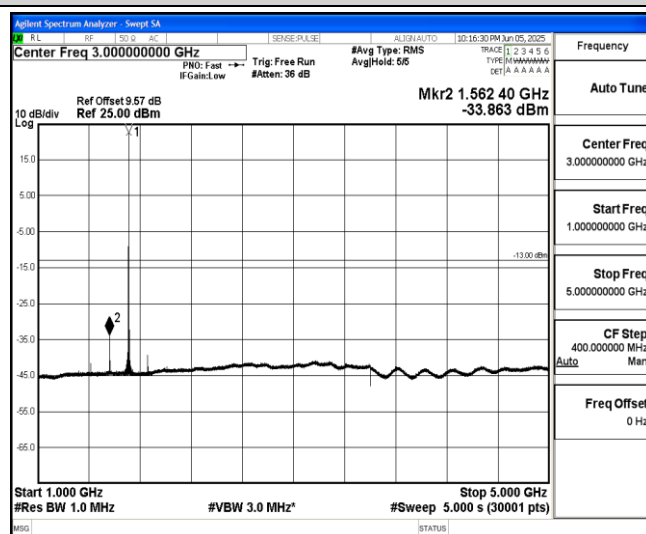
Band66-20MHz-16QAM-132072-1-0-Low-1000-5000--33.86-PASS
