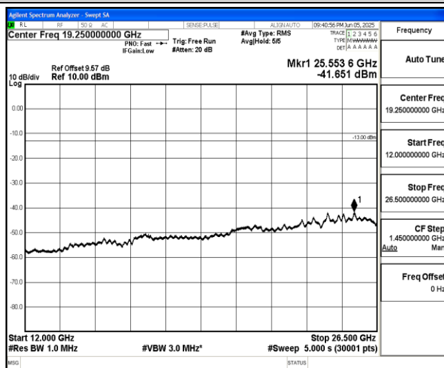
Band66-10MHz-16QAM-132322-1-0-Low-12000-26500--41.65-PASS
