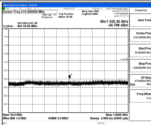
Band66-10MHz-QPSK-132322-1-0-Low-30-1000--34.8-PASS
