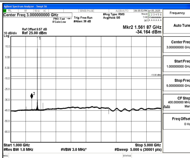
Band66-10MHz-16QAM-132022-1-0-Low-1000-5000--34.16-PASS
