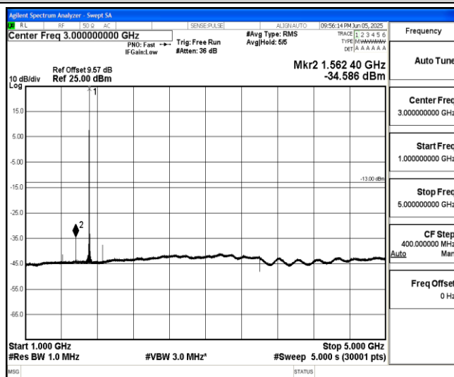
Band66-15MHz-16QAM-132047-1-0-Low-1000-5000--34.59-PASS
