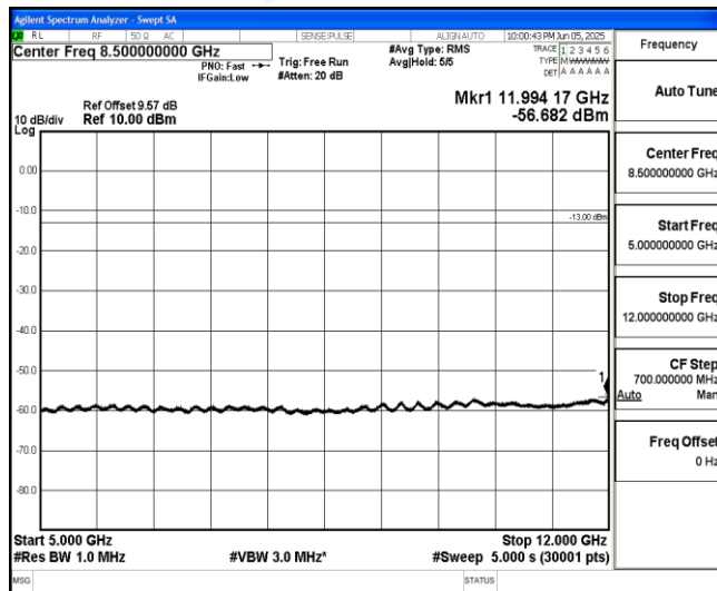
Band66-15MHz-16QAM-132322-1-0-Low-5000-12000--56.68-PASS
