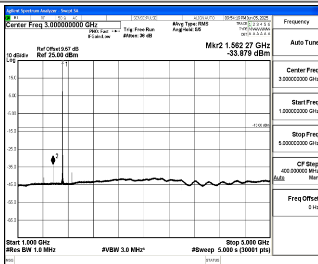
Band66-15MHz-QPSK-132047-1-0-Low-1000-5000--33.88-PASS
