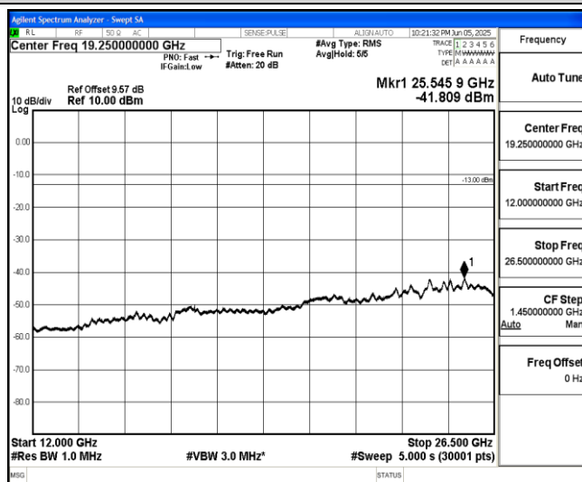
Band66-20MHz-16QAM-132322-1-0-Low-12000-26500--41.81-PASS
