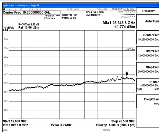
Band66-5MHz-16QAM-132322-1-0-Low-12000-26500--41.77-PASS
