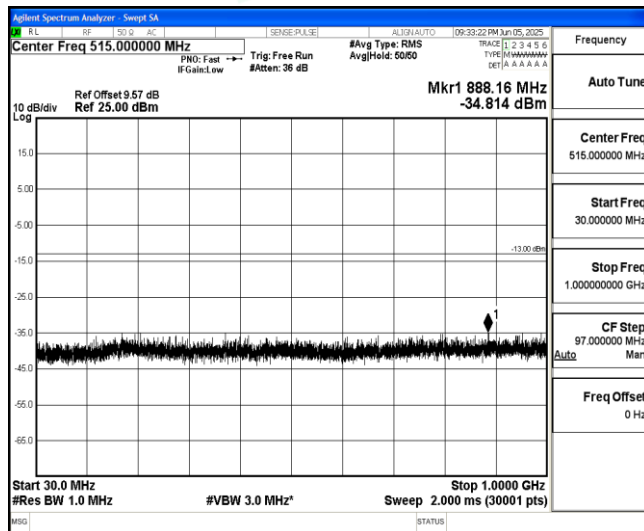
Band66-10MHz-QPSK-132022-1-0-Low-30-1000--34.81-PASS
