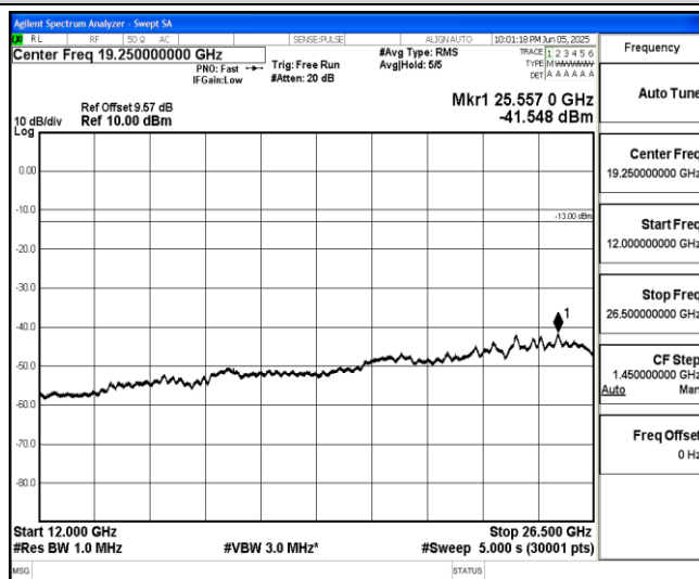
Band66-15MHz-16QAM-132322-1-0-Low-12000-26500--41.55-PASS
