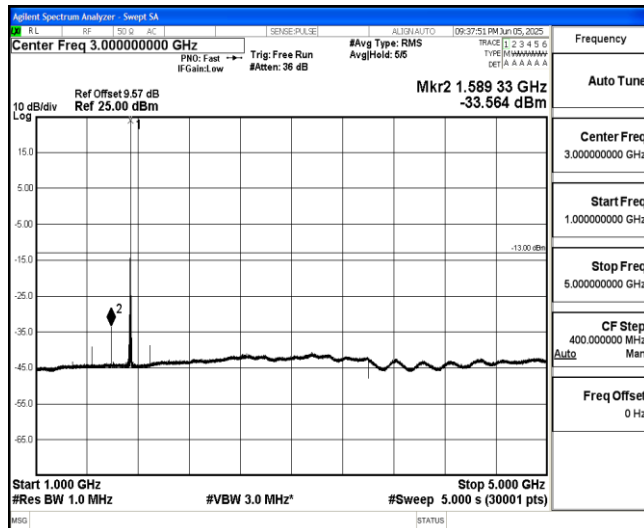
Band66-10MHz-QPSK-132322-1-0-Low-1000-5000--33.56-PASS
