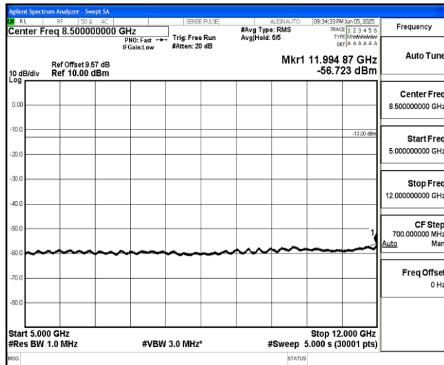
Band66-10MHz-QPSK-132022-1-0-Low-5000-12000--56.72-PASS
