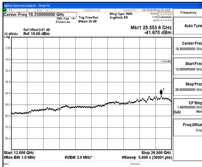
Band66-10MHz-QPSK-132022-1-0-Low-12000-26500--41.67-PASS
