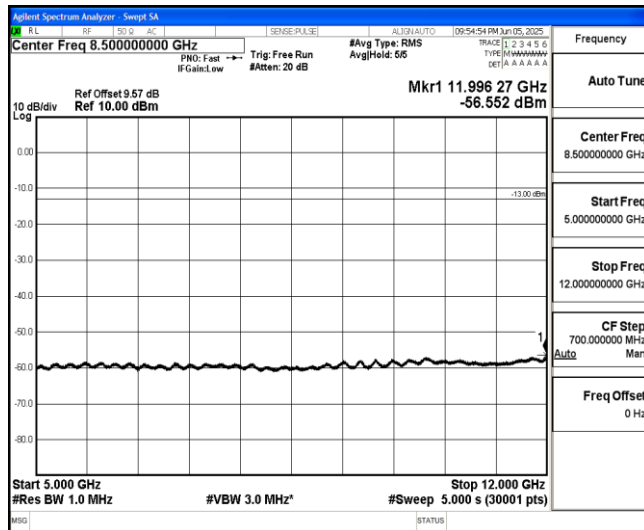
Band66-15MHz-QPSK-132047-1-0-Low-5000-12000--56.55-PASS
