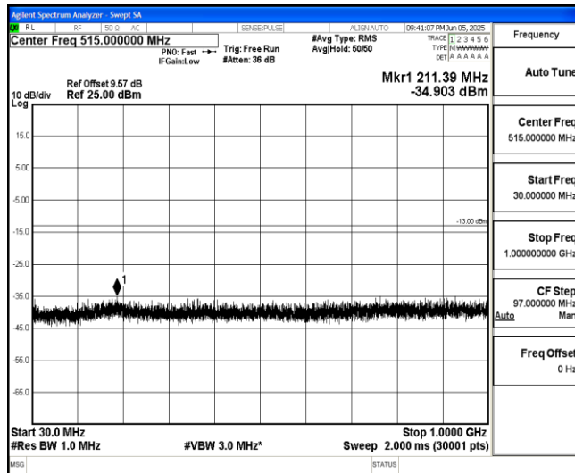
Band66-10MHz-QPSK-132622-1-0-High-30-1000--34.9-PASS
