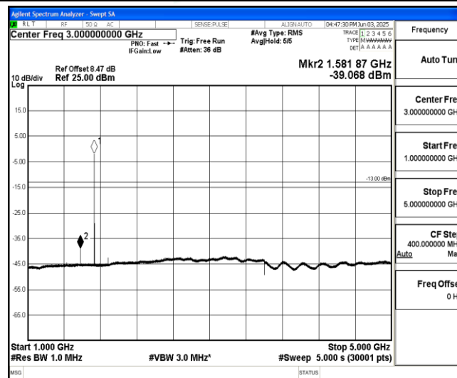
Band4-Stand-Alone-NaN-BPSK-20175-1@11-15kHz-1000-5000-1000~5000MHz@-39.07dBm--13-PASS
