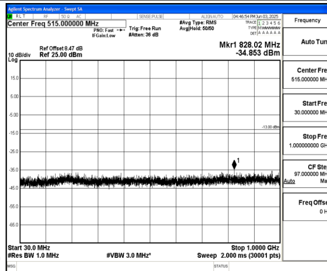
Band4-Stand-Alone-NaN-BPSK-20175-1@11-15kHz-30-1000-30~1000MHz@-34.85dBm--13-PASS
