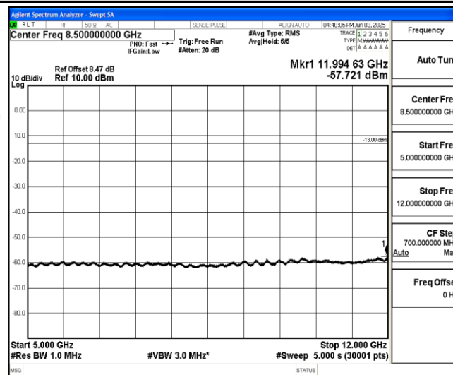
Band4-Stand-Alone-NaN-BPSK-20175-1@11-15kHz-5000-12000-5000~12000MHz@-57.72dBm--13-PAS
