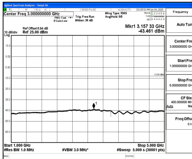
Band13-Stand-Alone-NaN-BPSK-23181-1@11-15kHz-1000-5000-1000~5000MHz@-43.46dBm--13-PASS
