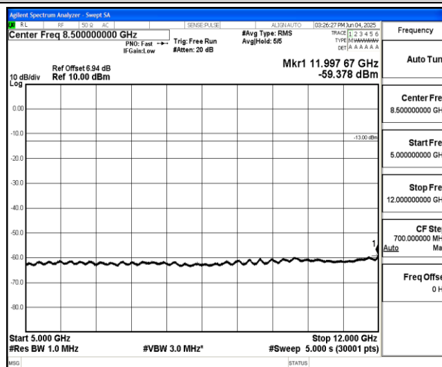
Band13-Stand-Alone-NaN-BPSK-23181-1@11-15kHz-5000-12000-5000~12000MHz@-59.38dBm--13-PASS
