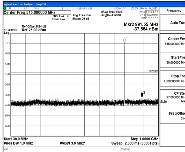
Band13-Stand-Alone-NaN-BPSK-23181-1@11-15kHz-30-1000-30~1000MHz@-37.55dBm--13-PASS
